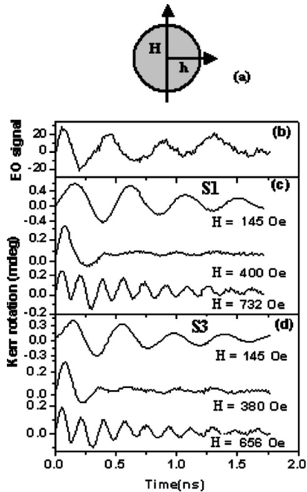
FIG. 1. (a). The experimental geometry is shown. The (b) pulsed field profile, and the measured time dependent Kerr rotations are shown for samples (c) S1 and (d) S3. The values of the static field H are shown within the figure.
