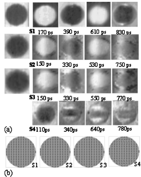
FIG. 4. (a) The time-resolved Kerr images obtained in the geometry of Fig. 1(a) are shown for S1, H=145 Oe; S2, H=145 Oe; S3, H=145 Oe; and S4, H=155 Oe. The delay times are shown under each image while intensity images are shown in the column at the left for S1–S3. (b) The simulated magnetic images before application of the pulsed field \mathbf{h} are shown.
