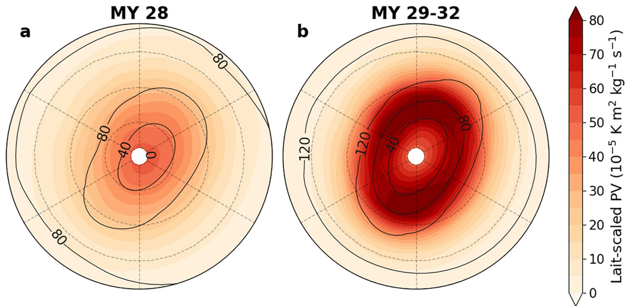
Figure 5. Mars' northern hemisphere polar vortex during a dust storm. Northern polar stereographic winter averages of Lait-scaled potential vorticity (shading) and zonal winds (contours) on the 350 K potential temperature surface. (a) The polar vortex during the Martian Year (MY) 28 global dust storm, and (b) the polar vortex averaged over MY 29–32, during which time there were no global dust storms. Data are extracted from the OpenMARS reanalysis data set and averaged over L_s = 255^\circ – 285^\circ . Panels are bounded at 50^\circ\text{N} and dashed lines of latitude are at intervals of 10^\circ\text{N} . Figure adapted from Ball et al. (2021).
