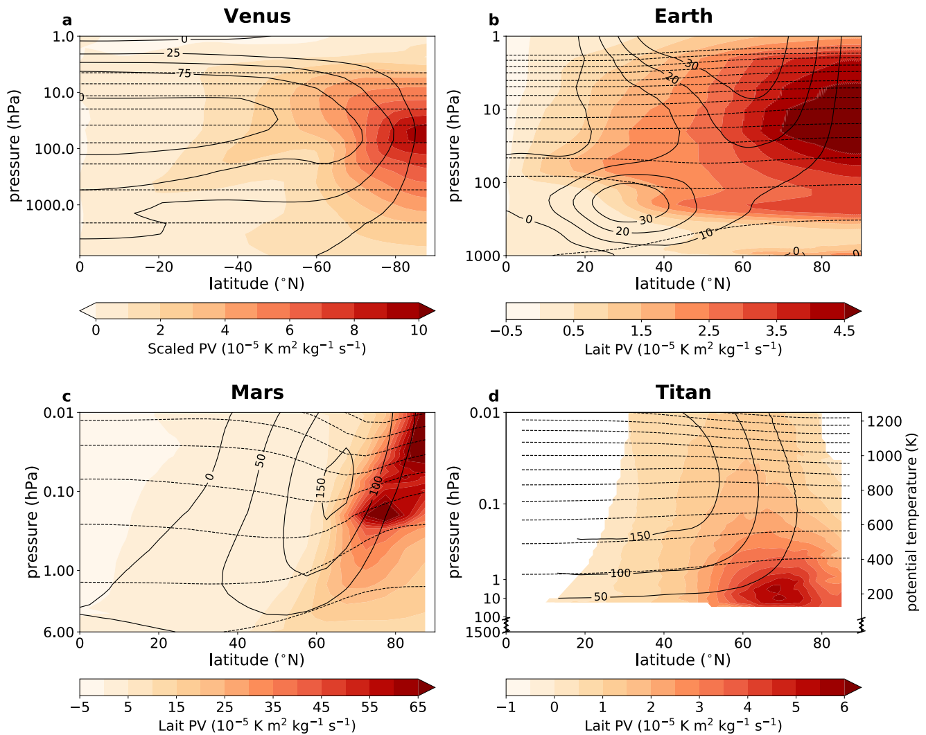
Figure 1. Winter zonal potential vorticity (PV) and zonal wind cross-sections as a function of altitude for Venus (a), Earth (b), Mars (c), and Titan (d). (a) Southern hemisphere monthly mean zonal-mean scaled potential vorticity (shading, scaling, and PV calculations according to Piccialli et al. (2012) and Garate-Lopez et al. (2016)), zonal wind (solid contours, units of \text{ms}^{-1} ), and potential temperature (dashed contours, corresponding to 300, 400, ... K). (b–d) Northern hemisphere monthly mean zonal-mean Lait-scaled potential vorticity (shading (Lait, 1994)), zonal wind (solid contours, units of \text{ms}^{-1} ), and potential temperature (dashed contours, corresponding to 200, 300 ... K). Data are taken from the following sources: (a) 30 Earth days (28 March–26 April 2008) of the AFES-Venus general circulation model with VALEDAS data assimilation, described in Sugimoto et al. (2019); (b) the ERA5 reanalysis data set, averaged over December–January–February for 1979–2019; (c) the OpenMARS reanalysis data set, averaged over Ls 255°–285° from MY 24–32; and (d) analysis of Cassini Composite InfraRed Spectrometer data from Sharkey et al. (2020b), averaged over Ls 325°–345° (September 2006–April 2008). The compressed axis represents Titan's troposphere. Note. Positive winds are defined as in the direction of the rotation of the planet, which for Venus is in the opposite sense to the other planets. Figure adapted from Ball et al. (2021), Mitchell and Ball (2021), Sharkey et al. (2020b), and Waugh et al. (2016).
