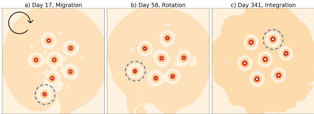
Figure 8. A simulation of Jupiter's vortex clusters, showing (a) an intruder migrating in, (b) rotation of that intruder around the main cluster, and (c) integration of the intruder into the main cluster. The vortex of interest has a dashed circle around it. The direction of rotation of the configuration is given in the left panel. Figure adapted from Li et al. (2020).
