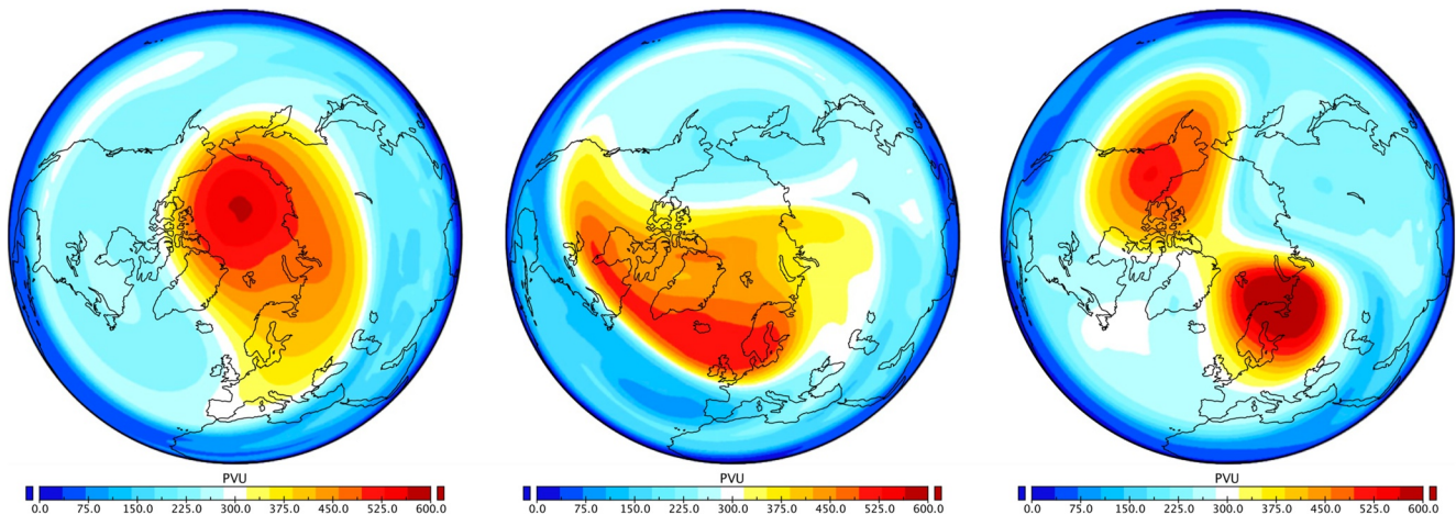
Figure 2. The different states of Earth's northern hemisphere stratospheric polar vortex. Northern polar stereographic plots of snapshots of Ertel (theta-normalized) potential vorticity in the mid stratosphere (10 hPa, ~30 km) during (left) a stable period, (middle) a vortex displaced period, and (right) vortex split period. Units are potential vorticity units (Kang & Tziperman, 2017).
