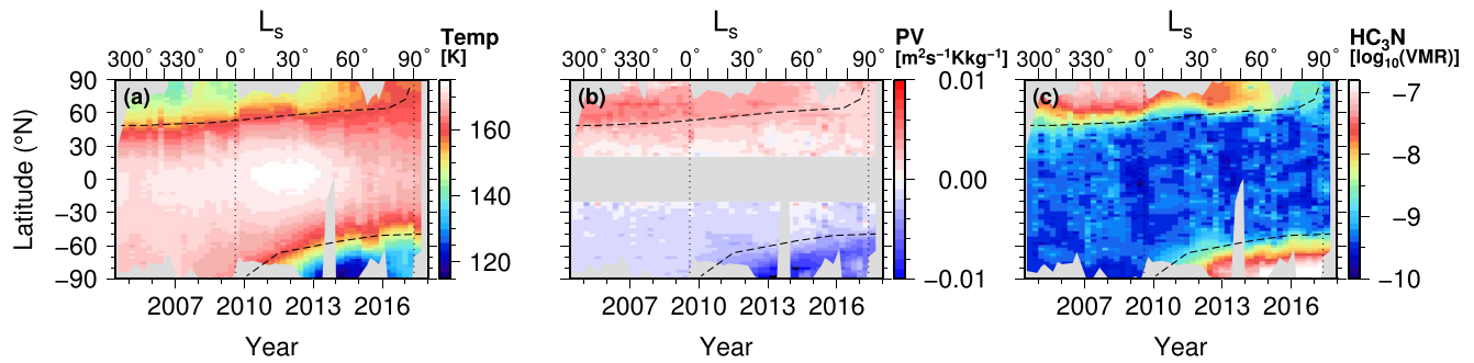
Figure 6. Titan's polar vortex structure and evolution observed by Cassini Composite InfraRed Spectrometer. (a) Temperature at 1 hPa (Sharkey et al., 2020b) showing cold mid-stratosphere temperatures within the polar vortices. (b) Potential vorticity (PV) at 0.1 hPa (Sharkey et al., 2020b) showing strong PV gradients near the vortex edge and an annular PV structure, with peak PV at \sim 65^\circ . (c) \text{HC}_3\text{N} volume mixing ratio (Teanyby et al., 2019) showing confinement of a short lifetime ( \ll Titan year) gas within the polar vortex. Dotted vertical lines are the 2009 northern spring equinox and 2017 northern summer solstice. Dashed regions indicate approximate edge of northern and southern vortices.
