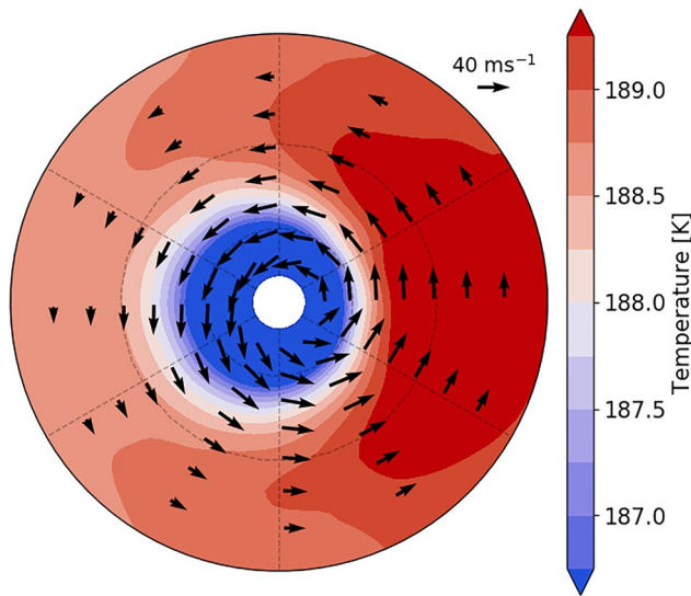
Figure 9. Northern polar stereographic plot of temperature (shading) and zonal wind (vectors) on the 5 hPa level from model simulations of TRAPPIST-1e. Dashed lines correspond to 30°, 60°N and the figure is bounded at the equator. Data is taken from the HAB1 Unified Model experiment from Fauchez et al. (2020).
