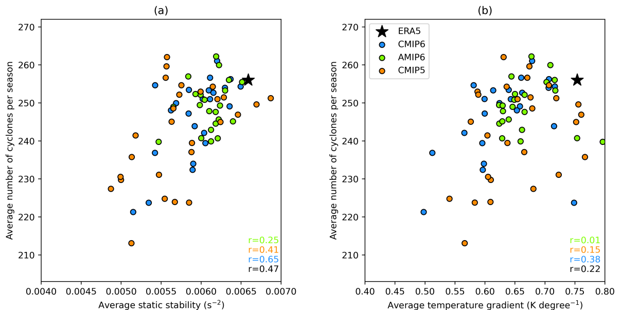
FIG. 8. Scatter plots of (a) lower tropospheric static stability ( s^{-2} ) and (b) 850 hPa potential temperature gradient ( K \text{ degree}^{-1} ) against seasonal cyclogenesis rate. Large-scale fields are averages from 40°S-70°S for CMIP6 (blue), CMIP5 (orange), AMIP6 (green) and ERA5 (black star) in JJA.
