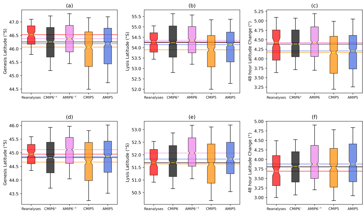
FIG. 3. Boxplots of annual mean cyclogenesis latitude (a,d), cyclolysis latitude (b,e), and cyclone 48-hour latitude change (c,f) for Reanalyses, CMIP6, AMIP6, CMIP5, and AMIP5 in DJF (a–c) and JJA (d–f). Horizontal coloured lines indicate the median value for each model distribution. Boxes extend to the 25th and 75th percentile respectively with yellow lines indicating the distribution median. Notches around the median show the uncertainty estimate based on 10,000 random samples and whiskers extend to the 10th and 90th percentiles. In the labels ★ indicates where the model group is significantly different from the reanalyses, † indicates where AMIP6 and CMIP6 are significantly different, and λ indicates where CMIP6 and CMIP5 are significantly different. Significance tests performed using a Mood’s Median test and quoted at the 5% level.
