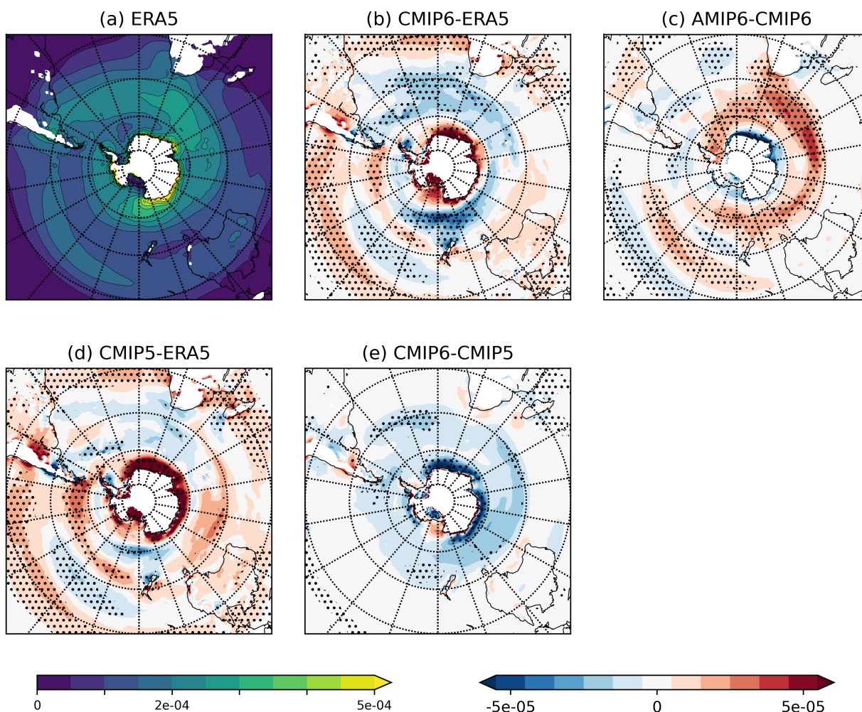
FIG. 7. Eady Growth Rate for JJA for (a) ERA5, (b) CMIP6-ERA5, (c) AMIP6-CMIP6, (d) CMIP5-ERA5, and (e) CMIP6-CMIP5. Units are s^{-1} . Stippling indicates where there is 80% model agreement on the sign of the change.
