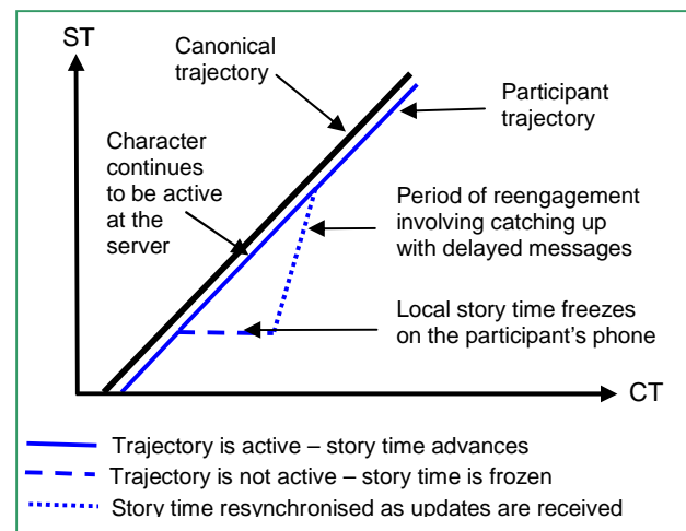
Figure 3: Disengagement and reengagement in DoF
