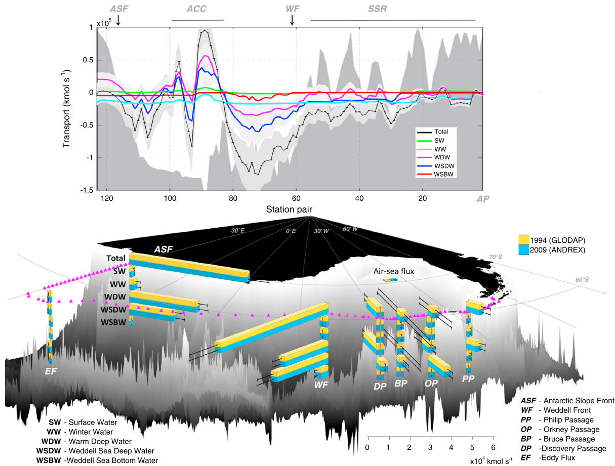
Figure 3. (a) Cumulative contemporary carbon transports (with shaded uncertainties) for a number of water mass classifications. The positive (negative) values indicate the transports into (out of) the Weddell Gyre box. Abbreviations: WF = Weddell Front, ACC = Antarctic Circumpolar Current, ASF = Antarctic Slope Front, AP = Antarctic Peninsula, and SSR = South Scotia Ridge. (b) Air-sea carbon flux and total carbon transports for ANDREX and GLODAP data inputs for the full water column and separated into constituent water masses for main import/export regions of the gyre, namely, the deep passages of the South Scotia Ridge and the Weddell Front and Antarctic Slope Front (southward view). The error bars indicate the transport uncertainties (standard deviation) to represent short-term variability of flows. Bathymetry from the ETOPO 2 2 min global bathymetry database.
