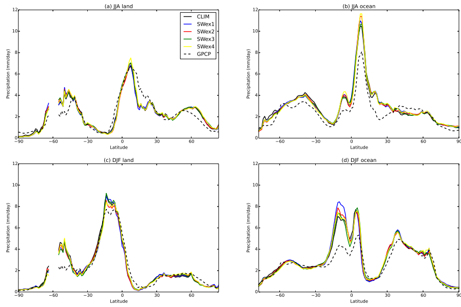
Fig. 5 Zonal mean precipitation in CLIM and SWex compared to GPCP ( \text{mm day}^{-1} ) in JJA (a,b) and DJF (c,d) over land (a,c) and ocean (b,d) points.
