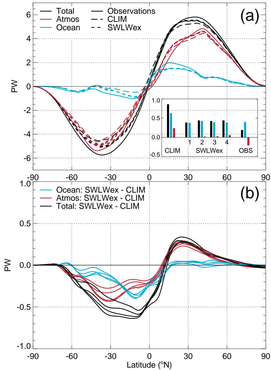
Fig. 10 Annual mean meridional energy transport: (a) total (black), ocean (blue) and atmospheric (red) components of the energy transport (PW, northward positive) in observations (solid), CLIM (long dashes) and the four SWLWex experiments (dashed), (b) the difference in the total/ocean/atmosphere between CLIM and the SWLWex experiments. The bar plot embedded within (a) shows the cross-equatorial energy transport (PW, northward positive) with colours as for the other plots.
