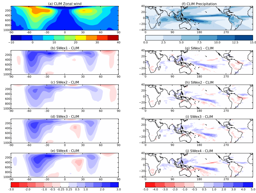
Fig. 3 Zonal mean eastward wind (a, \text{m s}^{-1} ) and precipitation (f, \text{mm day}^{-1} ) in the CLIM simulation and the difference in eastward wind (b-e) and precipitation (g-j) between the four SWex experiments and the CLIM simulation.
