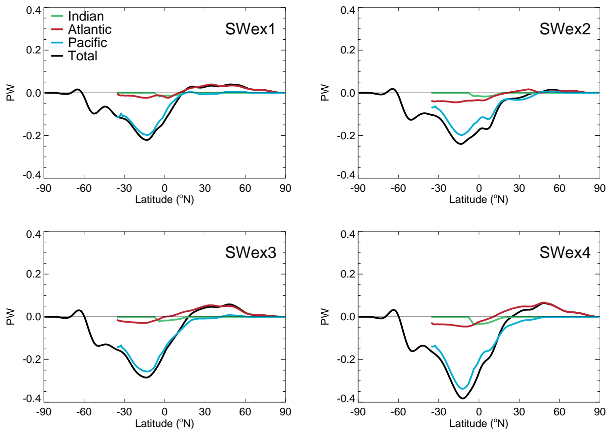
Fig. 7 Change in annual mean meridional energy transport (PW, northward positive) from the CLIM simulation for total ocean energy transport (black), Pacific (blue), Atlantic (red) and Indian (green) Oceans. In the model, Indian Ocean fluxes are only output to 5°S. The southern Indian Ocean fluxes are included in the Pacific transport term, though are small relative to the total energy transport in the Pacific basin.
