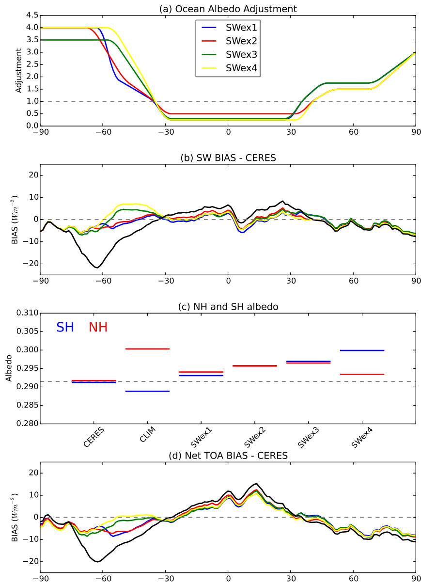
Fig. 2 Shortwave forcing applied and response obtained in the experiments: (a) the zonally uniform adjustment (multiplication of existing albedo, up to a maximum albedo of 1) to the ocean albedo applied to the model, (b) the zonal mean bias ( \text{W m}^{-2} , upwards as positive) in the top of atmosphere net shortwave radiation in the CLIM (black) simulation and the four SWex experiments as a result of the forcing applied in (a) compared to CERES, (c) the mean albedo in the Northern and Southern Hemisphere (NH/SH) in CERES, CLIM and SWex, (d) the zonal mean bias ( \text{W m}^{-2} , upwards as positive) in the top of atmosphere net radiation (shortwave and longwave) in CLIM and SWex compared to CERES.
