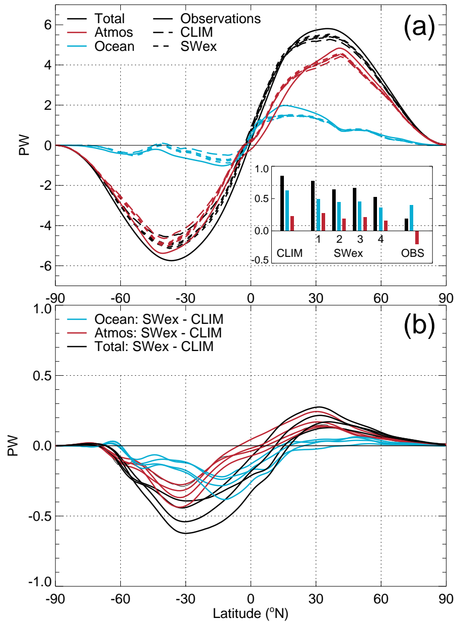
Fig. 6 Annual mean meridional energy transport: (a) total (black), ocean (blue) and atmospheric (red) components of the energy transport (PW, northward positive) in observations (solid), CLIM (long dashes) and the four SWex experiments (dashed), (b) the difference in the total/ocean/atmosphere between CLIM and the SWex experiments. The bar plot embedded within (a) shows the cross-equatorial energy transport (PW, northward positive) with colours as for the other plots.
