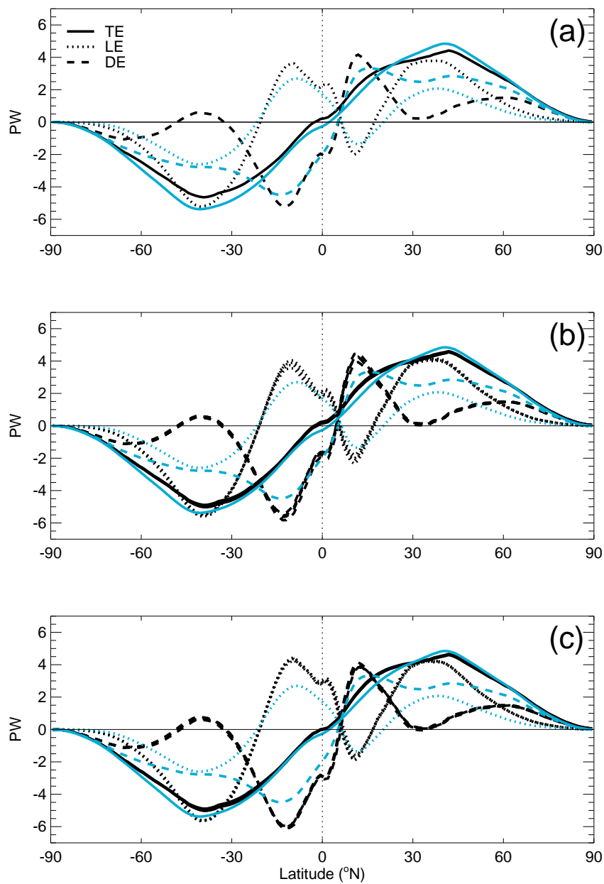
Fig. 11 Annual mean meridional energy transport (PW) in the atmosphere in HadGEM2-ES (black) and ERAI (blue) for (a) the CLIM simulation, (b) the SWex experiments and (c) the LWSWex experiments. The total AET (TE, solid lines), latent energy (LE, dotted lines) and dry energy (DE, dashed lines) transport terms are shown.
