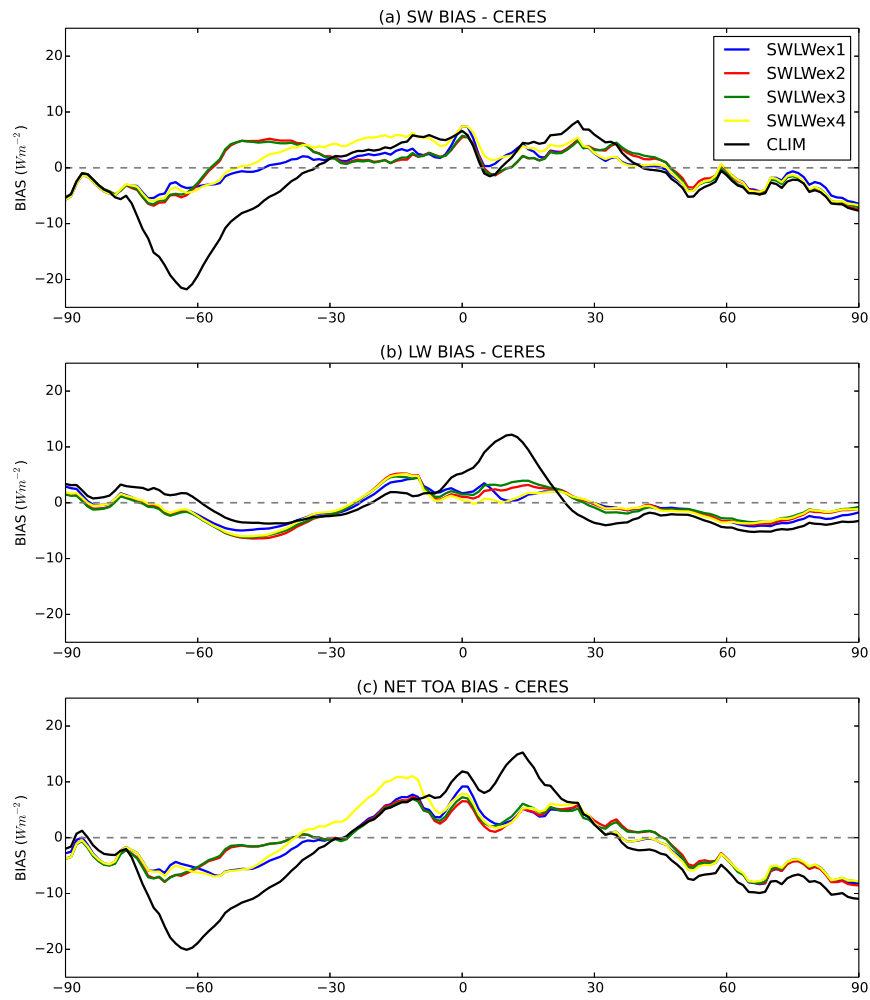
Fig. 9 Top of atmosphere net shortwave (a), longwave (b) and total net radiation (c, \text{W m}^{-2} , upwards as positive) zonal mean biases in CLIM and the SWLWex experiments compared to CERES.
