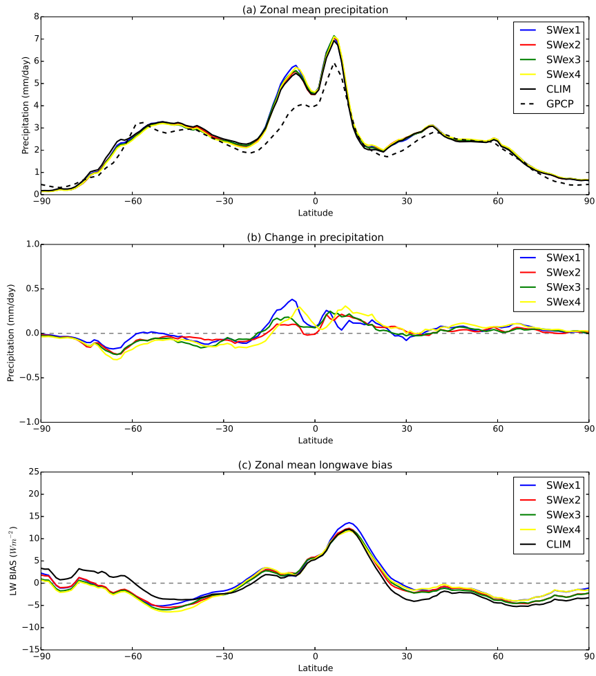
Fig. 4 Zonal mean (a) precipitation in CLIM and SWex compared to GPCP ( mm\ day^{-1} ), (b) change in precipitation from CLIM to SWex and (c) TOA outgoing longwave radiation bias in CLIM and SWex compared to CERES ( W\ m^{-2} , upwards as positive).
