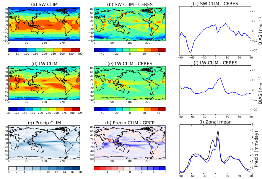
Fig. 1 Top of atmosphere net shortwave (a-c) and longwave (d-f) radiation ( \text{W m}^{-2} ) and precipitation (g-i, \text{mm day}^{-1} ) showing the model climatology (CLIM, a,d,g) with the model bias (b,e,h) and the zonal mean bias compared against CERES (c,f, upwards as positive) and zonal mean precipitation compared against GPCP (i, model in black and GPCP in blue).
