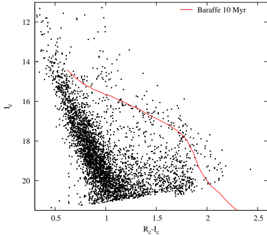
Figure 2. A colour-magnitude diagram for unflagged objects with uncertainties < 0.1 mag in I_C and R_C - I_C seen in CCD 4 (see Fig. 1). The solid line shows a theoretical 10 Myr PMS (from Baraffe et al. 2002) at an intrinsic distance modulus of 10.13, and with a reddening/extinction corresponding to E(R_C - I_C) = 0.14 (see Section 5).
