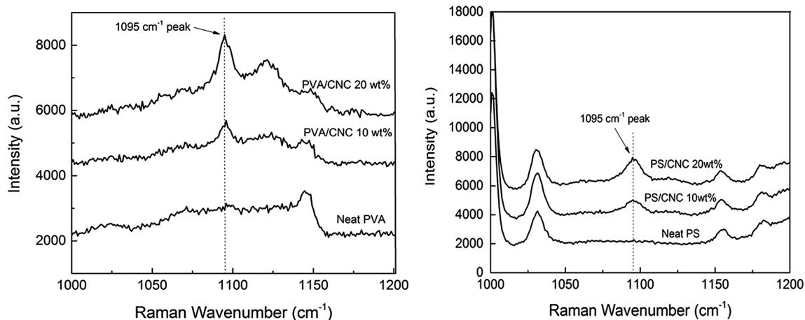
Fig. 3 Typical Raman spectra of (left) PVA/CNC (right) PS/CNC
