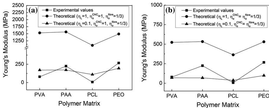
Fig. 7 A comparison between experimental and theoretical values of Young's moduli electrospun polymer/CNC fibre mats with different polymeric matrices; a only CNCs are highly oriented ( \eta_o = 1/3 ),
