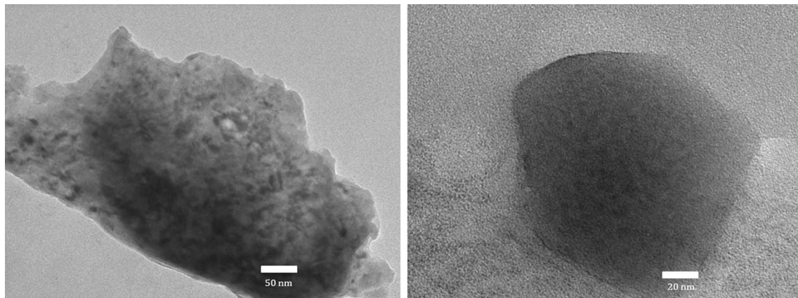
Fig. 5 Typical TEM images showing the orientation of CNCs in PS/CNC 10 % fibres. Left image showing CNCs present ( darker regions ) along the axis of the electrospun fibre, in the plane of the page; right
