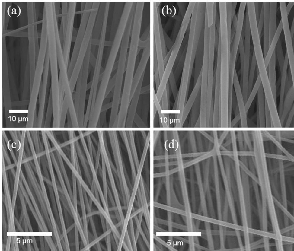
Fig. 1 SEM images of oriented fibres of PS/CNC a 10 %, b 20 %; and PVA/CNC c 10 %, d 20 %
