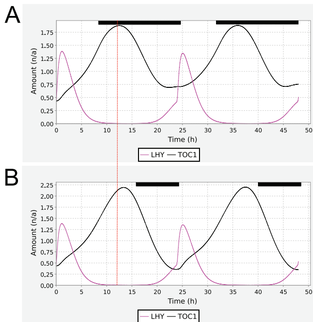
Figure 2. Shift in TOC1 peaks in Locke 3 loop model. Reproduction of Figure 3 from Locke et al. (2006), using the 3-loop circadian clock model BIOMD0000000089 enhanced with the SBML step function. The figure shows simulations of TOC1 mRNA (black) and LHY mRNA (magenta) under photoperiods of (A) LD8:16 and (B) LD16:8. The vertical dotted line highlights the shift in the peak phase of TOC1 mRNA levels from LD8:16 to LD16:8, whereas the peak phase of LHY mRNA is not shifted. Dark periods are indicated using the black bars above the traces. The parameterization of the step function for panel A was \Theta_0 = 0 , \Theta_1 = 1 , T_c = 24 h, T_p = 8 h, T = 0.1 h, and \phi = 0 h (A); for panel B, as for panel A but T_p = 16 h.
