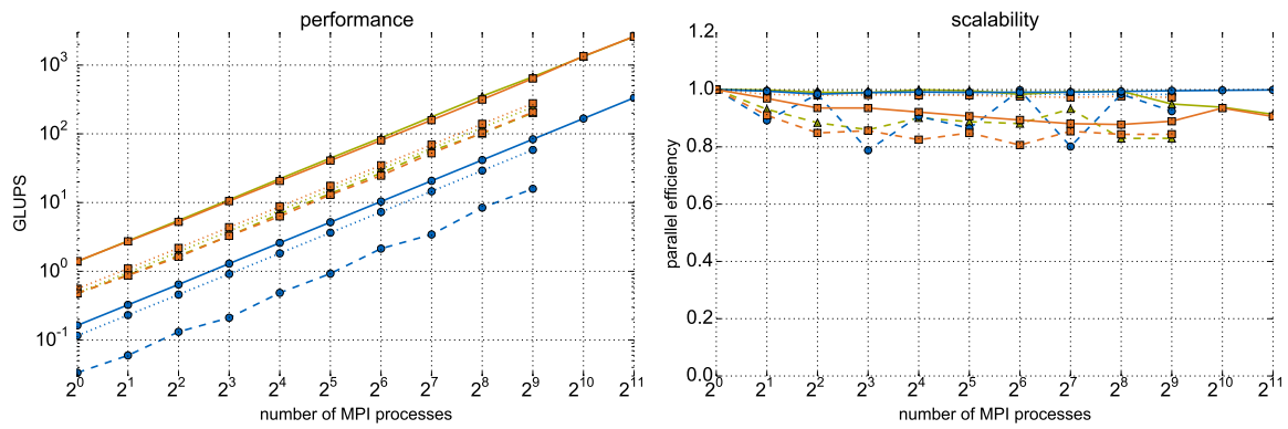
(a) Parallelization in y -direction
