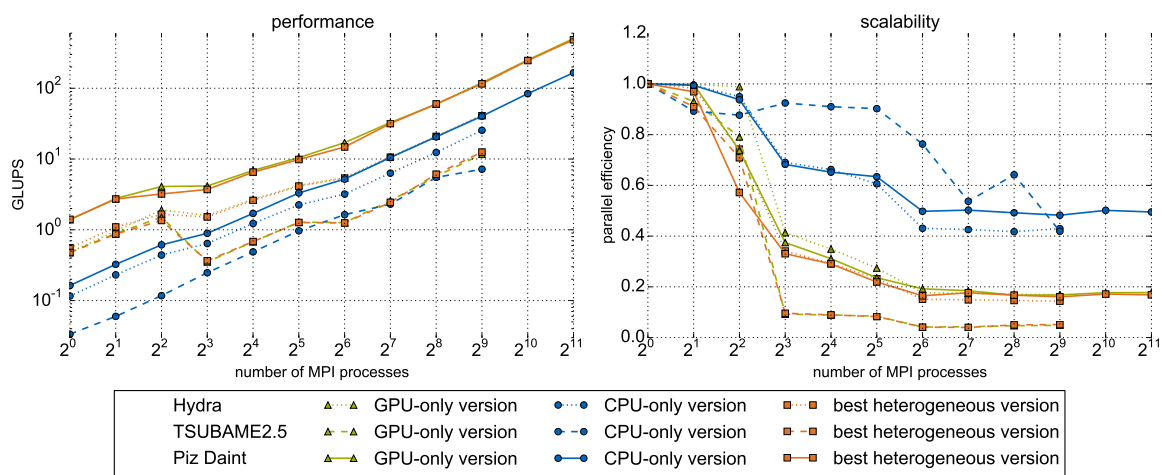
(b) Parallelization in x/y/z -direction
