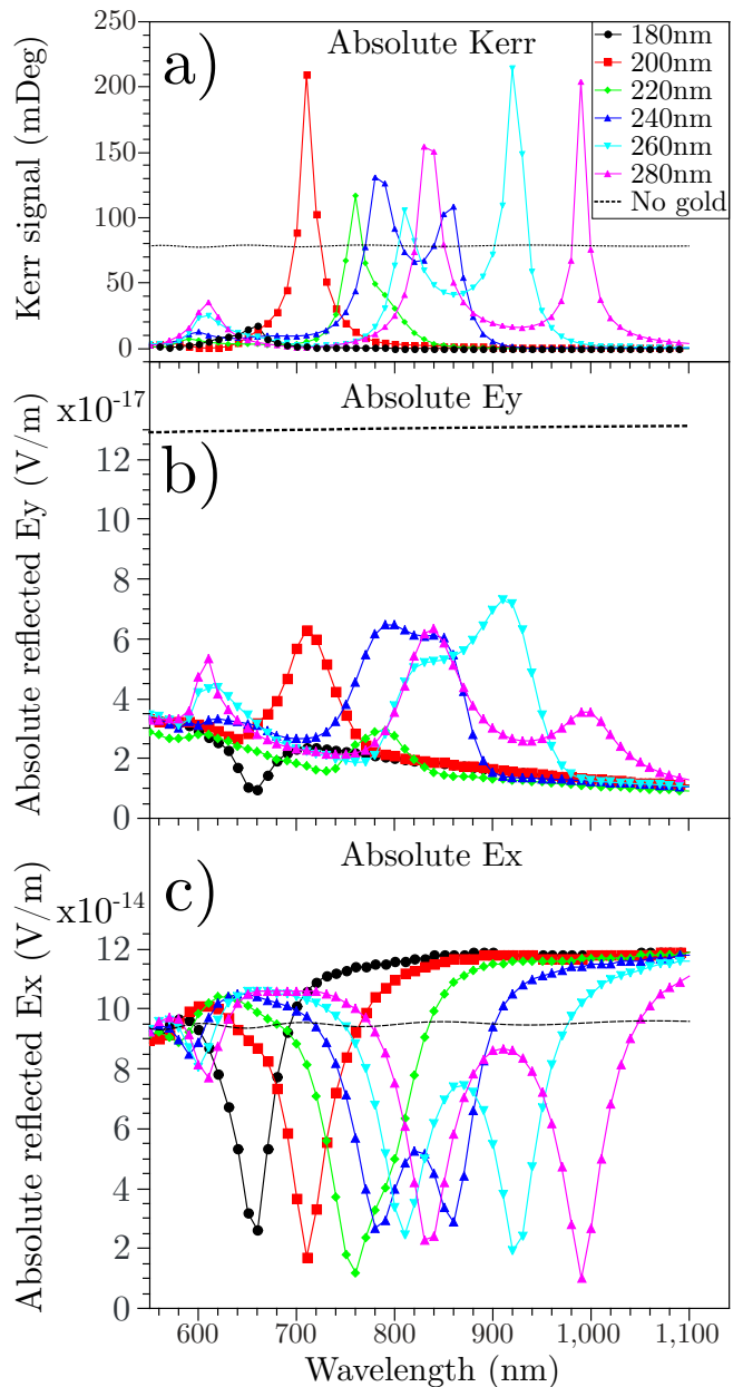
FIG. 2. a) Absolute Kerr signal (the rotation and ellipticity summed in quadrature) spectra for a series of cross structures of different arm length. The resonant wavelength varies linearly with arm length through the range studied. The maximum MOKE signal exceeds that of the bare magnetic film in all cases, and is greatest for the 200 nm arm length. The stated arm lengths are for the underside of the cross structure that faces the magnetic material. b) The spectra of the absolute relative y component of the electric field for a range of cross lengths, as well as the bare magnetic film (dashed line). c) The spectra of the absolute relative x component of the electric field.
