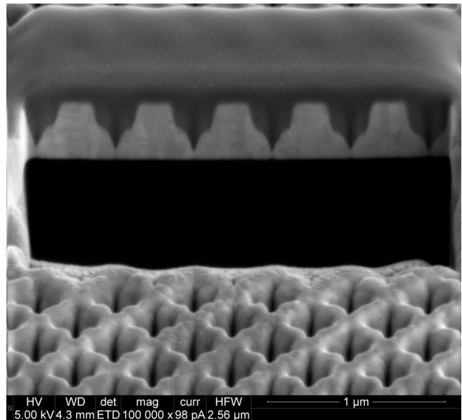
FIG. 6. SEM micrograph of a cross section taken through the center of several partially milled cross cavities. The central region of each cavity is milled to a greater depth due to the overlap of milling in this region.
