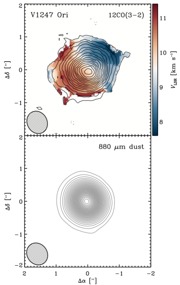
Fig. 9. (top): Synthesized 4'' \times 4'' map of the CO J=3-2 integrated intensity from the disc around V1247 Ori (contours increase at 150 \text{ mJy km s}^{-1} \text{ beam}^{-1} intervals) overlaid on the intensity-weighted velocities (colour scale; to show sense of rotation). (bottom) The synthesized 4'' \times 4'' 880 \mu\text{m} continuum map. Contours increase at 4.25 \text{ mJy beam}^{-1} intervals. The bottom left corners of each map show the synthesized beam dimensions.
