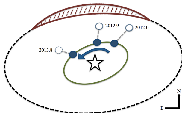
Fig. 4. A simple sketch of the scenario we propose to explain the non-physically fast change in position angle that is retrieved with simple companion-only fits. Our simulations show that for a close-in companion (solid circles), the best-fit angular separation derived with SAM interferometry (hollow circle) can be over-estimated, if the companion is roughly aligned with asymmetric disc emission (red dashed region). The strength of this over-estimation is related to several parameters, in particular the disc radius and the difference between the companion candidate position angle and disc position angle. An unfavourable alignment between the companion and the peak of the disc rim emission or a too-small separation result in no overestimation effect in the derived separation and the companion candidate remains undetected. This seems to be the case at the 2013.8 epoch, where the absence of extended disc emission along the same position angle causes no overestimation. Here, the orbit of the companion candidate and the arc of the disc is misaligned to better represent the position angles found within the previous disc observations of the outer disc ( \sim 120^\circ , green ring) and the position angle of the disc rim from the L'-band observations presented here ( \sim 95^\circ , black ring).
