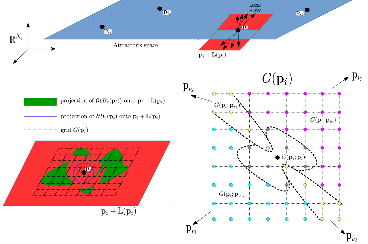
Figure 6: Top: in blue, the low-dimensional space containing the attractors; in red, a sketch of the LSS of attractor \mathbf{p}_i . Bottom left: representation of the local input response set \mathcal{G}(B_r(\mathbf{p}_i)) and the grid G(\mathbf{p}_i) in the LSS of \mathbf{p}_i . Bottom right: illustration of the partition of a two-dimensional grid G(\mathbf{p}_i) . Every colour represents a subset (25). Dashed black lines track the boundary of the basins corresponding to those attractors reachable from \mathbf{p}_i through excitable connections, which can be enabled by inputs allowing to explore the hypercube centred on \mathbf{p}_i .
