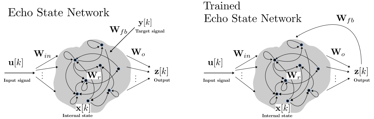
Figure 1: Left: Illustration of an ESN in the open-loop phase (4). Training is supervised by means of the target signal to learn \mathbf{y} . Right: Illustration of an ESN (5) after the optimisation of the read-out matrix. Feeding back the output signal into the reservoir (closed loop system) allows the system to self-sustain dynamics, which is also driven by the input signal.
