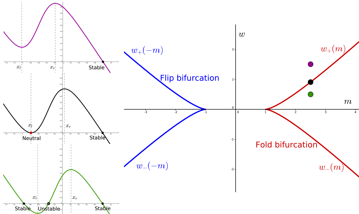
Figure 12: Left: three different folding configuration of the function Q(x) in (32) with m = 2.5 ; purple w = 1.5 , black w \approx 0.9 , green w = 0.5 . Right: bifurcation diagram of fixed points in one-dimensional ESN.
