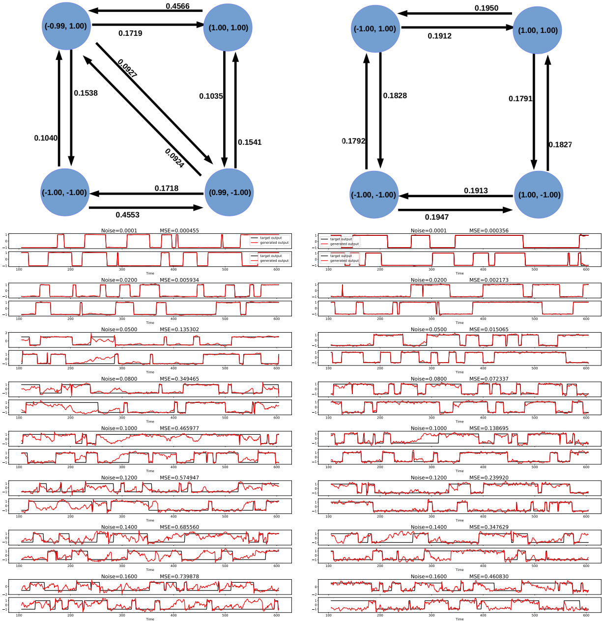
Figure 11: Left: results corresponding to a trained ESN giving rise to an ENA with undesired connections and unbalanced outgoing weights (28). Right: results obtained with a trained ESN giving rise to an ENA with balanced outgoing weights for all excitable connections. From top to bottom, in both columns, ESN outputs and related MSEs obtained with increasing noise standard deviation: 10^{-4} , 2 \cdot 10^{-2} , 5 \cdot 10^{-2} , 8 \cdot 10^{-2} , 10^{-1} , 1.2 \cdot 10^{-1} , 1.4 \cdot 10^{-1} , and 1.6 \cdot 10^{-1} .
