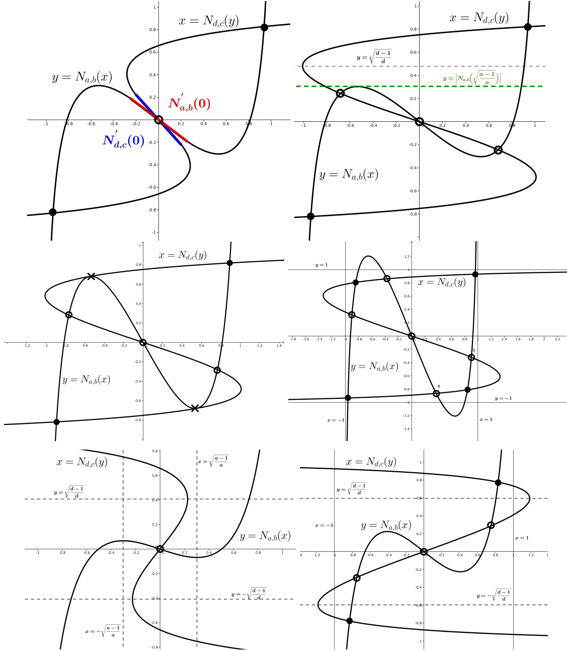
Figure 13: In all panels, filled points denote stable attractors, while circles denote saddles or repellers. Top left: geometric representation of the sufficient condition (37); nullcline slopes on the origin are highlighted with different colours. Top right: illustration of the condition (38); the black dashed line acts as an upper bound ensuring that the maximum height of the peak of the x -nullcline (represented by the green dashed line) does not cross further the y -nullcline. Centre left: special case of 7 fixed points. Crosses indicate neutral fixed points where fold bifurcations take place. Centre right: an example of nullclines configuration holding the condition (41) in the case of bc > 0 . Both curves come out of the invariant square [-1, 1]^2 with their humps, that guarantees 9 intersections, i.e., 9 fixed points. Bottom left: depiction of the sufficient condition (39); the origin is the only fixed point and it is unstable. Bottom right: illustration of the sufficient condition (40).
