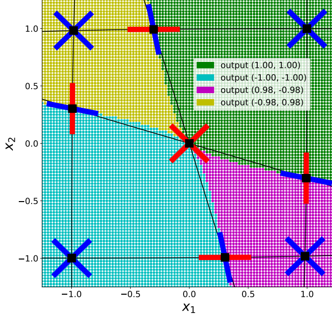
Figure 3: Basins of attraction, nullclines, fixed points and corresponding eigenvectors of the two-dimensional system defined by (16), with b = 0.2 . Black curves represent the nullclines (see Appendix B) whose reciprocal intersections determine fixed points (square black points). Red segments indicate eigenvectors associated with real eigenvalues larger than one. Blue line segments represent eigenvectors of real eigenvalues in (0, 1) . Particularly important are blue lines of saddles, which represent local linear approximations of the boundary of the basins of attraction. The whole phase space is divided in four basins of attraction associated to the four stable points. Boundaries between these basins coincide with the four heteroclinic trajectories connecting the origin with the saddles. The legend shows output values produced at every attractor, which, in this specific example, correspond with the internal state, i.e., the phase space coordinates of the attractors. Points on the plane have been coloured according with the attractor on which they converged to after 100 steps.
