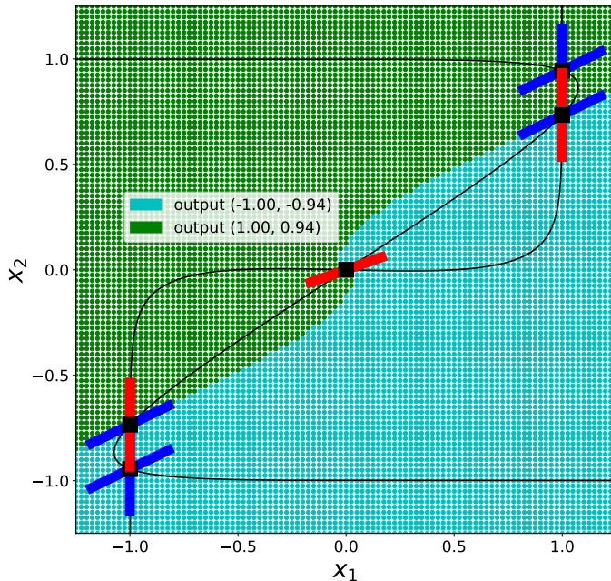
Figure 4: Basins of attraction, nullclines, fixed points and eigenvectors of the two-dimensional autonomous system having (18) as reservoir matrix, with s = 2 . Black curves represent the nullclines (see Appendix B) whose reciprocal intersections determine fixed points (square black points). Red segments indicate real eigenvectors associated with real eigenvalues larger than one. Blue line segments represent real eigenvectors of real eigenvalues in (0, 1) . The origin has complex conjugated eigenvalues lying outside the unit circle and a pair of eigenvectors; in the figure, only the real-valued one is depicted. Points of the plane have been coloured according with the attractor on which they converged after 100 steps.
