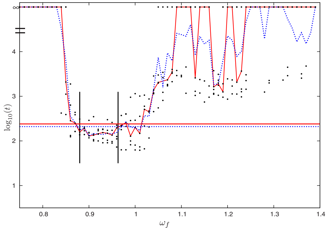
FIG. 8. (Color online) Extra current forcing: termination time for the amplitude A=0.3 . The black dots represent termination times for individual simulations. The red solid line goes through the median values of the termination times at a fixed frequency and the blue dashed line through the geometric mean values. The horizontal straight lines show the median (red solid line) and geometric mean (blue dashed line) termination times for the feedback experiments. The vertical brackets designate the window of resonant frequencies.
