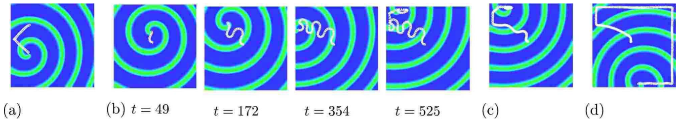
FIG. 12. (Color online) Two-dimensional phenomena. (a) “Resonant reflection:” Extra current forcing with constant frequency \omega_f=1.1855 and amplitude A=0.01 . (b)–(d) “Snake instability:” Extra current forcing with feedback controlled frequency applied with amplitudes A=0.01 (b), A=0.004 (c), and A=0.001 (d). Model parameters a=1.1 , b=0.19 , \epsilon=0.02 , L=60 , \Delta x=0.4 , and \Delta t=0.01 , with nine-point approximation of the Laplacian. The recording point in (b)–(d) was located in the bottom left corner.
