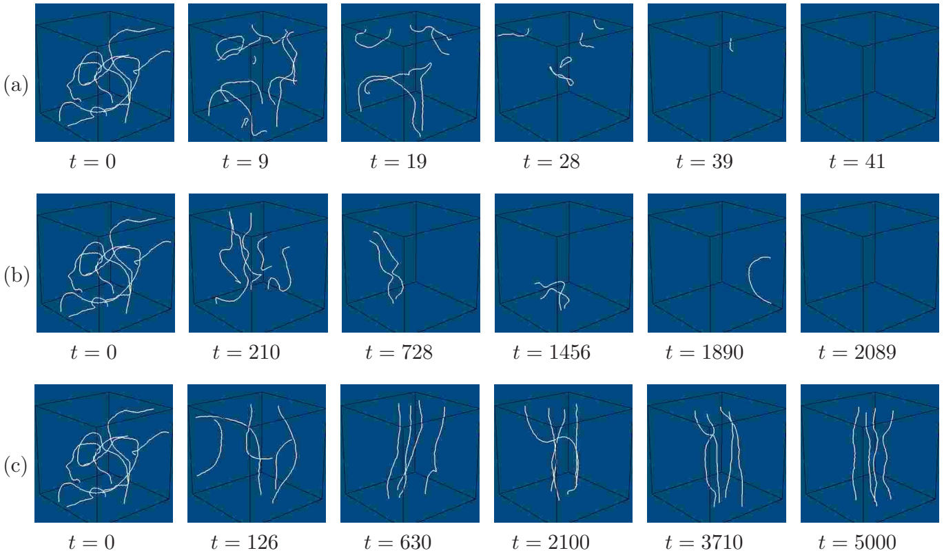
FIG. 4. (Color online) Examples of successful and unsuccessful elimination of turbulence. Evolution of the turbulence under modulation of medium excitability with (a) \omega_f=0.8 , (b) \omega_f=1.22 , (c) \omega_f=1.13 at fixed amplitude A=0.03 .
