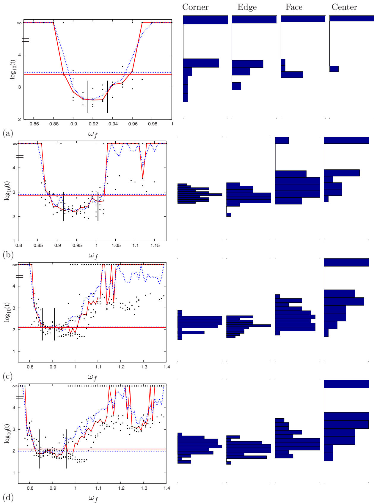
FIG. 9. (Color online) Extra current forcing: termination times for the amplitudes (a) A=0.1 , (b) A=0.2 , (c) A=0.4 , (d) A=0.5 . The left panels are as in Fig. 8. The histograms on the right are distribution of termination times for feedback controlled experiments, at different locations for the recording point (they are rotated 90° clockwise and flipped in the vertical direction, to bring their abscissa axes in line with the ordinata axes of the graphs on the left).
