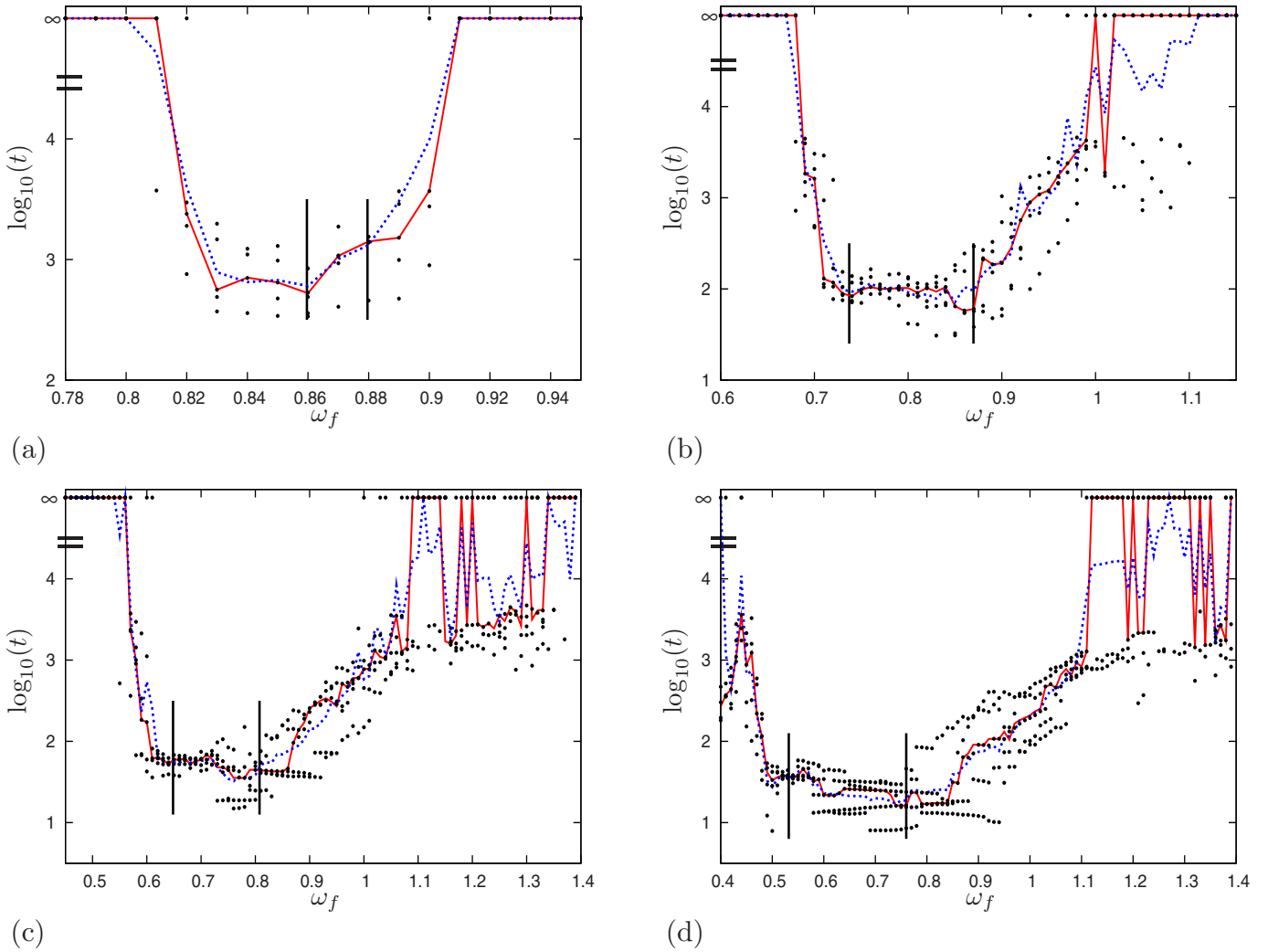
FIG. 5. (Color online) Modulation of medium’s excitability: termination times at different amplitudes (a) A=0.01 , (b) A=0.02 , (c) A=0.03 , and (d) A=0.05 . Black dots: termination times for individual simulations. Red solid line: median values of the termination times at every fixed frequency. Blue dashed line: same, geometric mean values. For averaging and visualization purposes, we assign value t=10^5 to the failures. Black vertical brackets: the windows of resonant frequencies for each amplitude.
