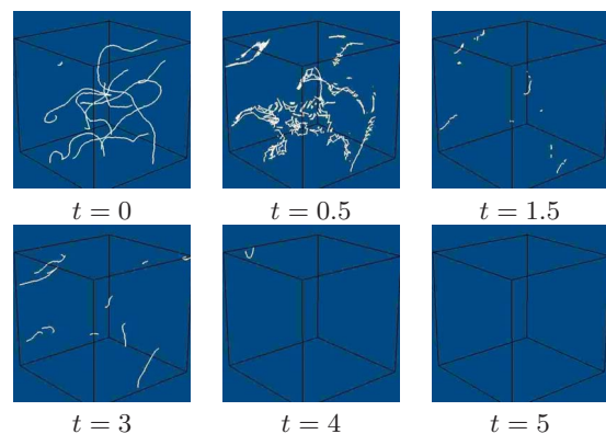
FIG. 7. (Color online) Single pulse: termination of the turbulence at forcing amplitude A=4.3 .
