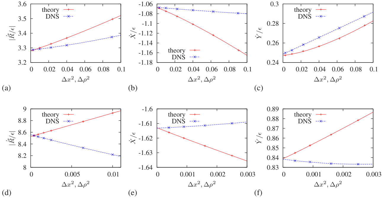
FIG. 3. (Color online) Numerical convergence of drift forces. Top row: FHN system. Bottom row: Barkley system. First column: resonant drift. Second and third columns: x and y components of the electrophoretic drift. The forces were measured for (a) \epsilon=10^{-3} , (b,c) \epsilon=10^{-2} , (d) \epsilon=5 \cdot 10^{-3} , (e,f) \epsilon=10^{-2} .
