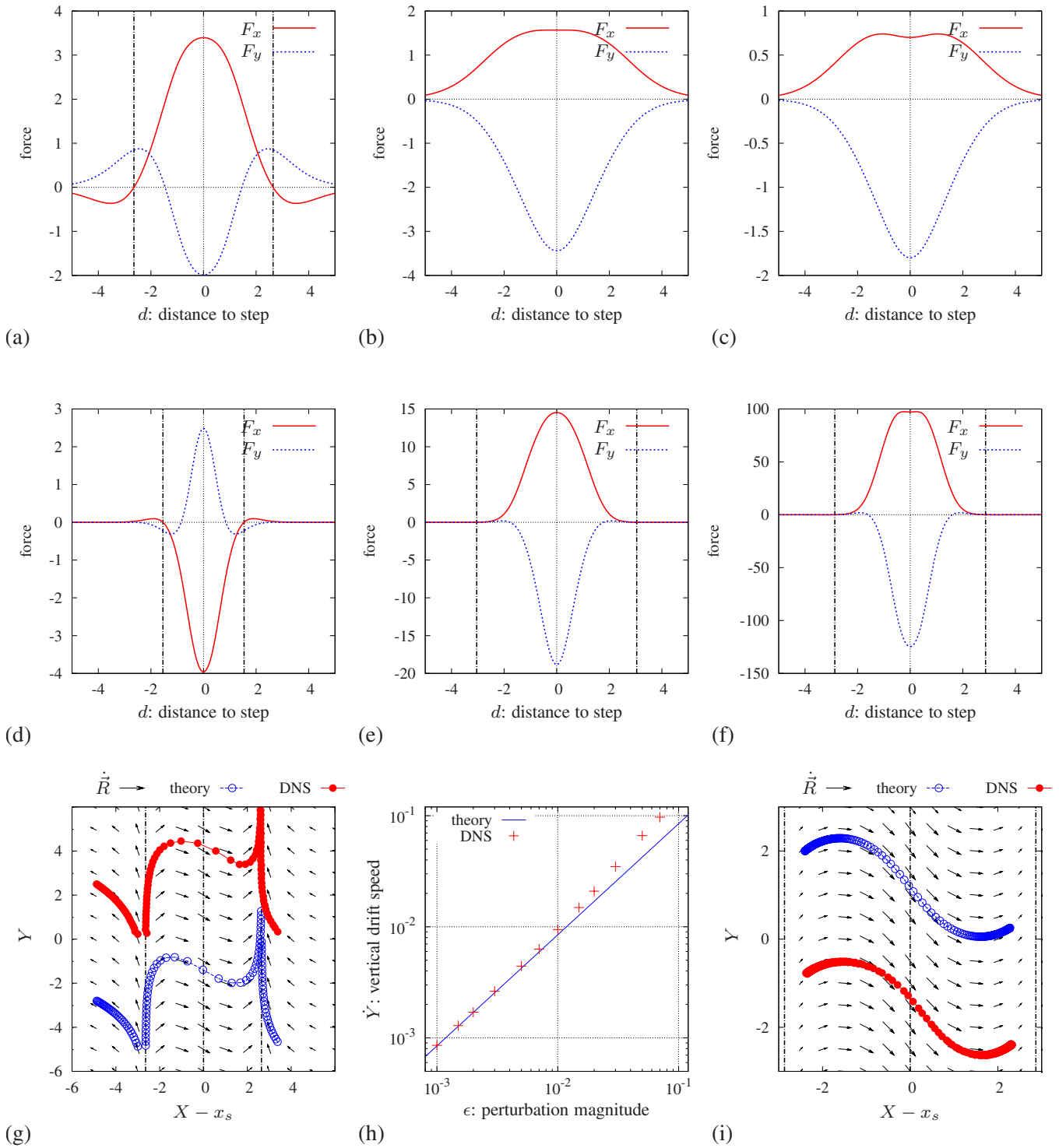
FIG. 4. (Color online) Drift in stepwise inhomogeneity Eqs. (45) and (47). First row: theoretical predictions for the drift forces components as functions of the distance to the steps, d=X-x_s , in parameters (a) \alpha , (b) \beta , and (c) \gamma , in the FitzHugh-Nagumo model. Second row: same for Barkley model, steps in parameters (d) a , (e) b and (f) c . Third row: comparison of theoretical predictions with DNS. (g) A phase portrait of the drift in the FitzHugh-Nagumo model, in theory, Eq. (37), and DNS, Eqs. (4), (45), and (47), with a step inhomogeneity of parameter \alpha [corresponds to panel (a)], at \epsilon=10^{-2} . Shown are the theoretical vector field (black arrows; the lengths are nonlinearly scaled for visualization), a selection of theoretical trajectories (red filled circles) and a selection of numerical trajectories (blue open circles) of the centers of the spiral waves. Trajectories are arbitrarily shifted in the vertical direction for visual convenience. Dashed-dotted vertical lines correspond to the root of the theoretical horizontal component of the speed, and the location of the step X-x_s=0 . (h) Speed of the established vertical movement along the stepwise inhomogeneity as in panel (g), as a function of inhomogeneity strength. (i) A phase portrait of the drift in the Barkley model with a step inhomogeneity of parameter c [corresponds to panel (f)], at \epsilon=3 \cdot 10^{-4} . Notation is the same as in panel (g).
