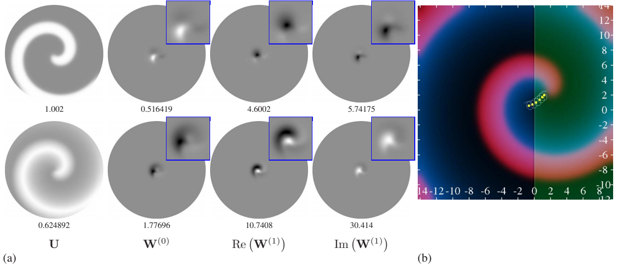
FIG. 1. (Color online) (a) Solutions of the nonlinear problem (3) and the adjoint linearized problem (9,10), i.e., the response functions, as density plots. Barkley model, \rho_{\max}=12.8 , N_\rho=1280 . Numbers under the density plots are their amplitudes A : white in the plot corresponds to the value A and black corresponds to the value -A of the designated field. Upper row: first components ( u ), lower row: second components ( v ). The central areas of \mathbf{W}^{(n)} , n=0, 1 , are also shown magnified in the small corner panels. (b) Snapshot of spiral wave in the Barkley model ( u : red color component, v : blue color component), drifting in a stepwise inhomogeneity of parameter c (green color component). The thin white line is the trace of the tip of the spiral in the course of a few preceding rotations. Yellow circles are positions of the centers calculated as period-averaged positions of the tip.
