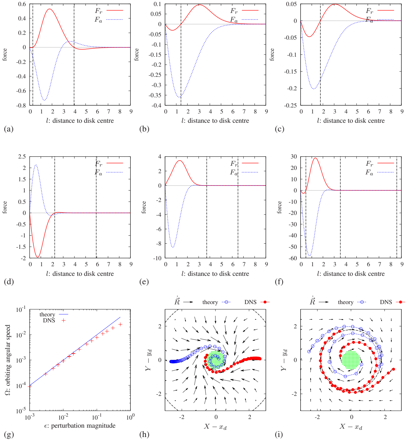
FIG. 5. (Color online) Drift around disk-shaped inhomogeneity Eqs. (45) and (48) of radius R_{in}=0.56 . First row: theoretical predictions for the drift speed components as functions of the distance to the disk center, l=((X-x_d)^2+(Y-y_d)^2)^{1/2} , for inhomogeneity in parameters (a) \alpha , (b) \beta , and (c) \gamma , in the FitzHugh-Nagumo model. Second row: same for Barkley model, steps in parameters (d) a , (e) b and (f) c . Third row: comparison of theoretical predictions with DNS. (g) Angular speed of the established orbital movement around the inhomogeneity site as on panel (i), as a function of inhomogeneity strength. (h) A phase portrait of the drift in the Barkley model in theory, Eq. (41), and DNS, Eqs. (4), (45), and (48), with disk-shape inhomogeneity (green) of parameter b [corresponds to panel (e)], at \epsilon=10^{-2} . Shown are the theoretical vector field (black arrows; the lengths are nonlinearly scaled for visualization), a selection of theoretical trajectories (red filled circles) and a selection of numerical trajectories (blue open circles) of the centers of the spiral wave. Dash-dotted circles correspond to the roots of the theoretical radial component of the drift force. (i) A phase portrait of the drift in the FitzHugh-Nagumo model with inhomogeneity of parameter \gamma [corresponds to panel (c)], \epsilon=0.3 . Notation is the same as in panel (h).
