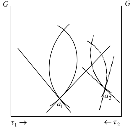
Figure 3: Multiple equilibria
