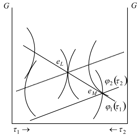
Figure 2: Incentive incompatibility
