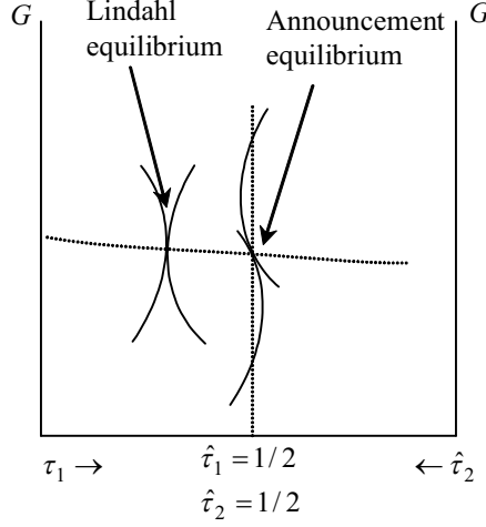
Figure 4: Announcement equilibrium
