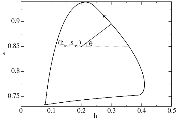
Fig. 2 Oscillation of an uncoupled Hodgkin-Huxley type neuron (21) in the (h, s) -plane. The phase variable is estimated with respect to the reference point (h_{\text{ref}}, s_{\text{ref}}) = (0.2, 0.85) .
