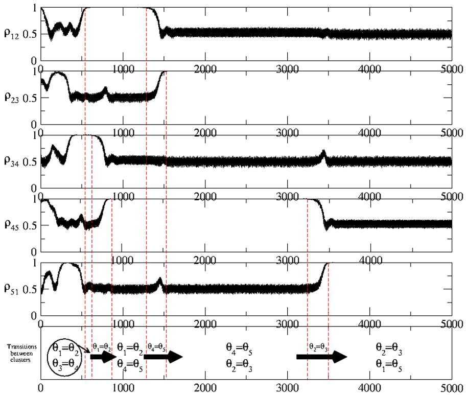
Fig. 5 A trajectory of the system of N = 5 neural oscillators (21) for \tau_d = 1.9 approaching to a heteroclinic cycle between two clusters. In the first five graphs, five synchronization indices are plotted (after block averaging of size 1000) for different synchronized pairs, whereas in the last graph transitions between synchronized clusters are illustrated.
