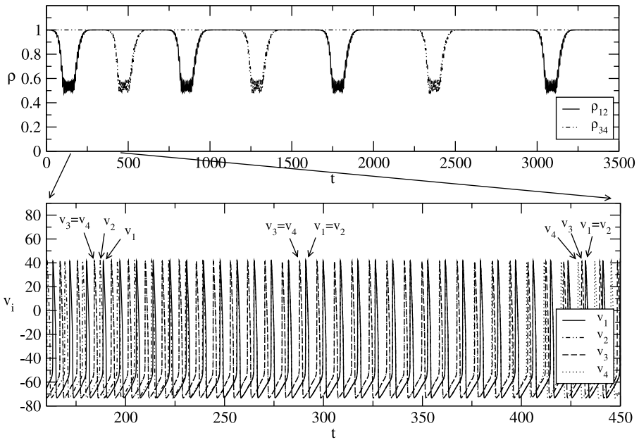
Fig. 3 A solution of (21) for N = 4 and \tau_d = 1.8 approaching to a heteroclinic cycle between two cluster states with the same clustering \{\{1, 2\}, \{3, 4\}\} but a different effective phase difference. In the upper graph, synchronization indices for neuron pairs (1, 2) and (3, 4) are plotted (after block averaging of size 1000), whereas in the lower graph a shorter time series of membrane voltages shows transitions between different synchronized clusters.
