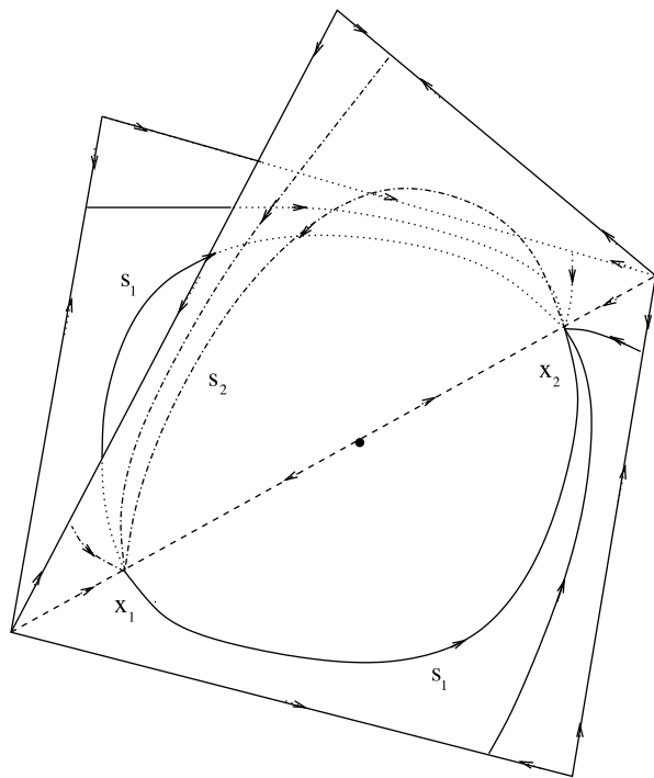
Fig. 4 A robust heteroclinic cycle for four all-to-all coupled phase oscillator system analogous to the cycle found in Figure 3 for the Hodgkin-Huxley type system. The heteroclinic cycle consists of two saddle equilibria x_1 and x_2 and connections s_1 and s_2 on invariant subspaces. The invariant subspaces are embedded in a cube that represents a unit cell for the torus of phase difference space—in this representation the vertices represent in-phase solutions where all oscillators are synchronized. (Adapted from [22].)
