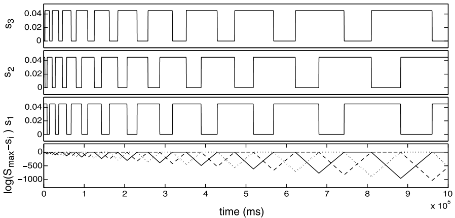
Fig. 1 A trajectory approaching a heteroclinic cycle for the rate model (18) with \epsilon = 10^{-3} and parameters as in Table 1. Observe that the trajectory cycles between the neighbourhoods of three saddle equilibria where two of the three s_i are close to saturated at S_{\max} = 0.045 . The switching dynamics between equilibria continues to slow down indicating that the trajectory is approaching the actual heteroclinic orbit. The bottom panel illustrates this further by showing that the s_i continue to approach the equilibria over the whole duration of the simulation. The simulation is performed using a numerical scheme that carefully resolves the behaviour near the equilibria.
