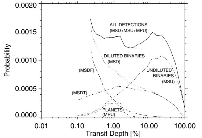
Fig. 3. Adaptation of Fig. 3 from Brown (2003), of probability estimates for a ground based survey in a field in Cygnus. In brackets the notation from Brown where MSD or Diluted Binaries are the sum of MSDF and MSDT. Axes are similar to Fig. 2.
