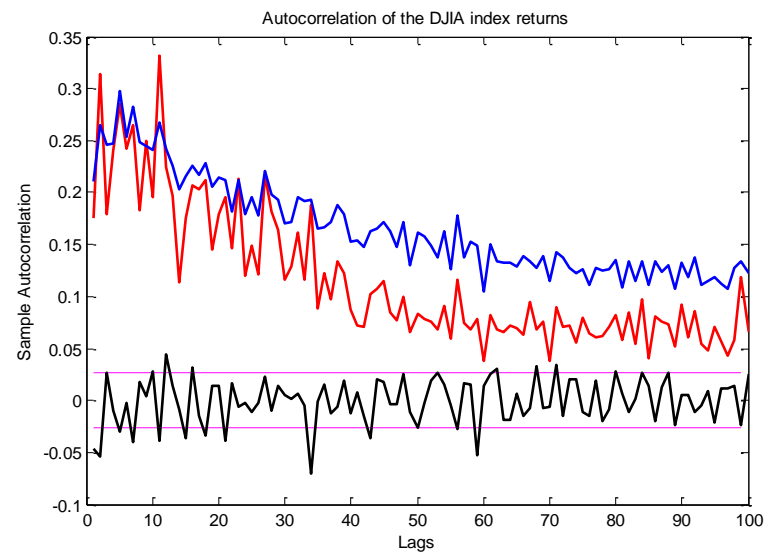
Figure 1. Autocorrelations of returns (black line), absolute returns (blue line,) and squared returns (red line).
