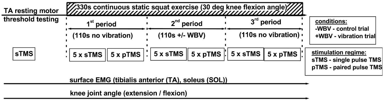
Figure 1. Experimental protocol.
