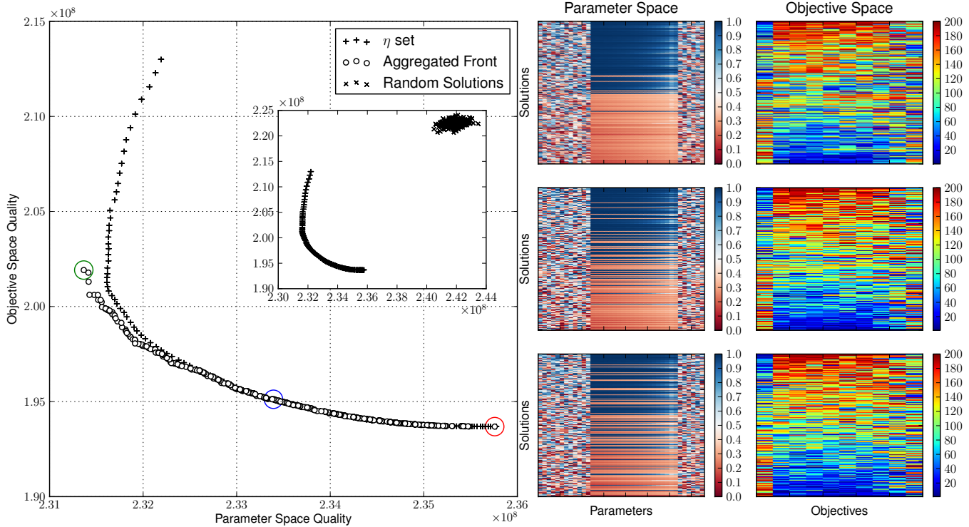
Fig. 7: Optimised trade-off between seriation quality in parameter space g_x(\pi) and objective space g_y(\pi) for the WFG8 solution set. The main panel shows the initial solutions from seriation using the similarity matrix S_\eta (16) as plus symbols (also shown in the insert) and the combined estimated Pareto front from 10 runs of the evolutionary optimiser. The heatmaps on the right-hand side of the figure correspond to optimised solutions marked on the main panel by large circles. The top and bottom visualisations are the solution orderings found by the MOEA which best optimise the parameter space ordering and objective space ordering respectively. The central heatmaps show a solution towards the centre of the Pareto front. Objectives and parameters have also been seriated independently. Parameter space seriation has grouped parameters x roughly into those which control the distance of a solution from the true Pareto front and those which control the angular location of a solution on the front.
