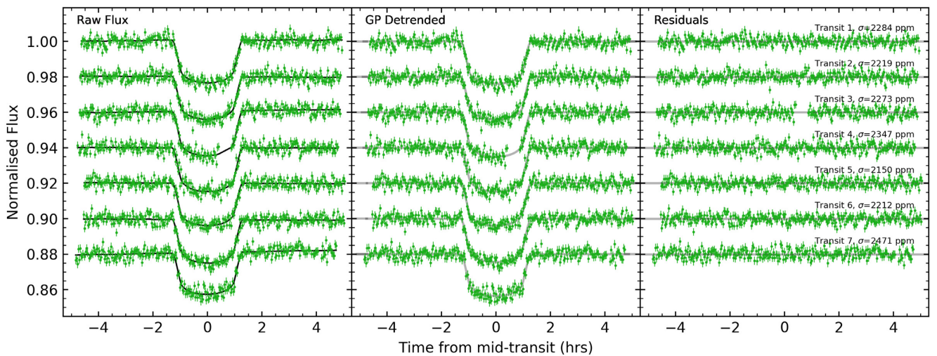
Figure 3. Normalized TESS photometric light curves multiplied by an arbitrary constant. Left: raw extracted light curves with black lines indicating the GP transit plus systematic model fits. Centre: light curves after removal of GP systematic component. The best-fitting transit models from Mandel & Agol (2002) are displayed in grey. Right: residuals after subtraction of best-fitting models from the GP systematic-corrected light curves.
