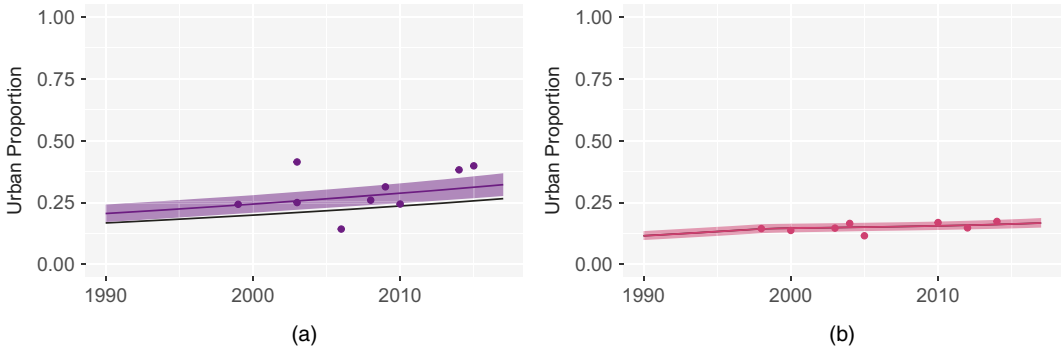
Fig. 6. Predicted mean survey urban proportions (—, —) for (a) Kenya and (b) Malawi, compared with observed survey urban proportions (●, ●) and associated UN urban population estimates (—)
