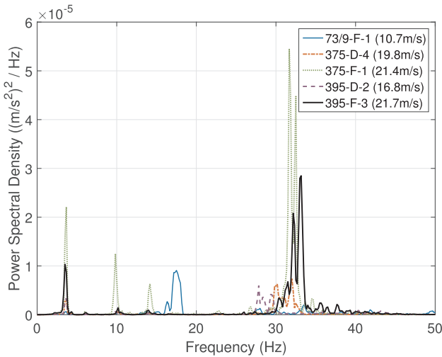
(b) Lateral mid-span acceleration
