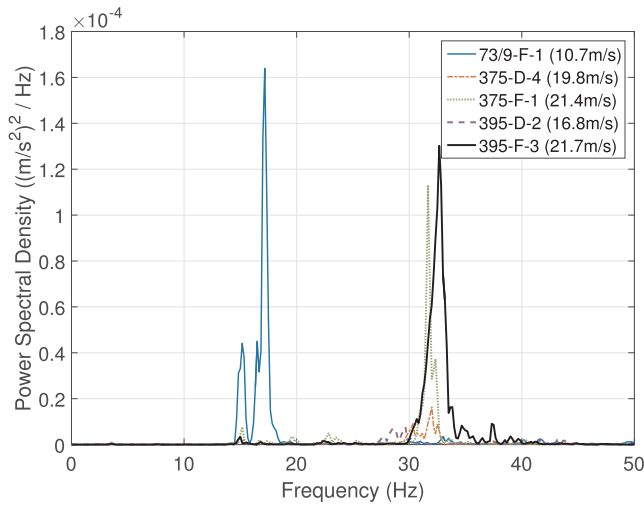
(a) Vertical mid-span acceleration
