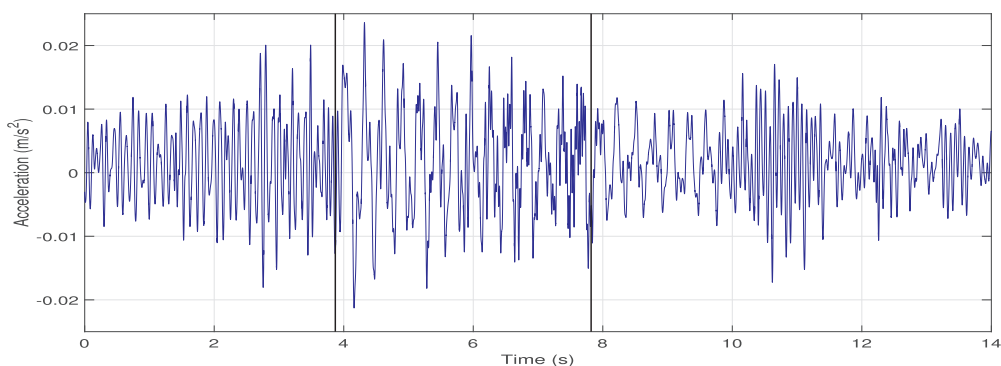
(b) Lateral mid-span acceleration
