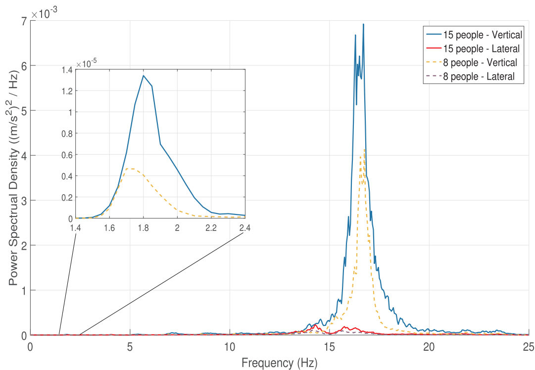
(b) PSD of the acceleration data from crowd loading
