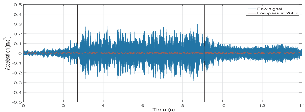
(a) Vertical mid-span acceleration
