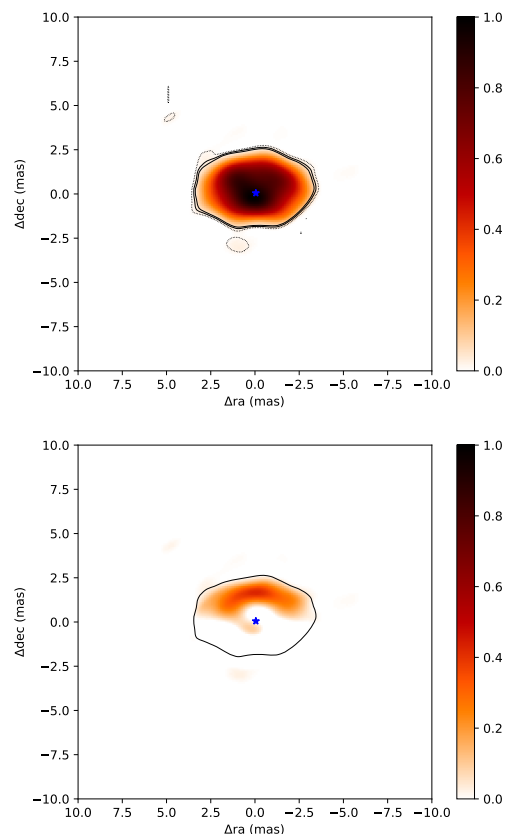
Fig. F.4. Top: Image reconstruction of a sharp model with an inclination of 49^\circ degrees and located at 100 pc. The blue star represents the position of the star. The contours are 1 (dotted), 2, and 3-sigma pixel significance levels. Bottom: Corresponding asymmetry map with the contour representing the 2\text{-}\sigma significance level.
