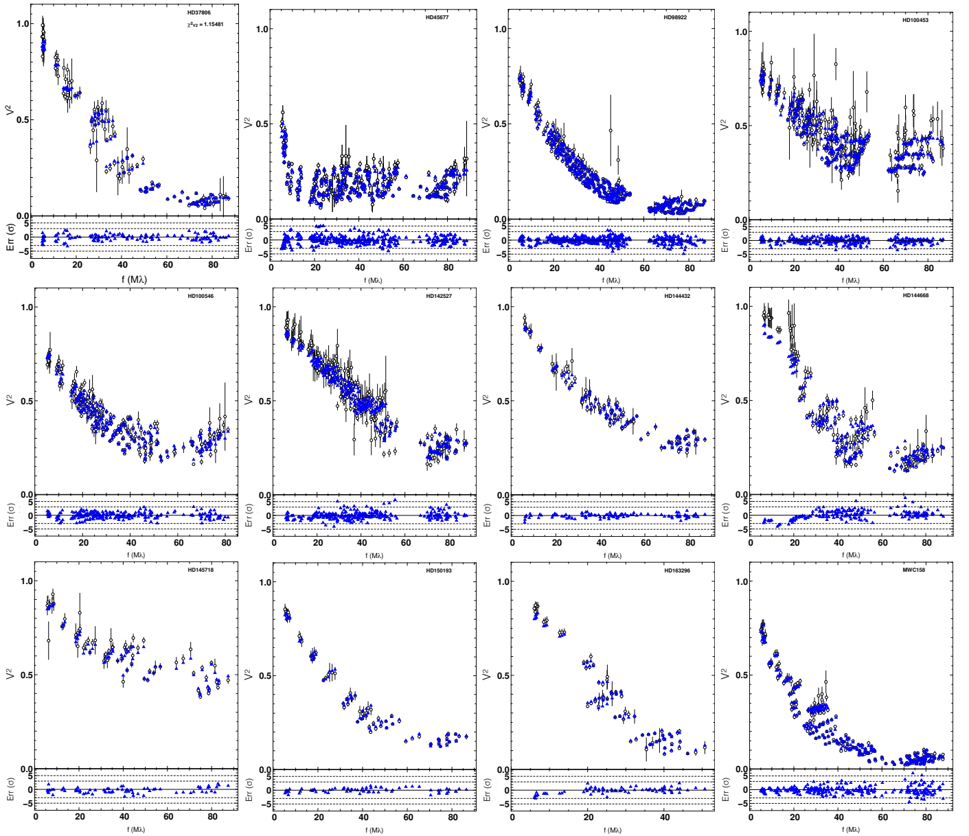
Fig. F.5. Squared visibilities of the dataset and the images. For each target the top panel shows the squared visibilities for the data (black circles) and the image (blue triangles). The bottom panel shows the residuals normalized by the error bars on each data point.
