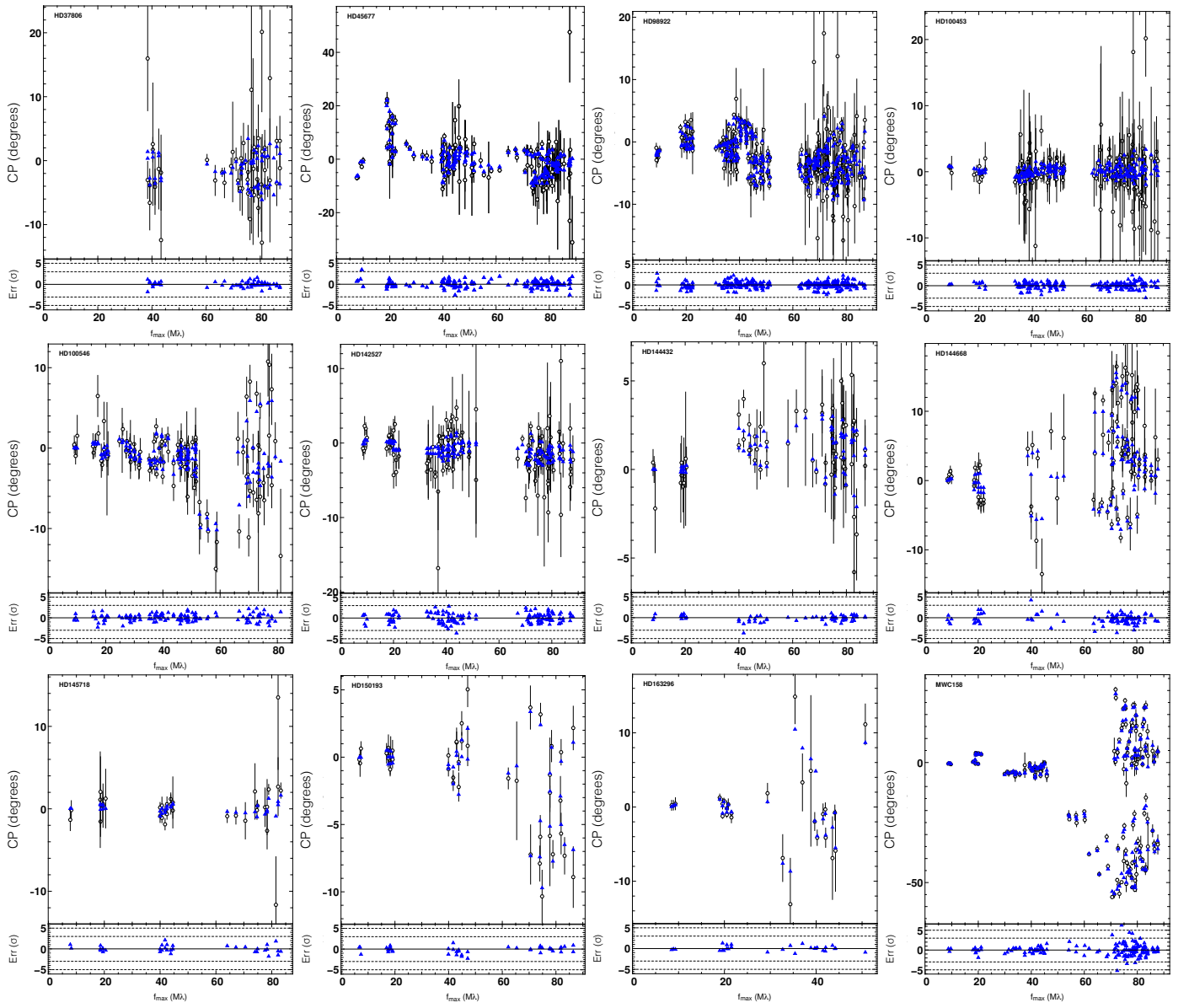
Fig. F.7. Closure phases of the dataset and the images. For each target, the top panel shows the closure phases for the data (black circles) and the image (blue triangles). The bottom panel shows the residuals normalized by the error bars on each data point.
