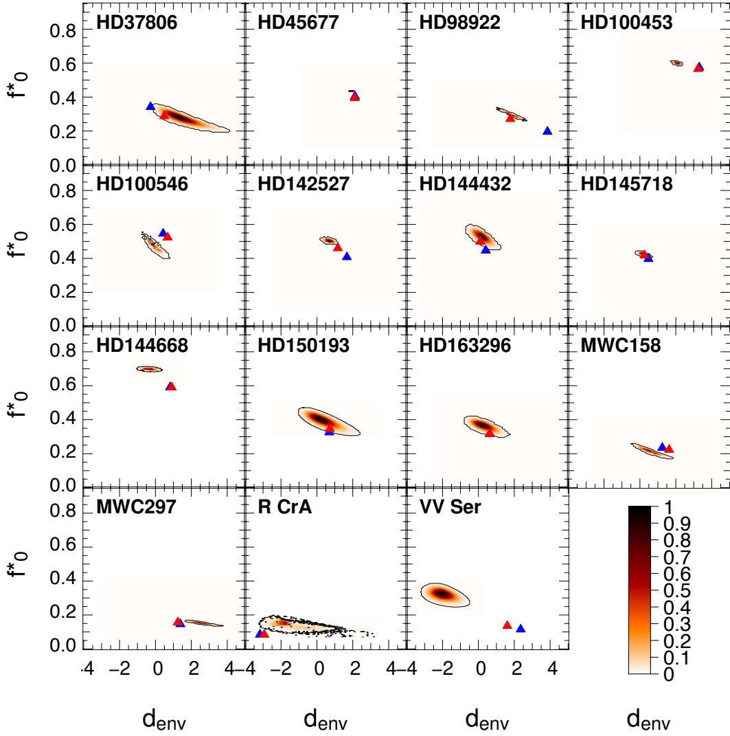
Fig. A.1. Significance maps for the chromatic parameters of each object. Contours indicate 5- \sigma likelihood of the parameters for the actual dataset (black). Blue and red triangles represent the chromatic parameters from L17 for ring models with first order and second order modulations, respectively.
