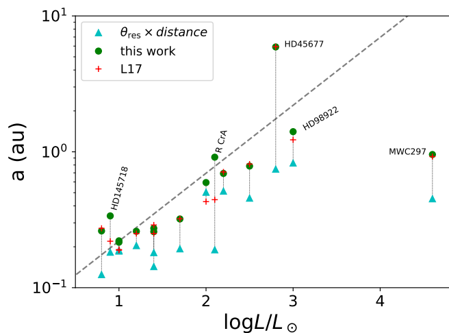
Fig. 8. Size-luminosity relation. The green circles are the sizes measured from images, red crosses are the sizes from parametric models as determined in L17, and cyan triangles are the physical spatial resolution reached by our observations. The two size estimations and the spatial resolution are linked by a vertical dotted line. The dashed gray line represents the theoretical sublimation radius.
