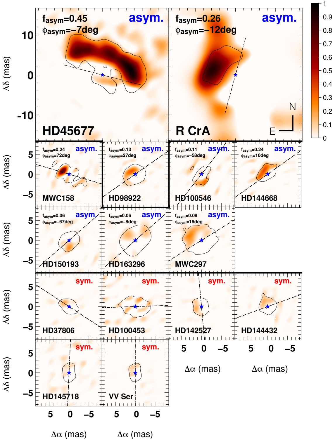
Fig. 4. Asymmetry maps of the targets classified the same way as in Fig. 2. The blue star represents the central star, the solid black contour represents the 3\text{-}\sigma significance profile, and the dot-dashed line represents the orientation of the major-axis from parametric fitting. The targets with three closure phase points or more with a significance of 5\text{-}\sigma are indicated as “asym.”
