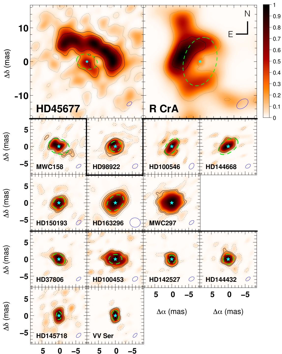
Fig. 2. Reconstructed images of the Herbig Ae/Be targets separated in three groups. Top: the centrally depressed objects; middle: the centrally peaked and asymmetric objects; bottom: the centrally peaked and asymmetric objects. The cyan star marks the position of the central star, which has been subtracted, the black contours indicate the significance at 1 (dashed line), 3, and 5- \sigma (solid lines), and the blue ellipse shows the size of the beam. The green dashed ellipses represent the theoretical dust sublimation radius (see Sect. 5.5).
