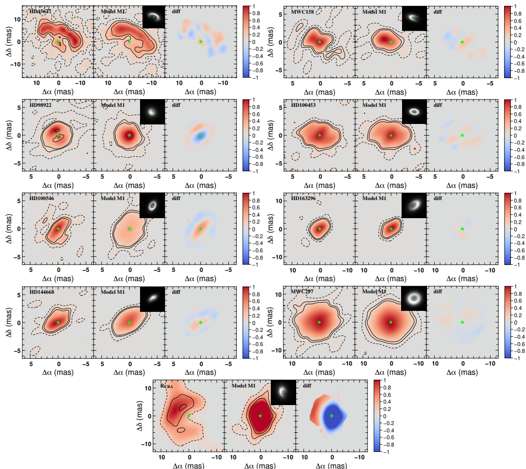
Fig. 7. Comparison between the image reconstructions on each target from the dataset (left panels) and the synthetic data based on the best-fit m1 model from L17 (middle panels) and the difference (right panels) in the 3\text{-}\sigma significance area of the image. In the top-right corner of the model image reconstruction, there is the high resolution image of the parametric model. The green star represents the position of the central star.
