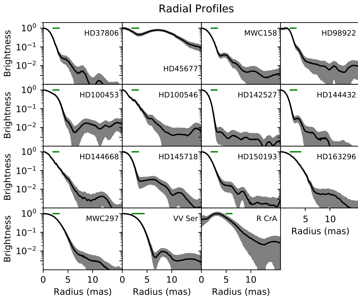
Fig. 3. Radial profiles of the reconstructed images of Fig. 2. Black solid lines: radial profiles from images with 5- \sigma error bars in color shades. The green line shows the azimuthally averaged size of the interferometric beam.
