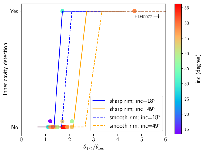
Fig. 5. Inner hole detection in image reconstructions from (a) (continuous lines) synthetic observations of radiative transfer models and (b) (dots) our targets. Models with two radial distributions and two inclinations are included, see legend and text. Some dots are offset to avoid overlap.
