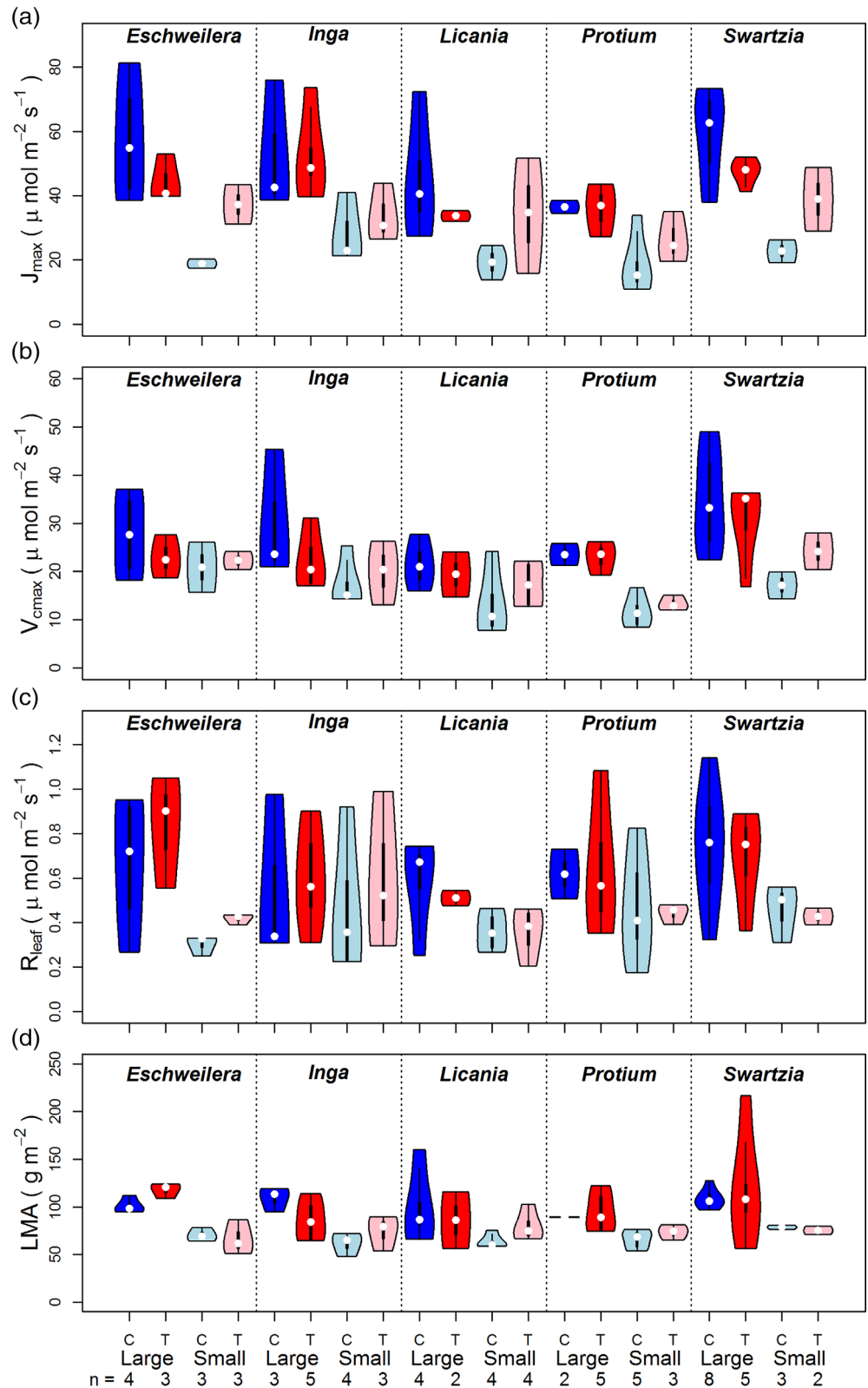
FIGURE 5 Violin plots comparing J_{\max} (a), V_{\max} (b), R_{\text{leaf}} (c) and leaf mass per area (LMA; [d]) between the Control (C) and TFE (T) treatment for large (>20 cm DBH) and small (1–10 cm DBH) trees across the five most common genera: Eschweilera , Inga , Licania , Protium , Swartzia . All genera with n \geq 2 for each of the four categories are presented. White dots represent the median, thick grey lines represent the interquartile range and thin grey lines represent the mean \pm 1.5 SEs [Colour figure can be viewed at wileyonlinelibrary.com ]
