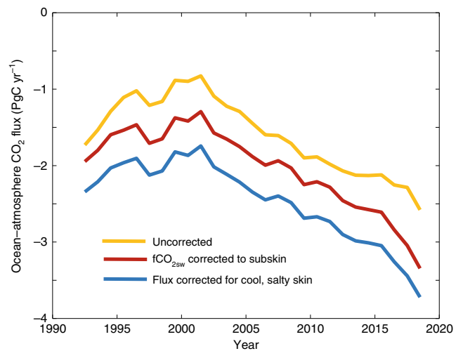
Fig. 1 Effect of near-surface temperature corrections. Global air–sea flux calculated by interpolating SOCAT gridded data using a neural network technique 8 , followed by the gas exchange equation applied to the ocean mass boundary layer. The net flux into the ocean is shown as negative, following convention. The uncorrected curve uses the SOCAT fCO 2 at inlet temperature as usually done. Correction of the data to a satellite-derived subskin temperature is shown, and the additional change in flux due to a thermal skin assumed to be cooler and saltier than the subskin by 0.17 K 15 and 0.1 salinity units 11 . Excludes the Arctic and some regional seas—ocean regions included are shown in Supplementary Fig. 2.
