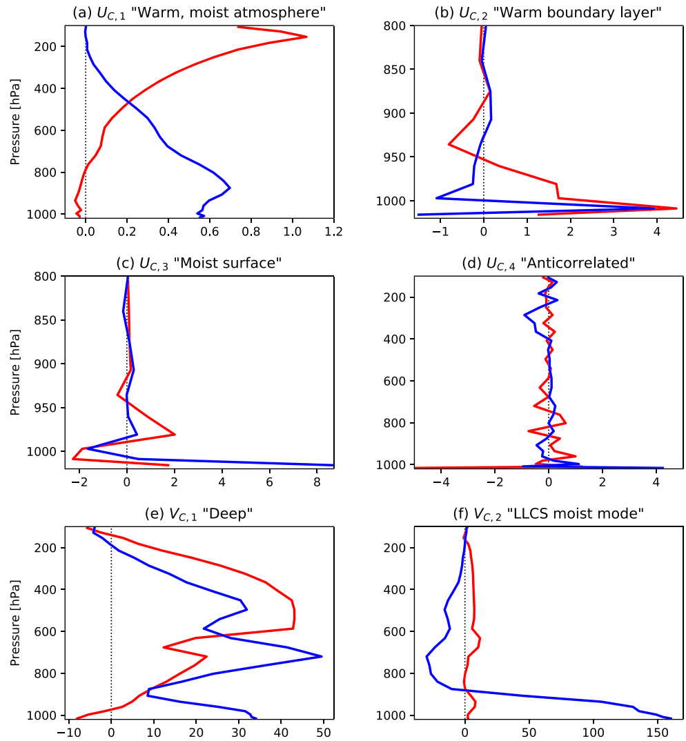
Figure 4. (a–d) The first four joint input eigenvectors for the LLCS CON and GR CON data sets. As in Figure 2, dry temperature components are red, and moist components are blue in units of K. (e, f) The first two joint output eigenvectors. As in Figure 1, the red lines are the effective convective heating rate, Q_1 , and the blue lines are the effective convective drying rate, Q_2 , in units of \text{K day}^{-1} . Note the different horizontal and vertical scales on each panel, in particular the vertical scales for (b) and (c), which show the boundary layer only.
