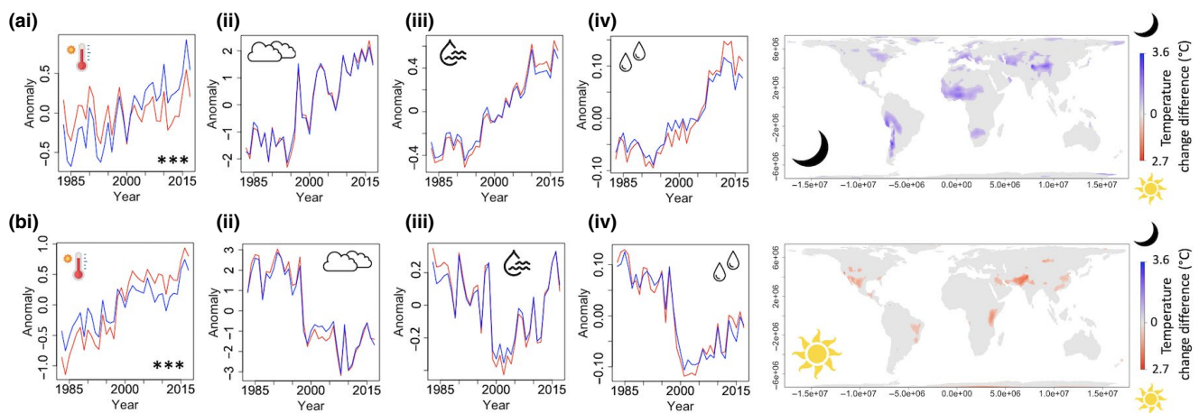
FIGURE 3 Diel asymmetry in the changing climate at extremes of >0.5^{\circ}\text{C} warming asymmetry. We show the relationship between warming asymmetry and diurnal asymmetric change in cloud cover, specific humidity and precipitation, in regions where (a) the night-time minimum temperature warmed by >0.5^{\circ}\text{C} more than the daytime maximum temperature, and (b) the daytime maximum temperature warmed by >0.5^{\circ}\text{C} more than the night-time minimum temperature. We give the anomaly plots for of annual daytime (red) and annual mean night-time (blue) relative to the 35 year mean of (i) temperature ( ^{\circ}\text{C} ), (ii) cloud cover (%), (iii) specific humidity (g/m 3 ) and (iv) precipitation (mm/6 hr). *** denotes a statistical significance of the interaction between year and a binary day/night variable as p < .001 . The global map was created by subtracting the change in daytime maximum temperature from the change in night-time minimum temperature, and masking regions where the warming threshold of >0.5^{\circ}\text{C} was not met. Coloured areas illustrate where warming of >0.5^{\circ}\text{C} that has occurred more in the daytime (red) or the night-time (blue). Negative values for temperature change difference were converted to absolute values and the direction of greater change is represented by a sun (daytime) or a moon (night-time). The map projections are Behrmann's equal area
