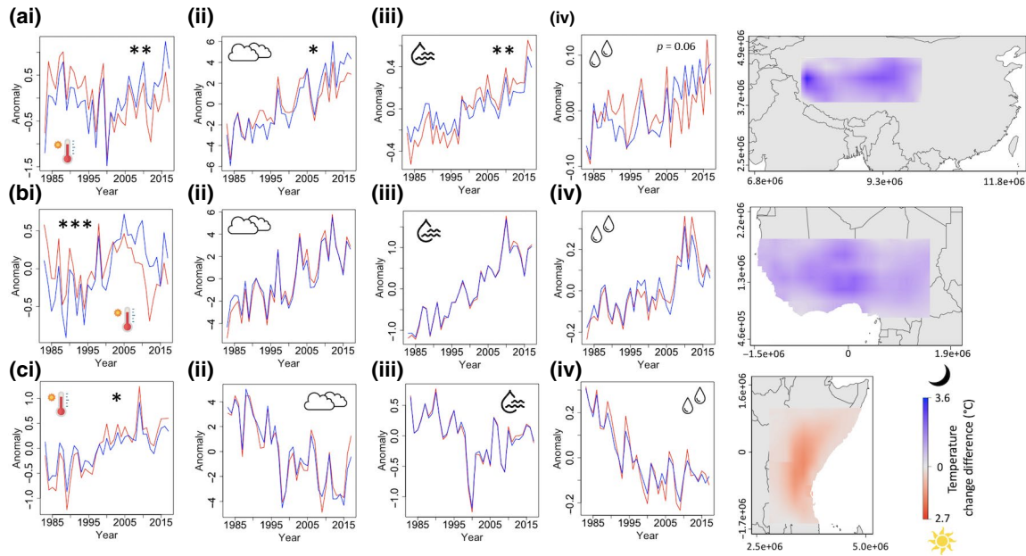
FIGURE 4 Diel asymmetry in the changing climate at smaller spatial scales. Warming asymmetry and diurnal asymmetric change in cloud cover, specific humidity and precipitation in (a) the Tibetan Plateau (33°N, 88°E), (b) West Africa (09°N, 02°E) and (c) East Africa (05°S, 36°E). We show the anomaly plots for annual mean daytime (red) and annual mean night-time (blue) relative to the 35 year mean of (i) temperature (°C), (ii) cloud cover (%), (iii) specific humidity ( \text{g/m}^3 ) and (iv) precipitation ( \text{mm}/6 \text{ hr} ). Statistical significance of the interaction between year and a binary day/night variable are shown as; * p < .05 ; ** p < .01 ; *** p < .001 . The global map was created by subtracting the change in daytime maximum temperature from the change in night-time minimum temperature. Coloured areas demarcate the degree to which the days warmed more quickly (red) or the nights warmed more quickly (blue). Negative values for temperature change difference were converted to absolute values and the direction of greater change is represented by a sun (daytime) or a moon (night-time). The map projections are Behrmann's equal area
