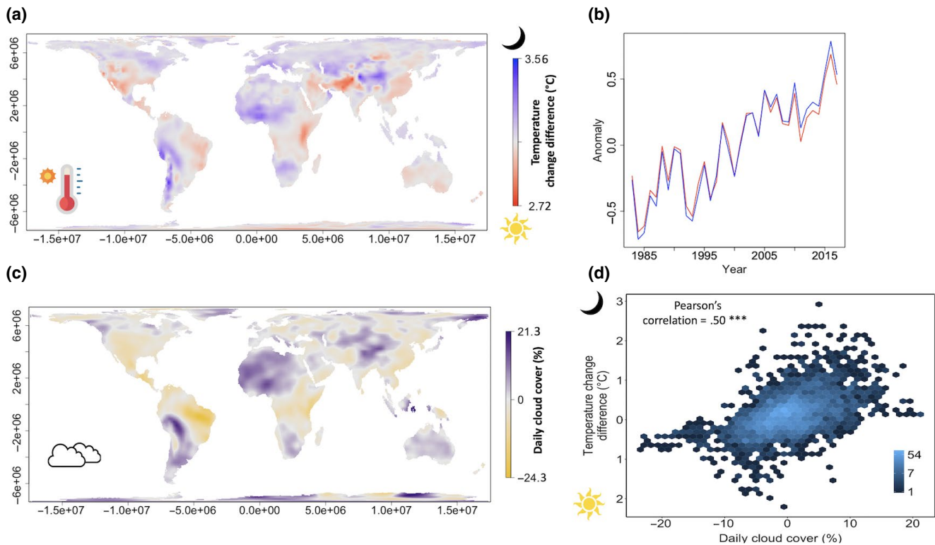
FIGURE 1 Spatial variation in diel warming asymmetry and change in daily cloud cover. (a) Spatial variation in the warming asymmetry between daytime maximum temperature and night-time minimum temperature. In each pixel the 35 year change in the daytime temperature was subtracted from the 35 year change in the night-time temperature. Red illustrates where the daytime has changed more rapidly and blue where the night-time has done so. (b) Anomaly plot of annual mean daytime maximum temperature (red) and annual mean night-time minimum temperature (blue) relative to the 35 year mean. (c) Spatial variation in cloud cover change. Pixels show the 35 year trend in mean daily cloud cover where yellow illustrates where cloud cover has decreased and purple where cloud cover has increased. (d) The relationship between the difference in change in temperature between the daytime and night-time and the change in daily cloud cover. The legend shows the log of the number of pixels, and *** denotes a statistical significance of p < .001 . Negative values for temperature change difference were converted to absolute values and the direction of greater change is represented by a sun (daytime) or a moon (night-time). The map projections are Behrmann's equal area
