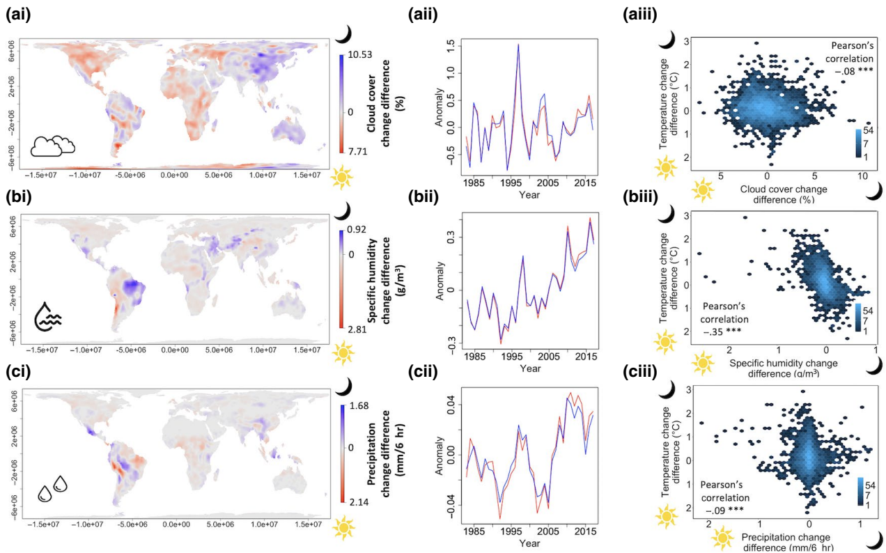
FIGURE 2 Spatial variation in diel asymmetry in cloud cover, specific humidity and precipitation. We show spatial variation in asymmetry between mean daytime and mean night-time (a) cloud cover (%), (b) specific humidity (g/m 3 ), and (c) precipitation (mm/6 hr). (ai, bi, ci) In each pixel the 35 year change in the daytime was subtracted from the 35 year change in the night-time. Red illustrates where the daytime has changed more rapidly and blue where the night-time has changed more rapidly. (a(ii), b(ii), c(ii)) Anomaly plots of annual mean daytime (red) and annual mean night-time (blue) relative to the 35 year mean. (a(iii), b(iii), c(iii)) The relationship between the difference in change in temperature between the daytime maximum and night-time minimum and the change difference between the mean daytime and mean night-time climate variable. The legend shows the log of the number of pixels, and *** denotes a statistical significance of p < .001 . Negative values for the change difference were converted to absolute values and the direction of greater change is represented by a sun (daytime) or a moon (night-time). Therefore, a negative correlation in (iii) illustrates that greater night-time warming is associated with greater change in the climate variable during the daytime, while higher daytime temperatures are associated with greater change in the climate variable during the night-time. The map projections are Behrmann's equal area
