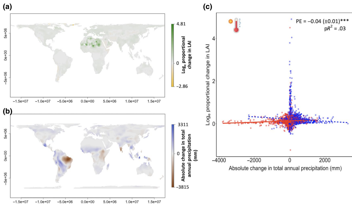
FIGURE 5 The response of LAI to diel warming asymmetry and absolute change in precipitation. We show spatial variation in (a) the \log_e proportional change in LAI between 1983 and 2017, and (b) the absolute change in total annual precipitation for the same period. (c) Relationship between the \log_e proportional change in LAI and the interaction between the absolute change in total annual precipitation and a binary factor of whether warming occurred more during the daytime (red) or the night-time (blue). We give the linear lines of best fit for the daytime (red, solid) and the night-time (blue, dashed), and the parameter estimate (PE) and standard error for the interaction. *** denotes a statistical significance of p < .0001 . The pR^2 is McFadden's. The map projections are Behrmann's equal area
