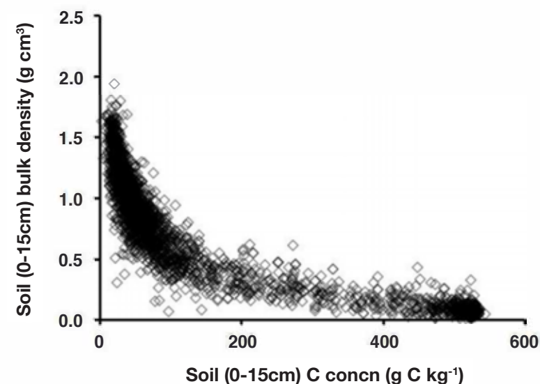
Figure 12: Countryside Survey, plot of soil (0–15 cm) bulk density against carbon concentration in 2007.
