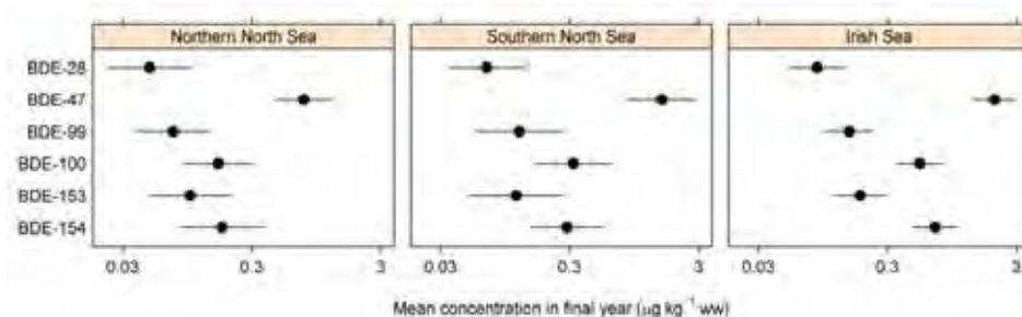
Figure 32: Estimated mean sea concentration profile of PBDE in final year, with 95% confidence limits
