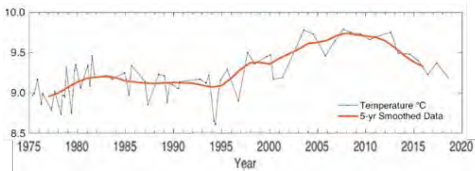
Figure 4: Rockall Trough temperature: 1975 - 2020
