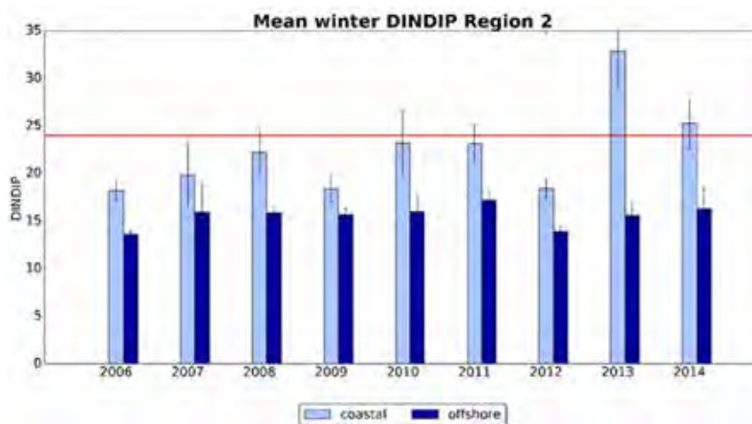
Figure 17: Mean winter ratios of DIN:DIP in the northern North Sea between 2006 and 2014
