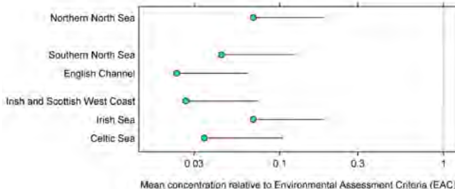
Figure 29: Mean concentrations of PAH in shellfish samples, relative to EAC and BAC: 1995 - 2015
