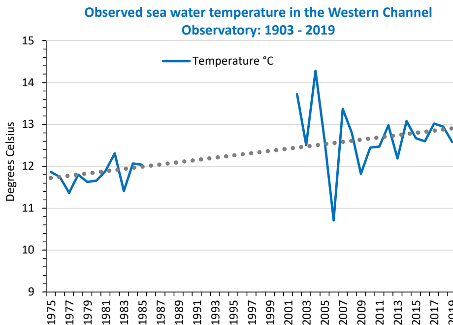
Figure 5: Seawater temperature from the Western Channel Observatory: 1975 - 2019
