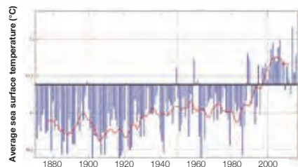
Sea surface temperature
