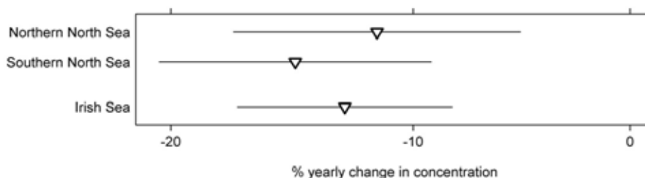
Figure 33: Average trend in concentrations in biota of PBDE congeners, per sub-region. Downward triangle: significant downward trend
