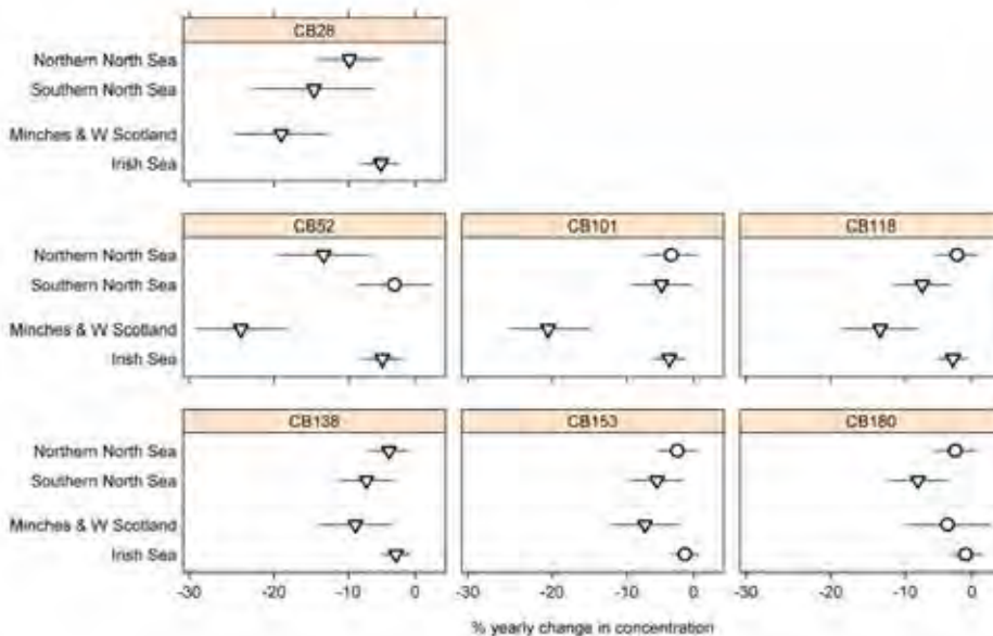
Figure 31: Average annual trends in PCB concentrations in biota by biogeographic region, with 95% confidence limits. Upwards triangle : upward trend. Downwards triangle : downward trend. Circle : no change.
