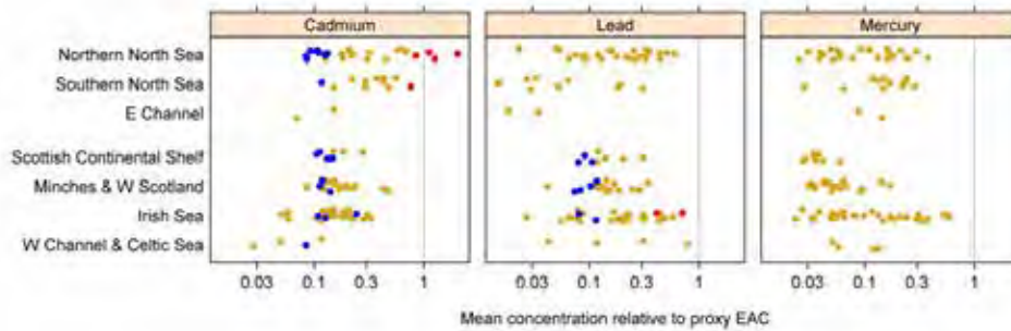
Figure 34: Mean concentrations of cadmium, lead, and mercury relative to individual proxy EACs, by biogeographic sub-region. Blue: mean concentration significantly ( p < 0.05 ) below the Background Assessment Concentration. Orange: mean concentration significantly ( p < 0.05 ) below the proxy Environmental Assessment Criteria. Red: mean concentration not significantly below the proxy Environmental Assessment Criteria.
