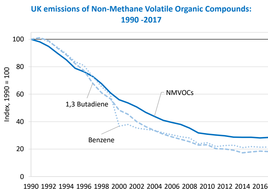
Figure 25: UK Emissions of non-methane volatile organic compounds (NMVOCs)
