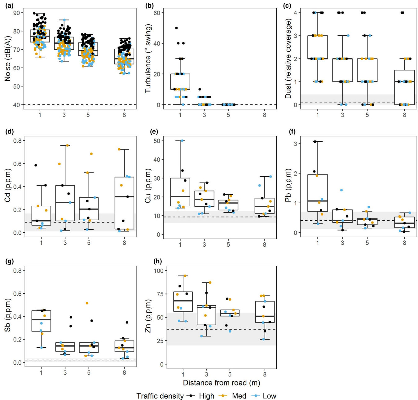
FIGURE 1 The spatial distribution of pollution in road verges: (a) noise (maximum dB(A) when a vehicle passed), (b) turbulence (the maximum angle ( ^{\circ} ) swing, from vertical, of a suspended pollinator when a vehicle passed), (c) dust (the relative coverage of dust on a piece of sticky tape after 4 days), and (d–h) metals (cadmium, copper, lead, antimony and zinc). Dashed lines in a–b are background levels, while dashed lines with grey areas in c–h are the M \pm SD at control sites (>50 m from roads). See Table 1 for descriptions of methods for measuring each form of pollution. Traffic density (vehicles/hr) categories are: low 100–250, medium 300–400 and high 900–1,500. Data points are jittered for clarity of presentation. Samples sizes ( n ) per boxplot are (a): 135, (b): 45, (c): 27, (d–h): 9. Four metal outliers have been cropped for clarity of presentation (all for distance from the road = 1 m): 192.983 ppm Cu at site 2 (high traffic), 1,456 ppm Sb at site 1 (high traffic), 622.200 ppm Zn at site 2 (high traffic), and 7.959 ppm Pb at site 8 (low traffic). Statistical analyses are provided in Appendix S3
