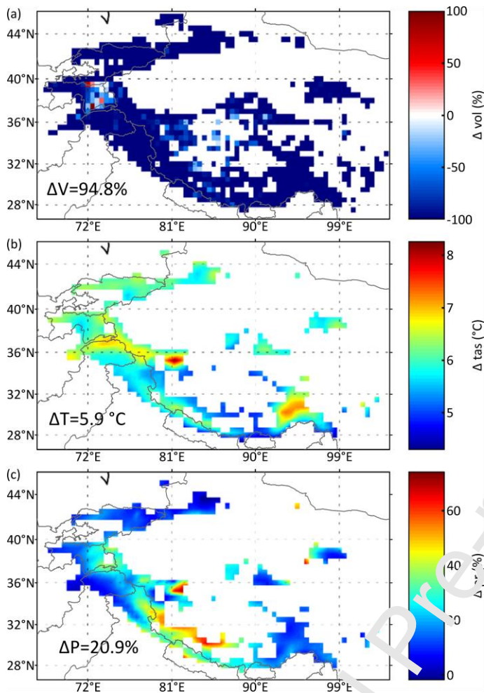
Figure 1. (a) Ensemble glacier mean glacier volume loss, (b) air temperature change, and (c) precipitation change between the historical period (1980–2010) and the end of this century (2067–2097) over glaciated grid points in the high mountains of Asia. See the Supplementary Methods for the description of the climate modelling implemented here.
