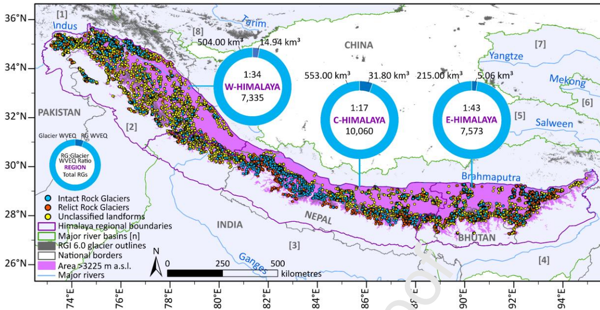
Figure 3. Map depicting the distribution of rock glaciers across the Himalaya. Rock glaciers with unclassified dynamic status (i.e. landforms not digitised as part of the sampling strategy) are included here for completeness. The total rock glacier number, rock glacier and glacier WVEQ and rock glacier: glacier WVEQ ratios for the west, central and east Himalaya regions are shown. These regional outlines were derived from Bolch et al. (2012). Note that rock glacier WVEQ values presented here assume 50% (average) ice content by volume. The area >3,225 m a.s.l. represents the terrain above the minimum elevation at which rock glaciers were found. The major river basin boundaries are also shown: [1] Amu Darya, [2] Indus, [3] Ganges, [4] Brahmaputra, [5] Salween, [6] Mekong, [7] Yangtze, and [8] Tarim.
