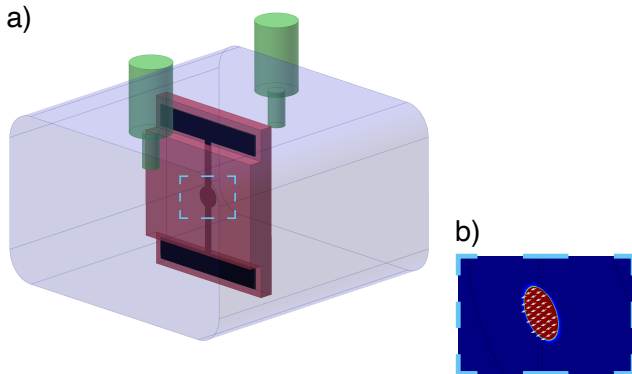
FIG. 17. a) Schematic of a nanofluidic device (light red area) composed of a nanoscale capacitor (dark red area) terminated by two large antennas (black area), embedded in a 3D superconducting microwave cavity (blue area), which can be readout with a pair of pin couplers (green areas). b) Numerical simulation of the electric field mode shape in this type of resonator showing the focusing of the electric field inside the nanoscale capacitor with arb. unit scale (red is for high intensity and blue for low intensity).
