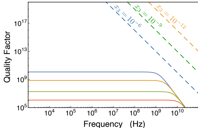
FIG. 7. Quality factor of an acoustic mode \mathbf{q} , computed using the expression of the damping rate given at Eq. 29 for 3-phonon interaction, as a function of the mode frequency \Omega_{\mathbf{q}}/2\pi at temperatures 10 (blue line), 20 (orange line), 50 (green line) and 100 mK (red line). The quality factor is computed from Eq. 40 for phonon- ^3\text{He} interaction processes is shown for different ^3\text{He} concentrations: x_3 = 10^{-6} (blue dashed line), x_3 = 10^{-9} (green dashed line) and x_3 = 10^{-12} (orange dashed line).
