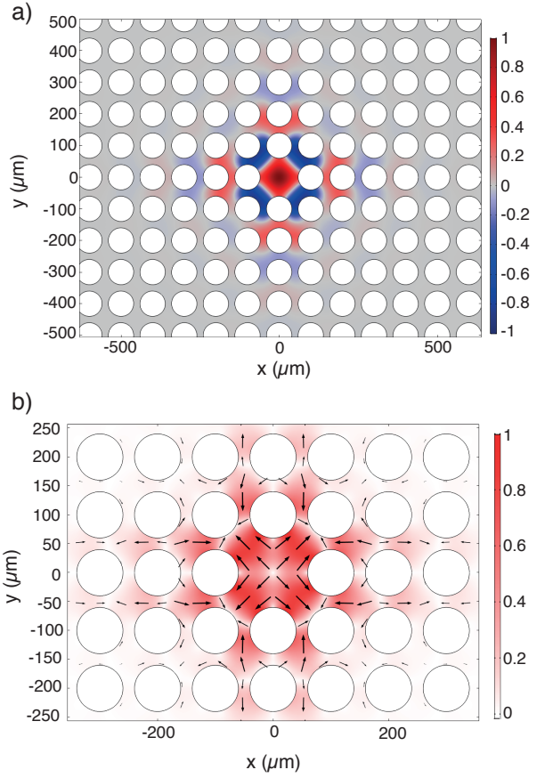
FIG. 12. Mode shape of a point defect acoustic mode ( \Omega_a/2\pi=1.34 \text{ MHz} ) at the center of a 2D sonic crystal of parameters a_1 = 100 \mu\text{m} and a_2 = 80 \mu\text{m} . (a) Acoustic pressure field mode shape, (b) velocity field mode shape indicating the velocity magnitude (color scale) and direction (black arrows).
