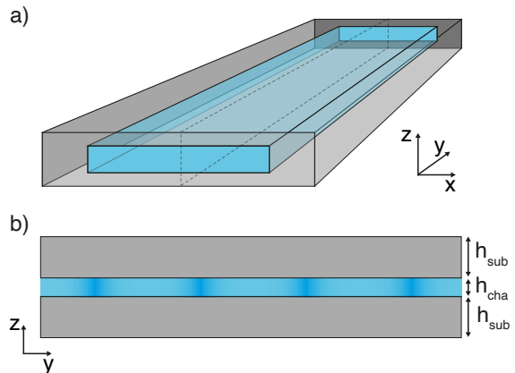
FIG. 9. a) Schematic of a rectangular nanofluidic channel made in a solid substrate (grey color), and filled with superfluid ^4\text{He} (blue color) b) Cross-section of the nanofluidic channel taken along the black dashed line rectangle drawn in (a) showing an acoustic wave propagating in the y -direction. In the range of parameters used in this proposal, such nanofluidic channel acts like an acoustic waveguide.
