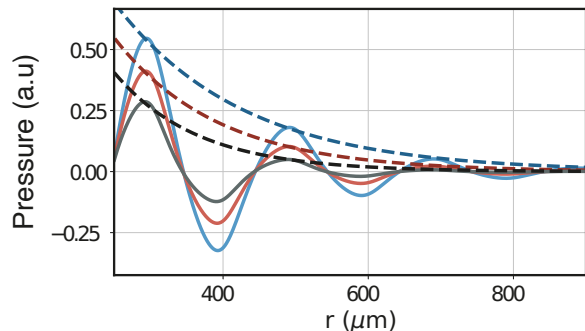
FIG. 14. Calculated pressure field outside of the defect at the mode frequency ( \Omega_a/2\pi = 1.34 \text{ MHz} ) as a function of the distance to the centre of the point defect for 3 sonic crystals with parameters a_1 = 100 \mu\text{m} , a_2 = 75 \mu\text{m} (blue line), 80 \mu\text{m} (red line), and 85 \mu\text{m} (black line). The pressure field is normalized by the maximum of the field at the centre of the point defect. The envelope of the normalized pressure field is fitted with an exponential function p(r) = \exp(-r/l_c) where l_c is the characteristic decay length extracted from the fit and given by l_c = 176 \mu\text{m} (dashed blue line), l_c = 143 \mu\text{m} (dashed red line), l_c = 115 \mu\text{m} (dashed black line).
