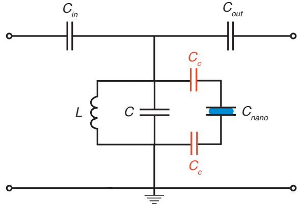
FIG. 18. Circuit diagram showing the coupling between the nanoscale capacitor ( C_{\text{nano}} ) and the 3D superconducting microwave cavity with effective inductance L and capacitance C . The coupling capacitors ( C_c ) couple the in-cavity field to the nanoscale capacitor. The in and out coupling capacitors ( C_{\text{in}} and C_{\text{out}} ) represent the pin coupling to the measurement transmission line.
