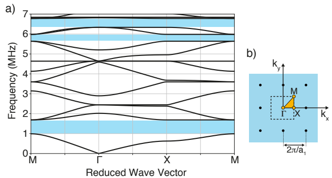
FIG. 10. a) Calculated phononic band structure for a square lattice of cylindrical pillars in a superfluid ^4\text{He} . The lattice spacing is a_1 = 100 \mu\text{m} and the pillar diameter is a_2 = 90 \mu\text{m} . Three bandgaps are visible (blue bands) in this structures. b) The reciprocal lattice showing the irreducible Brillouin zone (orange triangle), and the characteristic points: \Gamma , M and X .
