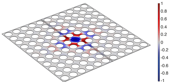
FIG. 19. Illustration of the overlap between the pressure field (normalized color scale) of the sonic crystal's defect mode and the electric field confined in the nanoscale capacitor located at the center of defect where the pressure field is maximum leading to a mode overlap function close to unity.
