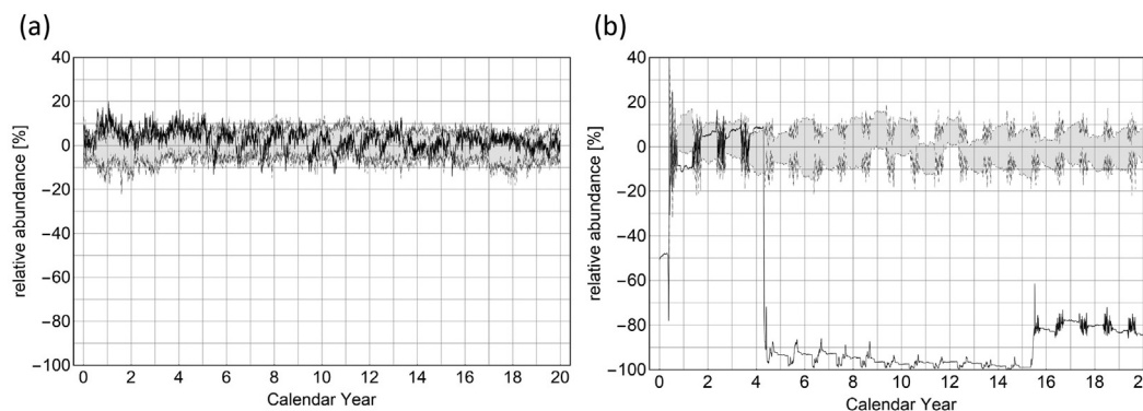
Fig. 1. Outputs for (a) earthworm and (b) springtail model. Models are run for 5 years pre-treatment, 10 years pesticide treatment (2 applications per year at approved application rates) and 5 years post treatment. Grey shaded area represents the normal operating range and black lines are the population response relative to no-application controls (For full description of methods and results, see Van den Brink et al., 2021).
