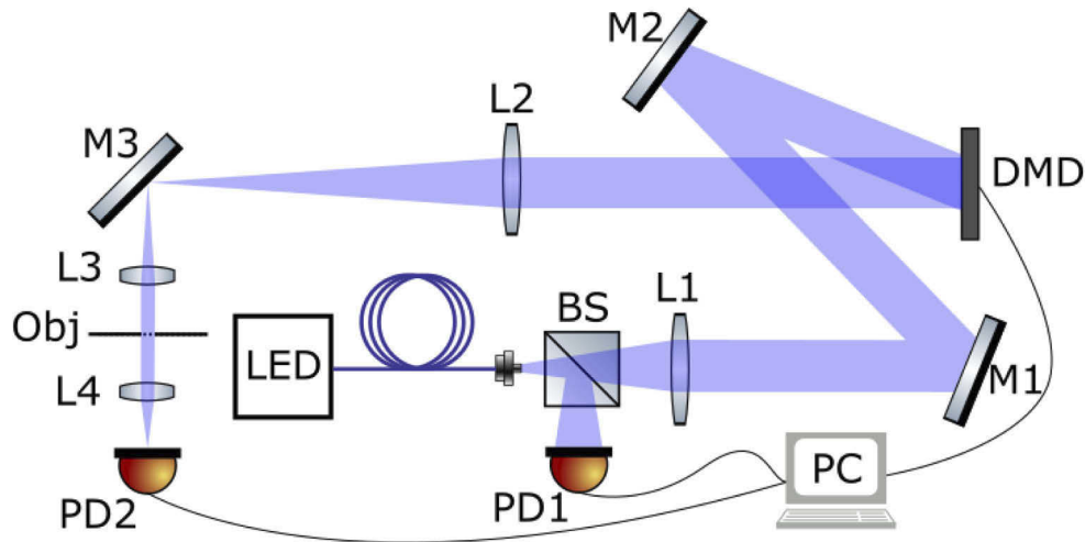
Fig. 2. Schematic of the experimental setup. A fibre coupled blue LED is collimated and illuminates a DMD. The DMD is imaged at reduced magnification by lenses L2 and L3 onto a planar transmissive object (Obj). The transmitted light is then collected by lens L4 and focused onto photodiode 2 (PD2). The photodiode 1 (PD1) and beam-splitter combination allow for compensation for fluctuations in the light source intensity.
