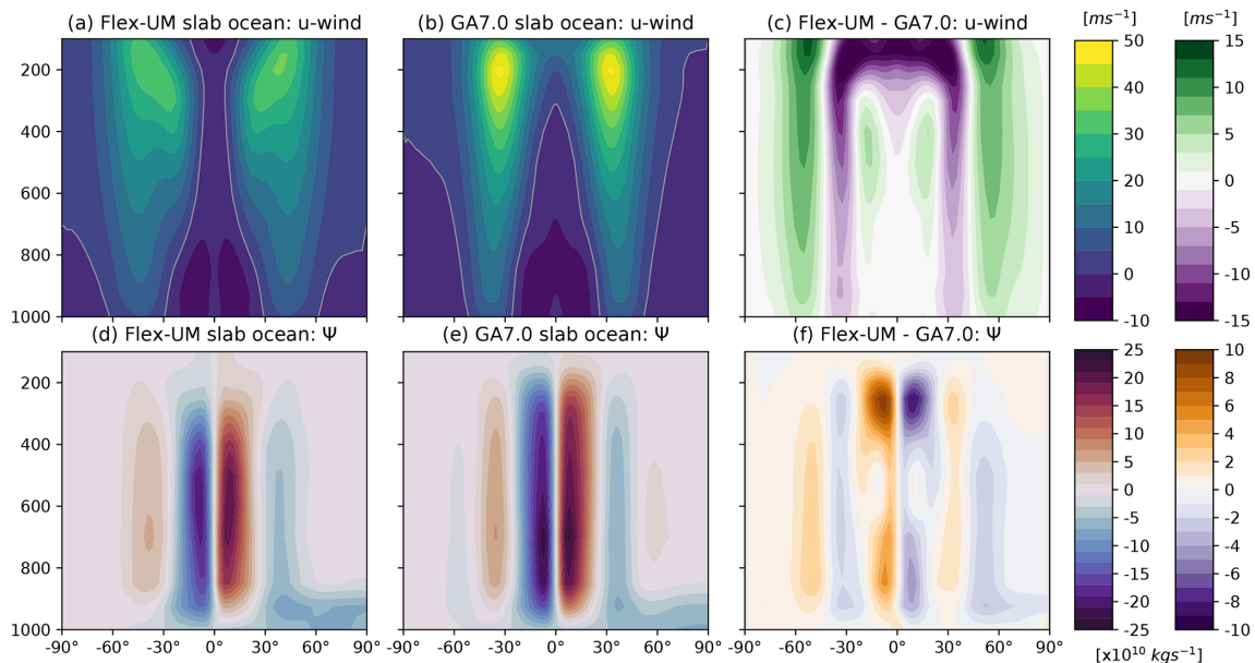
Figure 10. As in Fig. 9 but for zonal-mean zonal wind ( u in \text{m s}^{-1} , a, b, c) and mass stream function ( \psi in \times 10^{10} \text{ kg s}^{-1} , d, e, f).
