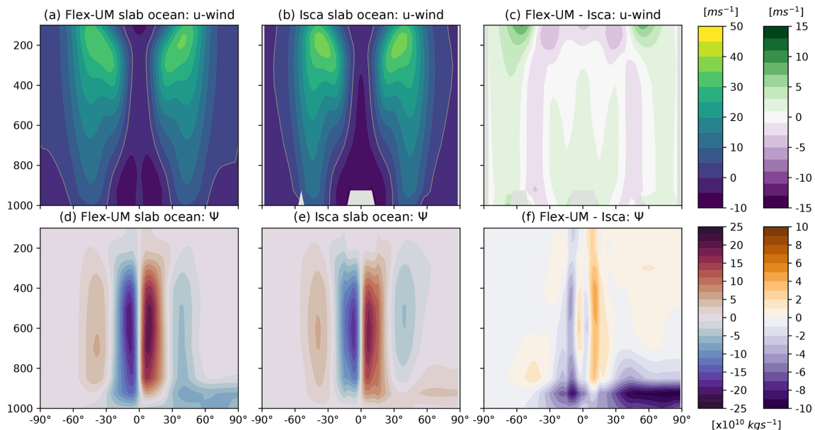
Figure 4. As in Fig. 3 but for zonal-mean zonal wind ( u in \text{m s}^{-1} , a, b, c) and mass stream function ( \psi in \times 10^{10} \text{ kg s}^{-1} , d, e, f).
