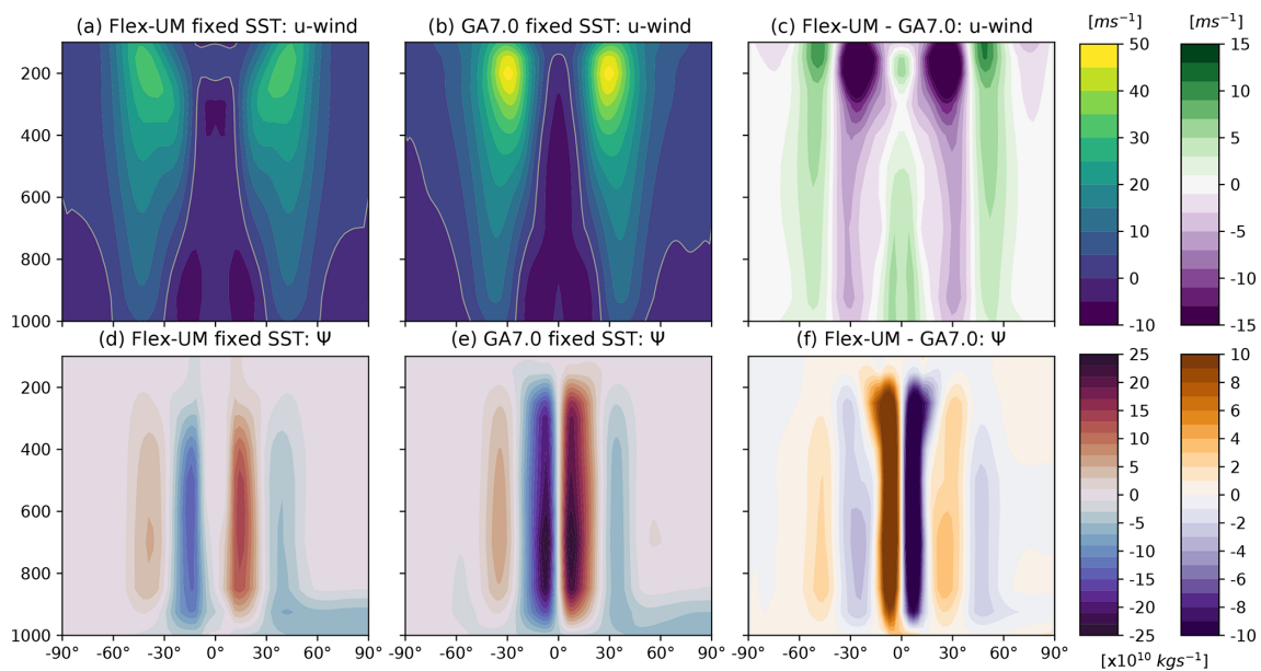
Figure 7. As in Fig. 6 but for zonal-mean zonal wind ( u in \text{m s}^{-1} , a, b, c) and mass stream function ( \psi in \times 10^{10} \text{ kg s}^{-1} , d, e, f).
