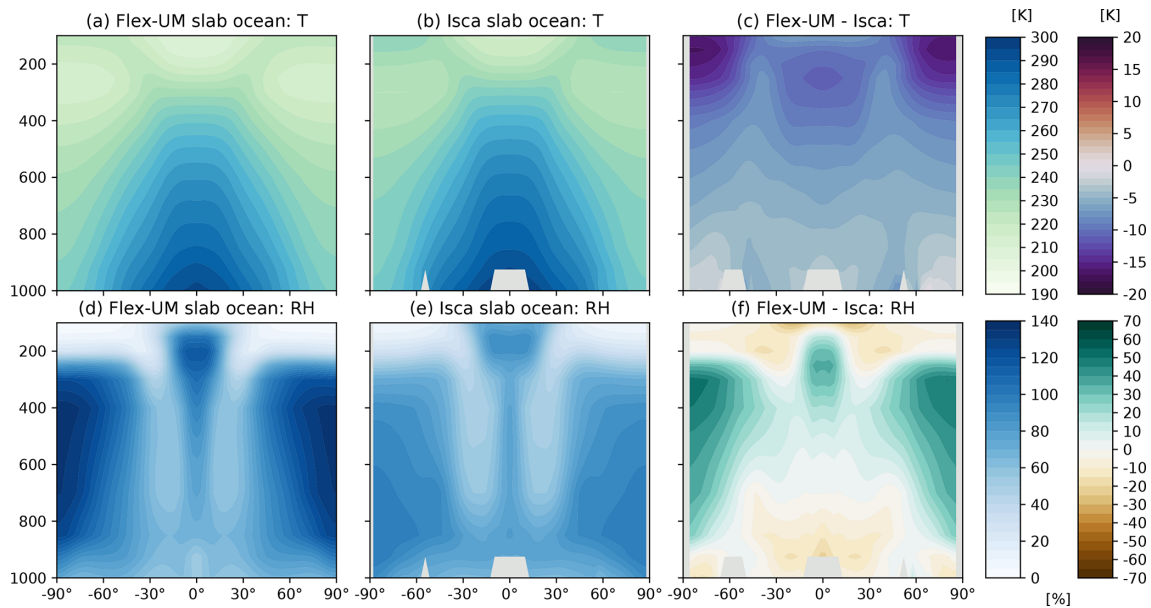
Figure 3. Slab-ocean aqua-planet model climatologies for Flex-UM (a, d) and Isca (b, e) for temperature ( T in K, a, b, c) and relative humidity (RH as a %, d, e, f) on their native model grids. The differences between the models (Flex-UM – Isca) is plotted in panels (c, f) and are interpolated onto the Flex-UM grid. Grey masking near the surface in the middle and right plots (b, e; c, f) occur where the Isca surface pressure is lower than the interpolated model level.
