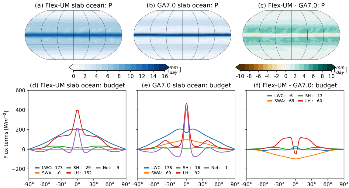
Figure 11. As in Fig. 9 but for precipitation ( P in \text{mm d}^{-1} , a, b, c ) and the atmospheric energy budget ( \text{W m}^{-2} , d, e, f ).
