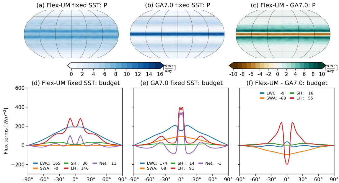
Figure 8. As in Fig. 6 but for precipitation ( P in \text{mm d}^{-1} , a, b, c ) and the atmospheric energy budget ( \text{W m}^{-2} , d, e, f ).
