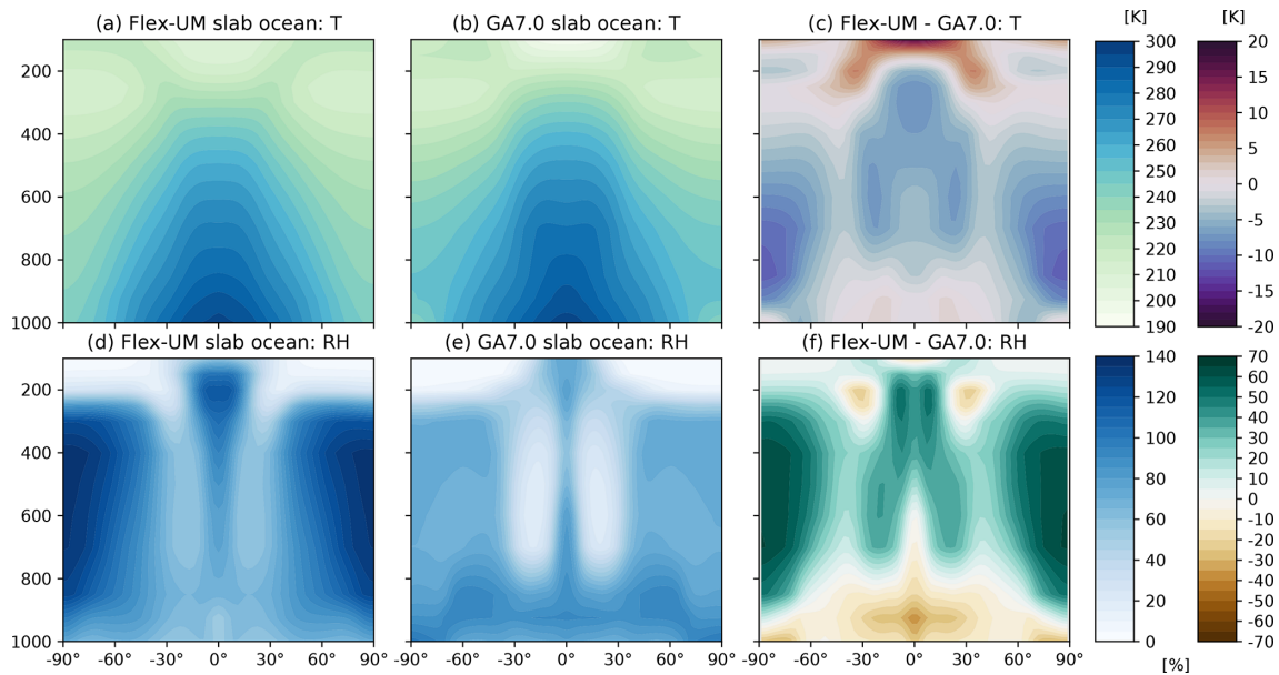
Figure 9. Slab-ocean aqua-planet model climatologies for Flex-UM (a, d) and GA7.0 (b, e) for temperature ( T in K, a, b, c) and relative humidity (RH as a %, d, e, f) on their native model grids. The differences between the models (Flex-UM – GA7.0) are plotted in panels (c, f) and are interpolated onto the Flex-UM grid. Subplots in panels (a) and (d) are identical to those in Fig. 3a and d but are shown here for ease of comparison.
