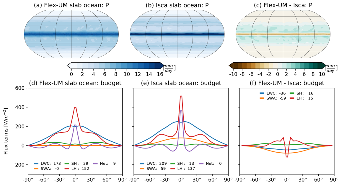
Figure 5. As in Fig. 3 but for precipitation ( P in \text{mm d}^{-1} , a, b, c ) and the atmospheric energy budget ( \text{W m}^{-2} , d, e, f ).
