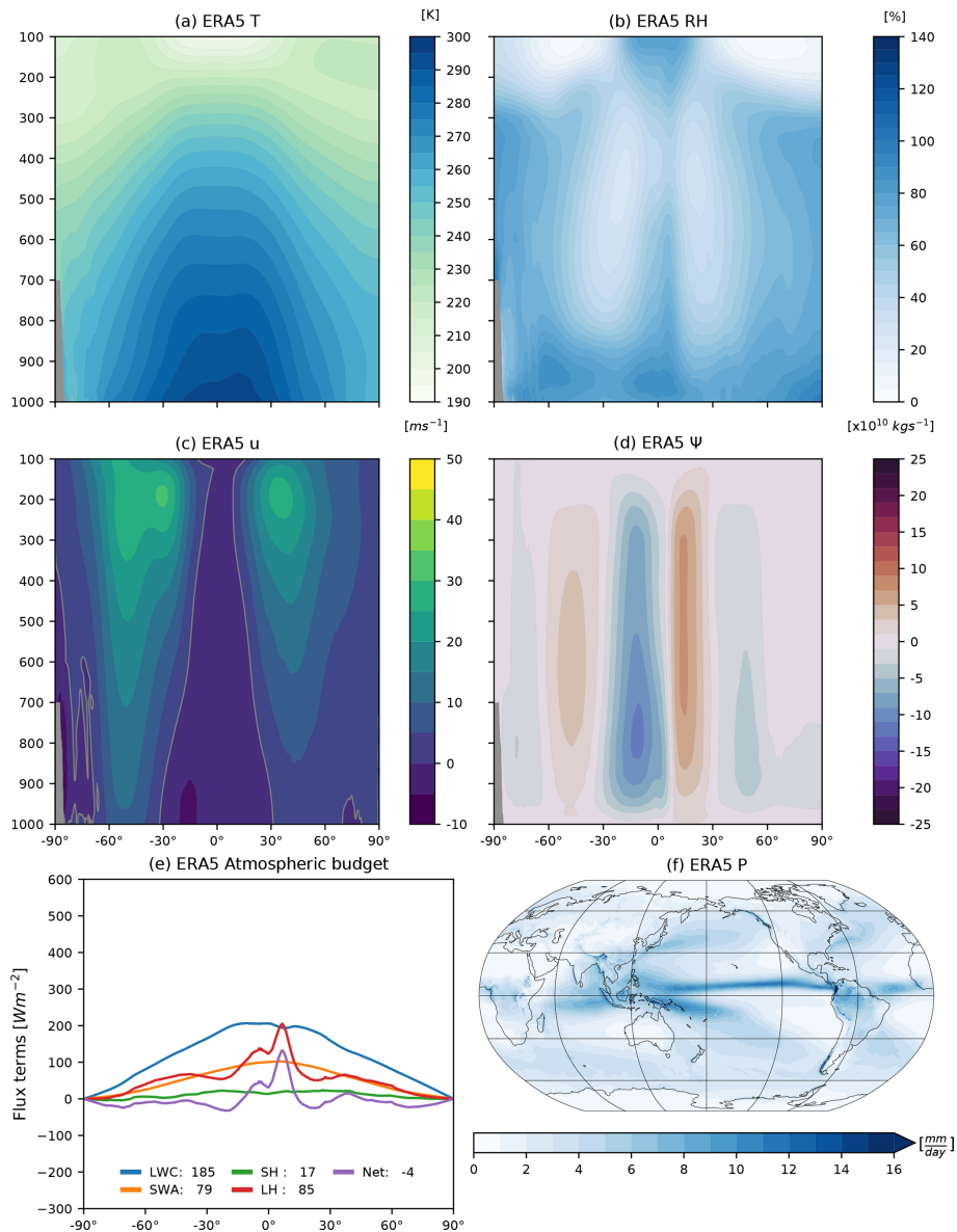
Figure 2. ERA5 reanalysis climatologies for (a) zonal-mean temperature ( T in K), (b) zonal-mean relative humidity (RH as a %), (c) zonal-mean zonal wind ( u in \text{m s}^{-1} ), (d) meridional mass stream function ( \psi in \times 10^{10} \text{ kg s}^{-1} ), (e) atmospheric energy budget (see Eq. 1 in \text{W m}^{-2} ) and (f) precipitation ( P in \text{mm d}^{-1} ). Grey-filled contouring in the SH in subplots in panels (a–d) indicates data masked where the surface pressure is lower than the plotted contour level. The grey line contour in the subplot in panel (e) is the zero wind contour. The legend plotted in the subplot in panel (e) indicates the area-weighted global averages.
