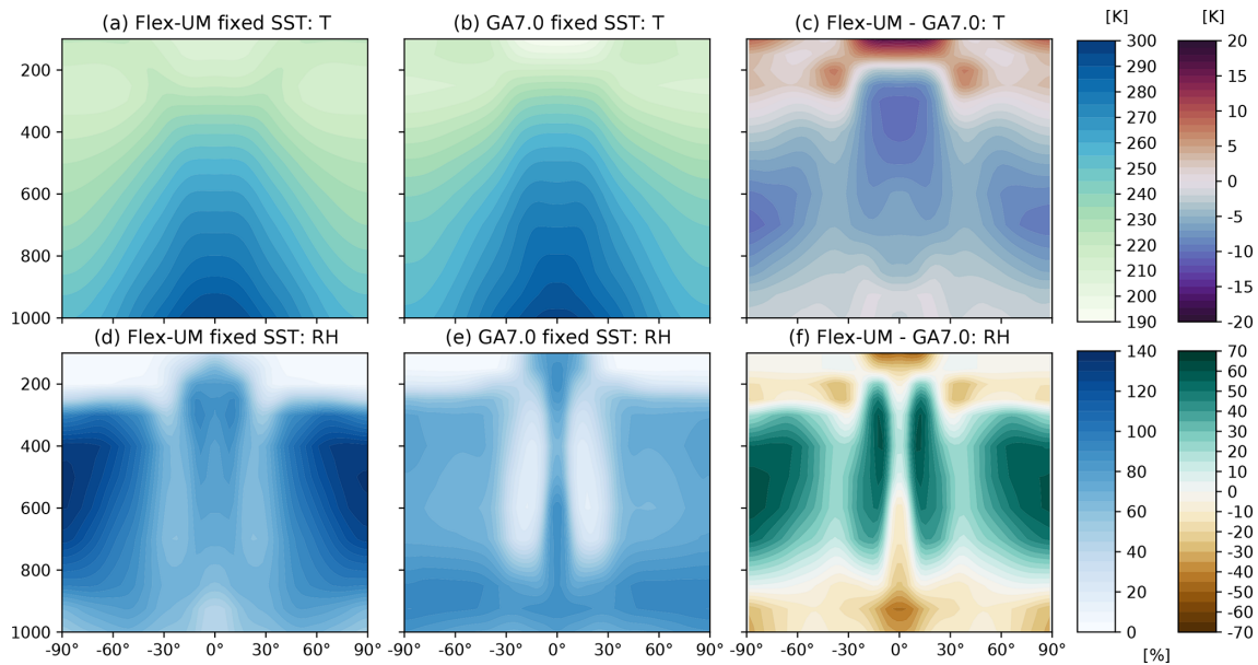
Figure 6. Fixed-SST aqua-planet model climatologies for Flex-UM (a, d) and GA7.0 (b, e) for temperature ( T in K, a, b, c) and relative humidity (RH as a %, d, e, f) on their native model grids. The differences between the models (Flex-UM – GA7.0) are plotted in panels (c, f) and are interpolated onto the Flex-UM grid.
