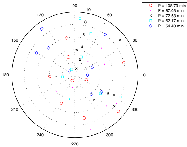
Fig. 5. The phases for each Fourier component over the 9 days of observation after filtering the signals to contain only periods in the range P = 50\text{--}150 min. Phases are given in degrees and the points for each day lie on an annulus at r = 1, 2, \dots, 9 , corresponding to the day number (i.e. 1 for 06 April 2003, 2 for 07 April, etc.).
