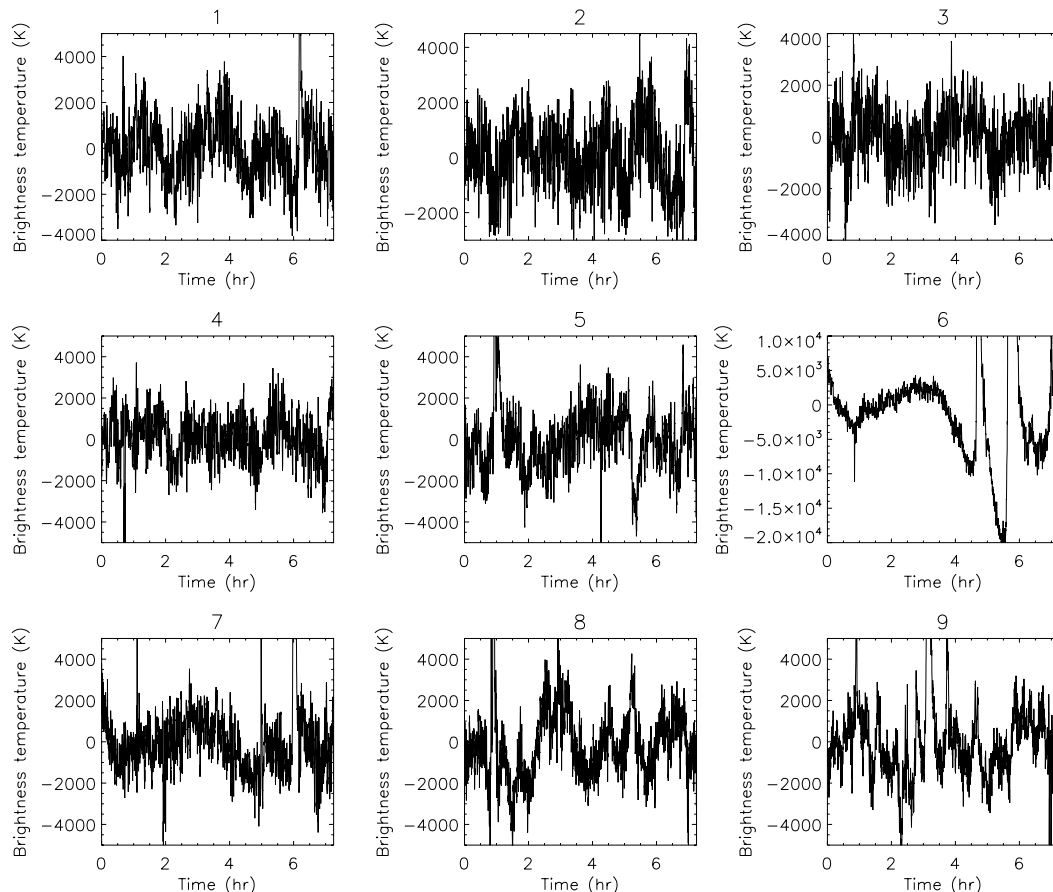
Fig. 2. Time series of microwave intensity generated from sequences of images of AR 10330 obtained with NoRH. The signals have been detrended with a 4th order polynomial. The title for each signal gives the day number in the sequence of the 9 days of observation.
