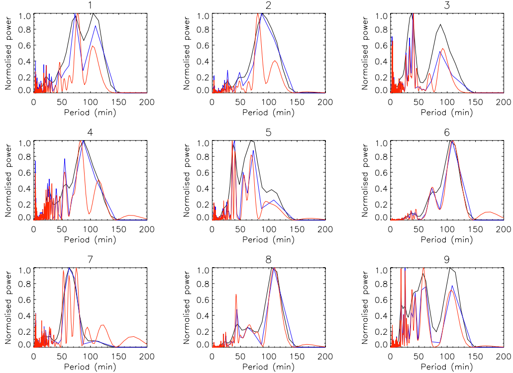
Fig. 3. Normalised power spectra obtained for each of the 9 detrended signals, using the global wavelet (black), Lomb-Scargle periodogram (red) and FFT (blue). Each spectrum has been normalised to its maximum amplitude. As in Fig. 2, the title for each signal gives its position in the sequence of the 9 days of observation.
