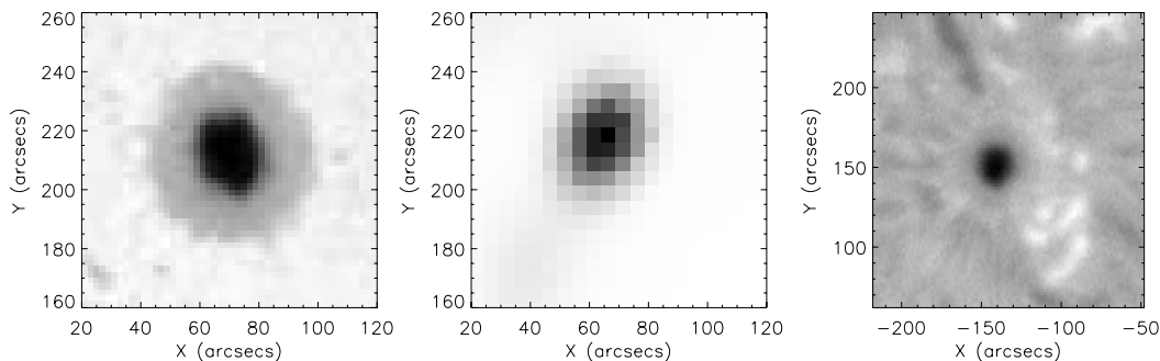
Fig. 1. Images of AR 10330 in white light ( left ) and microwave (17 GHz, centre ) taken at 23:59 UT on 09 April 2003 and in H\alpha ( right ), taken at 01:03 UT on 10 April 2003.
