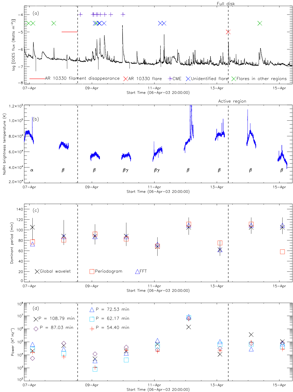
Fig. 4. a) The GOES X-ray flux during the period 06 April 2003 20:00–15 April 2003 10:00, showing events that occurred in AR 10330 and elsewhere. b) The original time series obtained from NoRH images. The Mt. Wilson classification for AR 10330 is also shown. c) The dominant periods in the range P = 50 – 120 min, obtained with all three of the methods for computing the power spectrum. The error bars on the global wavelet spectrum were obtained using the full width at half maximum (FWHM) of the corresponding spectral peak. d) The power for each Fourier component in the range P = 50 – 150 min for each day. In panels c) and d) , the points for each day have been plotted at the midpoint of each signal.
