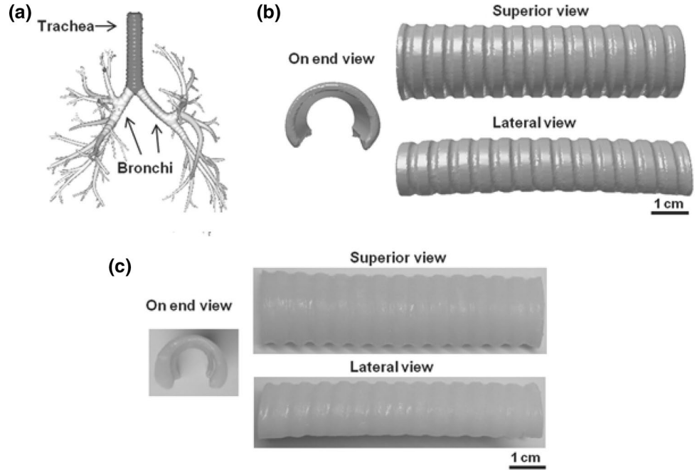
Fig. 6 Illustration of the process of producing a stent. a Imaging stage by MRI. b Prepare digital model (CAD). c Final stent structure in the original state. Reproduced from ref [88], with permission from John Wiley and Sons
