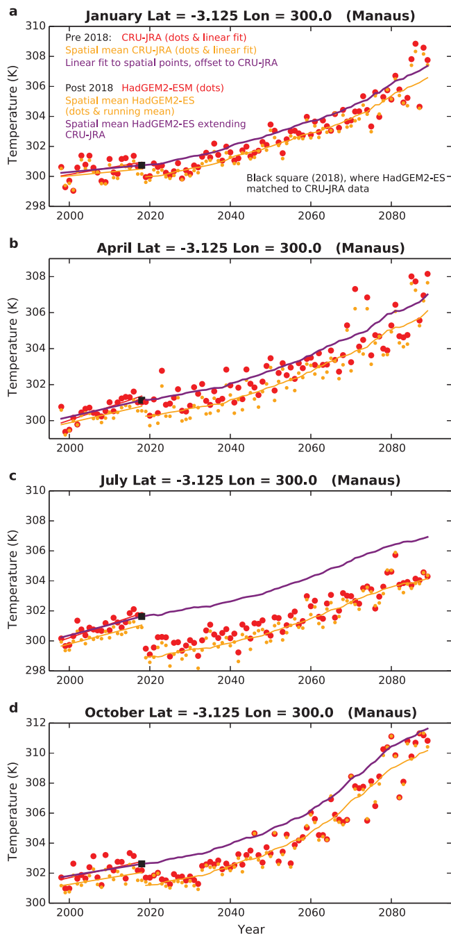
FIGURE 1 Bias-correction method. Monthly mean temperature (shown for January, April, July and October) for the gridbox containing the city of Manaus. Curves in the period to year 2018 are based on the data-led CRU-JRA climatology, whereas after that year, the diagram uses projections with the HadGEM2-ES ESM. Pre-2018, the red dots are for 21 years (1998–2018) at the individual gridbox, with a linear fit shown for information. Yellow dots are spatial means of the monthly values, including nearby points ( \pm 3^\circ latitudinally, \pm 2^\circ longitudinally), and shown with their linear fit (also yellow). The latter linear fit, so including the averaging of neighbouring points, we regard as a better estimate of trends by removing local fluctuations. This trend (yellow line) is then offset, so that its mean value equals that of the red dots for the single gridbox. We show this final linear fit in purple, and regard it as our estimate of background trends for the Manaus gridbox, pre-2018. For
