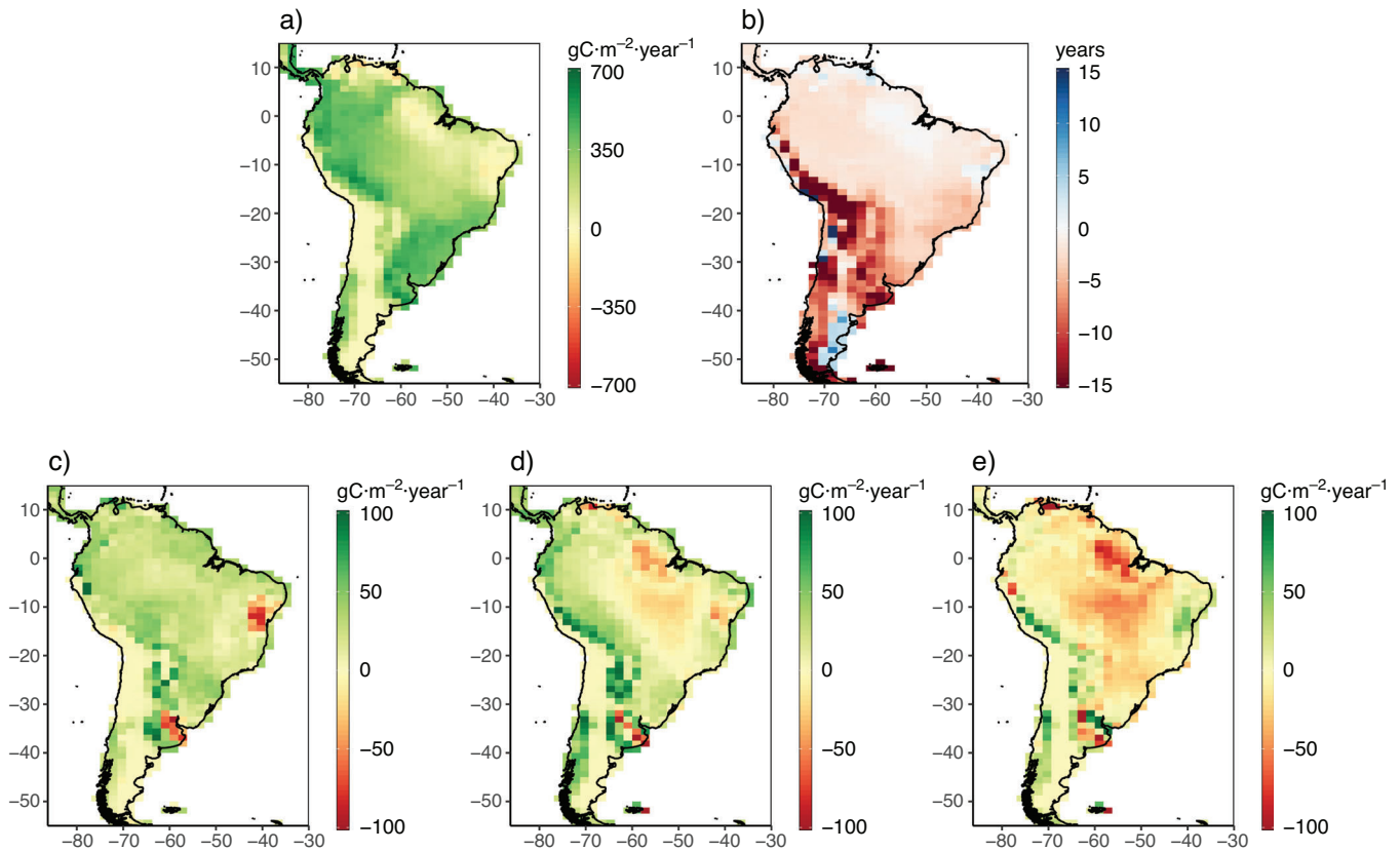
FIGURE 4 Attributes of the South American terrestrial carbon cycle fluxes. Panel (a) is the change in NPP (period 2069–2089 minus 1999–2019) and (b) is the change in soil carbon residence time over the same timeframe. Panel (c) is NBP for period 1999–2019 and (d) is NBP for future period 2069–2089. Panel (e) is the projected NBP changes (middle minus left, lower plots). Negative values of NBP correspond to carbon released from the vegetation to the atmosphere. Values are gridbox means and are therefore calculated from the areal weighting based on PFT fractions
