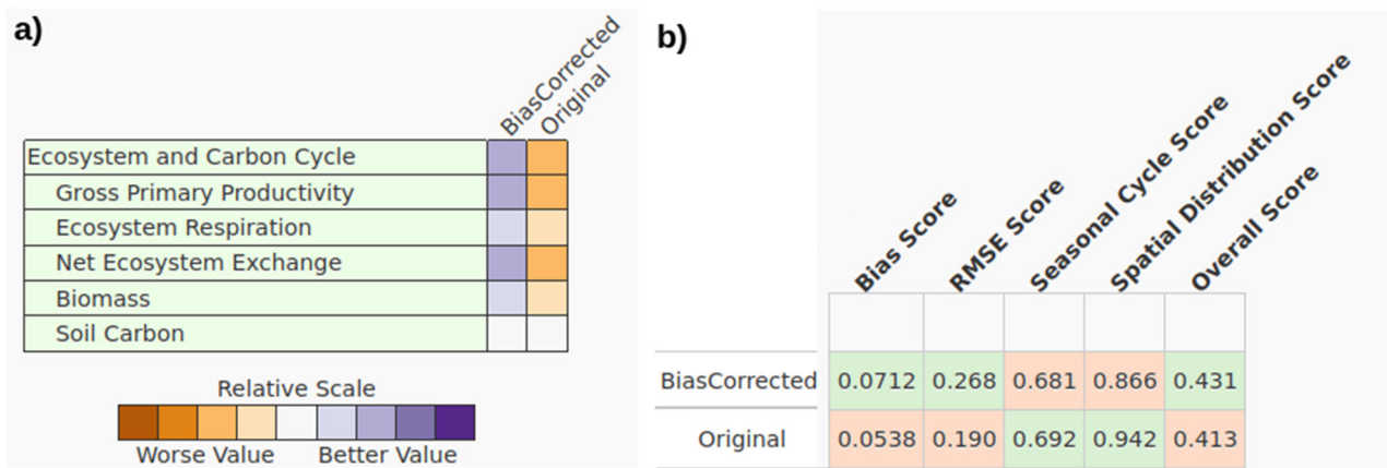
FIGURE 7 ILAMB statistics. (a) Comparison of the relative performance of JULES-ES forced by bias-corrected climate data from HadGEM2-ES (marked here as ‘BiasCorrected’) and with mean biases re-added to the climate forcing data (‘Original’). Calculations are for South America, obtained by placing JULES-ES projections in the International Land Model Benchmarking system (ILAMB) framework and selecting the comparison against the GBAF/FLUXCOM gridded data. As the DGVM data examined are for the recent historical period, the climate forcing data used in our simulations that we describe as bias-corrected are that of the CRU-JRA data set. (b) Statistics for the performance of both sets of simulations at projecting ecosystem respiration (Collier et al., 2018 for details). It is the overall bias score in panel (a) that determines the colour coding for ecosystem respiration in panel (a)
