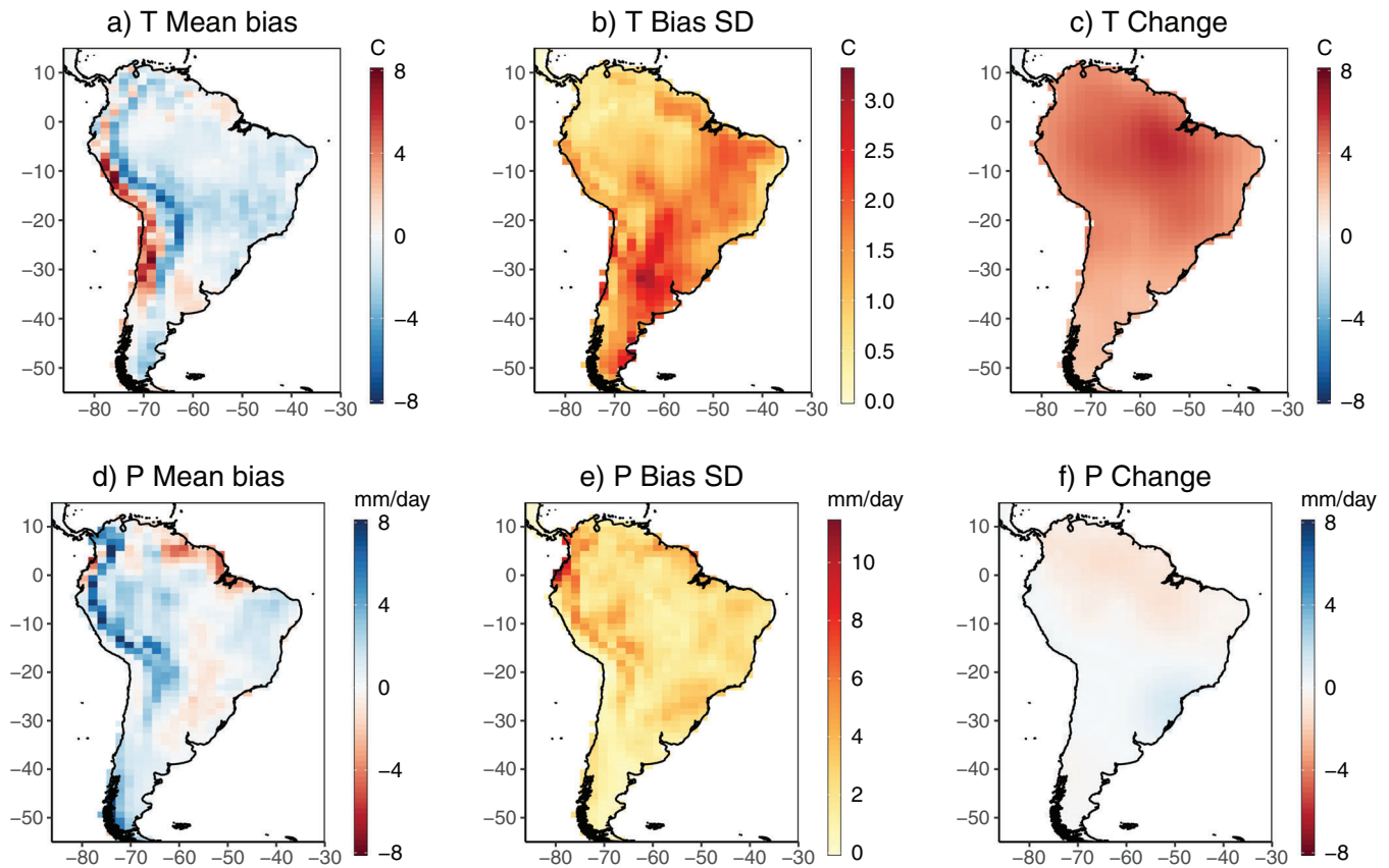
FIGURE 2 HadGEM2-ES biases and projections. Comparison of the magnitudes of bias correction versus climate change for near-surface temperature, T (first row), and for precipitation, P (second row). First column is annual mean offsets, as the average of the monthly bias corrections, shown as direct HadGEM2-ES diagnostics (i.e. without bias corrections) minus climatology based on CRU–JRA re-analysis values. The second column also relates to bias magnitude, and shows the standard deviations of the 12 bias correction values for each month and for each location. The third column presents the amount of annual mean climate change (future minus recent) between the recent past (mean of years 1999–2019) and towards the end of the 21st Century (2069–2089). We keep the colour bar ranges identical between the first and third columns for ease of comparison. Panels c and f are repeated in Figure S2 with colour bars more tightly aligned to the range of projected climate change
