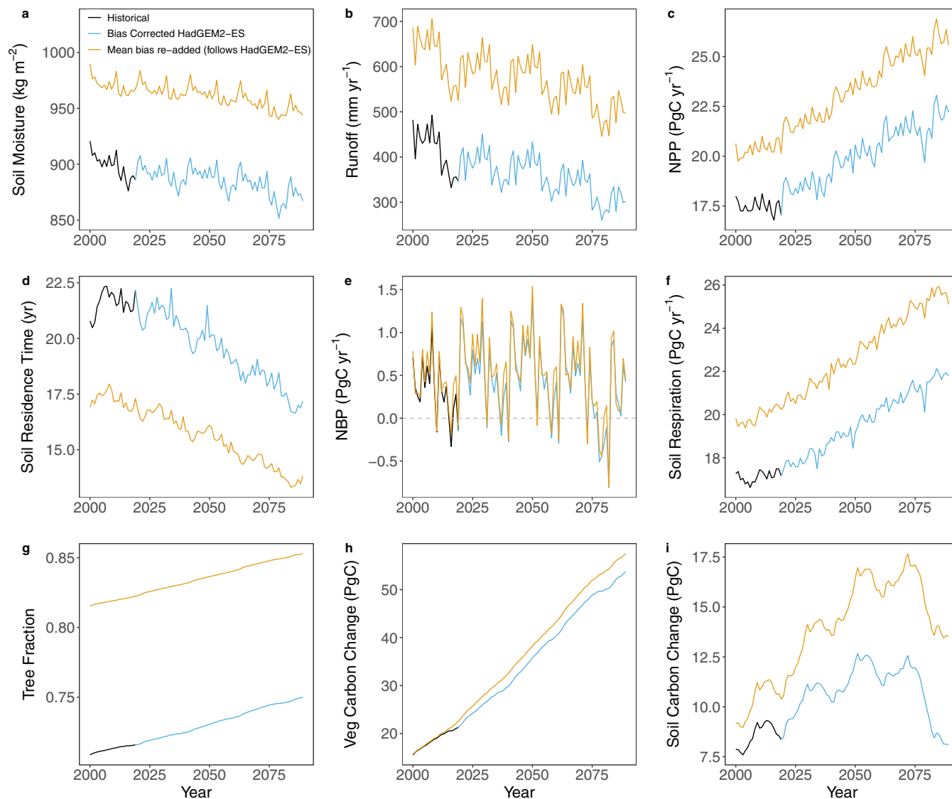
FIGURE 6 Time series of South American land changes for the RCP8.5 greenhouse gas scenario. Time-evolving annual values of spatially averaged attributes of the land for South America (areal averages across same domain as the maps of Figures 2–5). Spatial means are for the hydrological variables of (a) soil moisture and (b) runoff, and of carbon-related variables of (c) net primary productivity, (d) soil carbon residence time, (e) net biophysical production, (f) soil respiration, (g) tree fraction, (h) vegetation carbon and (i) soil carbon. The black and blue curves are simulated land changes when forced with historical measurement-based data from the CRU–JRA data set, followed by our bias-corrected version of the HadGEM2-ES ESM. The orange curves are for forcing where the mean monthly ESM bias corrections are added back on to the historical and corrected future data. This approach to reintroducing biases ensures that the emphasis is on the mean offset errors, while retaining similarities for the higher frequency variations contained in the drivers needed by the JULES DGVM. All calculations are from year 1901, but to aid focus on the decades ahead, presented are years from 1990 onwards only. Panels (h) and (i) are anomalies, relative to period 1901–1930
