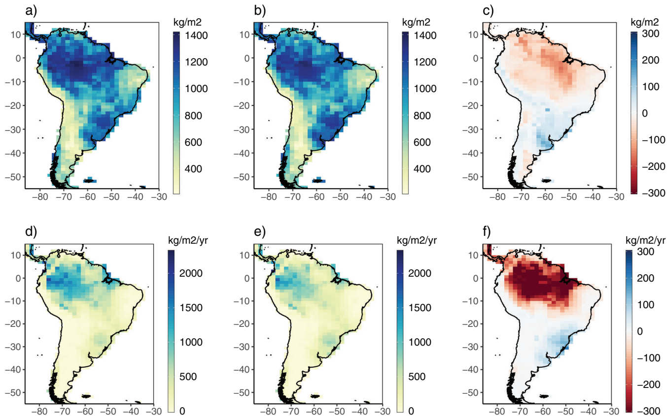
FIGURE 3 Hydrological variables. Spatial hydrological variables, and their changes, of soil moisture (top row) and surface runoff (bottom row). The left column is annual mean values, averaged for period 1999–2019, and the middle column is values for future period 2069–2089. The right column is the changes (future climate minus recent past, i.e. middle minus left columns)
