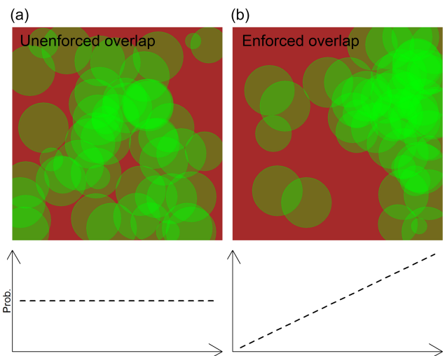
Figure 2. Visual representation of the effects of enforcing overlap within a ( 100\text{ m} \times 100\text{ m} ) TROBIT site with a given canopy area index (CAI). (a) Overlap is not enforced, and individual crowns follow a uniform random distribution. (b) Overlap is enforced by linearly increasing the probability of a canopy being located more on one side of the site (i.e. here the right side of the site) than the other. This results in tree canopies “overlapping” to a greater extent, which affects how accurately CAI represents actual canopy cover.
