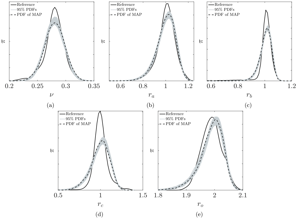
Figure 5: Results for the univariate marginal PDFs. The reference results are the results of the deterministic identifications (based on 2400 observations per parameter). The grey lines are PDFs associated with the 95% credible region (i.e. the region that one believes 95% it contains true value of some parameter [72]). The dashed line is the PDF associated with the MAP estimate. This graphical test [9] shows a reasonable agreement between the simulated curves and the ones based on observations.
