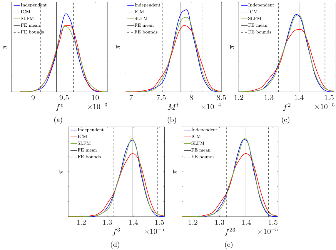
Figure 17: The PDFs for the reaction forces and moments as well as the FE values. For all the cases the reference values as well as their bounds are inside the prediction PDFs. Except for f^e and M^t the corresponding mean values of the reaction forces and moments are located at the peak of the PDFs. The independent fields yields narrowest PDFs (i.e. more certainty about the estimated values).
