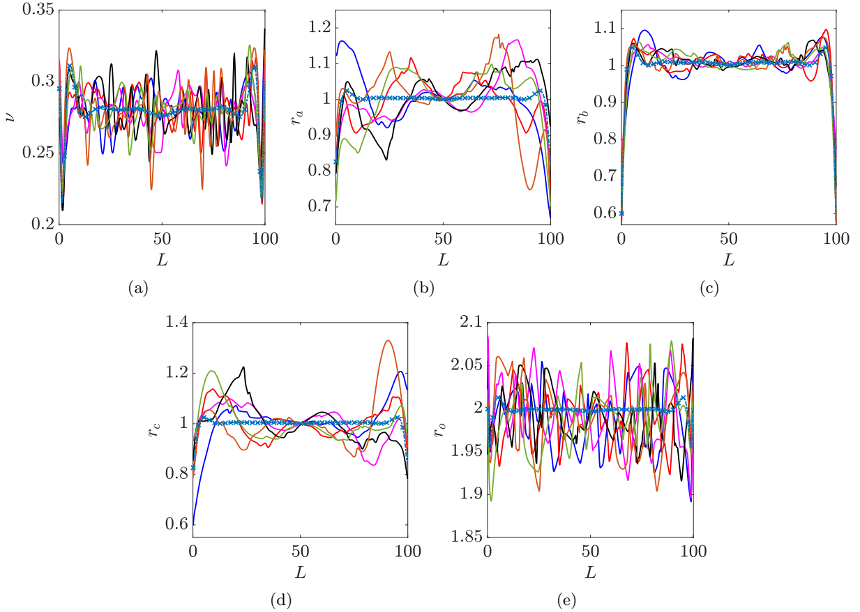
Figure 4: Deterministically identified input fields for the beam representations of the six struts and (for comparison purposes) the homogeneous strut. The colors distinguish the different struts and the triangles are for the homogeneous strut.
