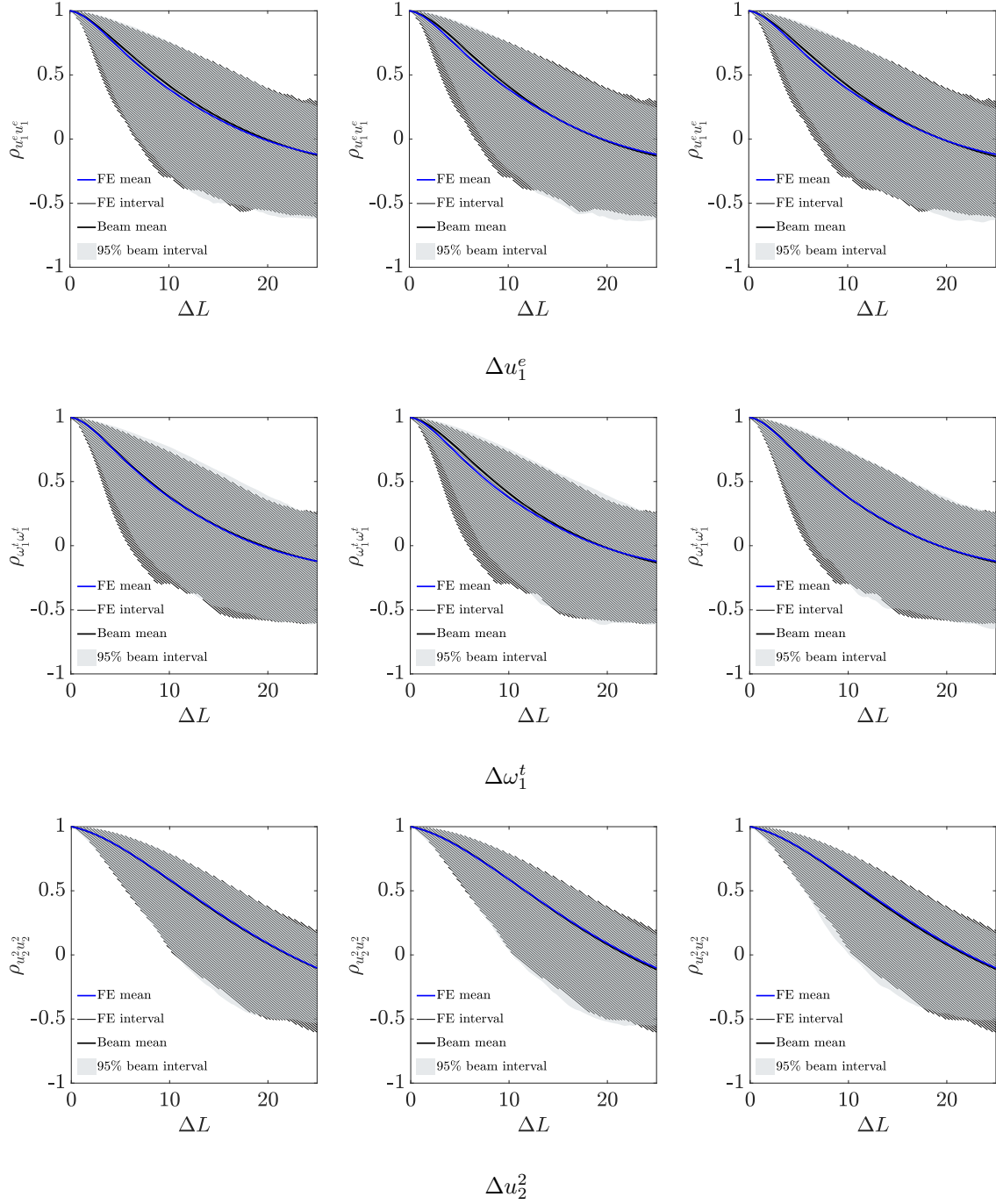
Figure 18: Prediction and observation intervals for the autocorrelation functions of both the FE and beam simulations alongside the means. Left column: independent fields, center column: ICM and right column: SLFM. All predictions and observations are similar. However, based on the means for \Delta u_1^e and \Delta \omega_1^t , it is clear that the independent fields and SLFM are more accurate than the ICM approach. The ICM method yields wider prediction intervals, so that, with the exception for \Delta u_1^e and \Delta \omega_1^t , a larger portion of the FE results remains within its prediction intervals. Note that the numerical estimate for the autocorrelation function provides a reasonable estimate for \Delta L \leq \frac{L}{4} [73]. Furthermore, a good estimate of the autocorrelation function needs at least 50 sample points of a realization from a random process/field [73].
