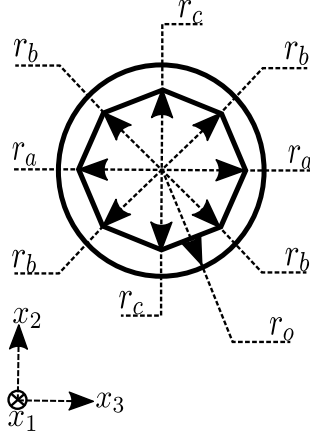
Figure 2: The hollow cross section of each beam element.
