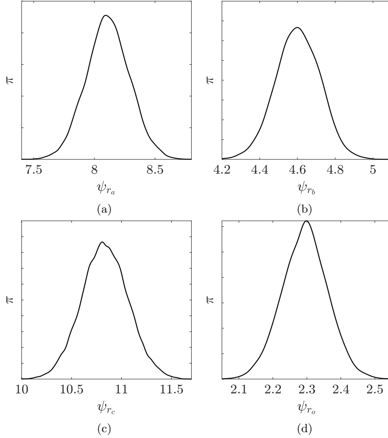
Figure 7: Independent fields: marginal posteriors for the identified parameters. The marginal posterior distributions are obtained using the histogram of samples simulated by the Metropolis algorithm with an adaptive proposal distribution from Eq. (44).
