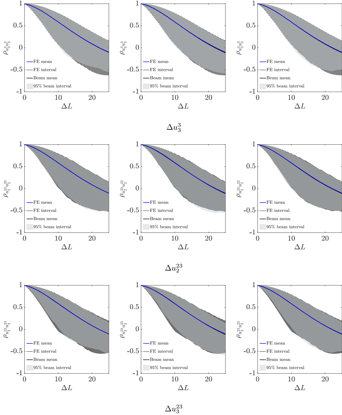
Continued Figure 18: Prediction and observation intervals for the autocorrelation functions of both the FE and beam simulations alongside the means. Left column: independent fields, center column: ICM and right column: SLFM. All predictions and observations are similar. However, based on the means for \Delta u_1^e and \Delta \omega_1^t , it is clear that the independent fields and SLFM are more accurate than the ICM approach. The ICM method yields wider prediction intervals, so that, with the exception for \Delta u_1^e and \Delta \omega_1^t , a larger portion of the FE results remains within its prediction intervals. Note that the numerical estimate for the autocorrelation function provides a reasonable estimate for \Delta L \leq \frac{L}{4} [73]. Furthermore, a good estimate of the autocorrelation function needs at least 50 sample points of a realization from a random process/field [73].
