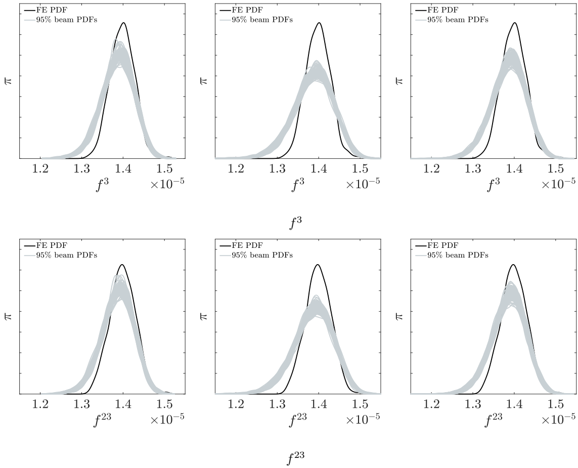
Continued Figure 16: The FE PDFs (solid black lines) as well as the PDFs associated with 95% credible region (gray lines) for the reaction forces and moments of the different applied deformation modes (indicated by the superscript). Left column: independent fields, center column: ICM and right column: SLFM. The independent fields and the SLFM methods are more accurate than the ICM method. However, the MAP estimates of all three approaches are sufficiently close to the peaks of the FE PDFs. Furthermore, the PDFs associated with the ICM method are the widest.
