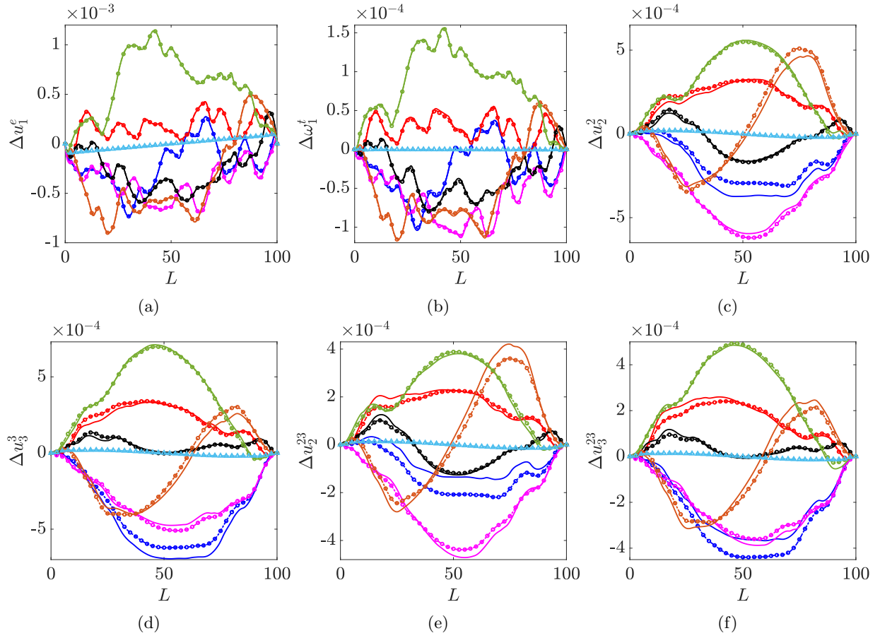
Figure 3: The final differences between the relative center line displacements and rotations of the FE simulations (solid lines) and the beam simulations (dashed lines with circles) for the six struts and (for comparison purposes) a perfectly homogeneous strut (homogeneous strut: triangles with dashed lines for the beam simulations, dotted lines for the FE simulations). The results are presented relative to those of a linear interpolation (top left and top center diagrams) or cubic interpolation (top right and bottom diagrams), so that the fluctuation are better visible. The colors denote the different struts. The subscripts refer to the three directions and the superscripts refer to the five applied deformation modes ( e : axial elongation, t : torsion, 2: nodes at one end displaced in the x_2 -direction, 3: nodes at one end displaced in the x_3 -direction, and 23: nodes at one end simultaneously displaced in the x_2 -direction and x_3 -direction).
