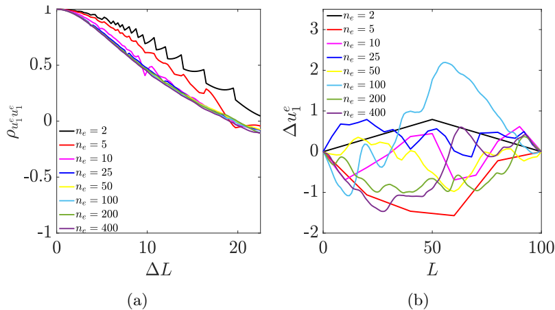
Figure B.20: Mesh convergence analyses for the intrinsic coregionalization model with axial elongation as the employed deformation mode. Left: the predicted autocorrelation mean for the predicted relative center line displacements in axial direction ( \Delta u_1^e ), for eight different discretizations (with 2, 5, 10, 25, 50, 100, 200 and 400 elements). Each curve is the mean of autocorrelation predictions for each particular discretization. Right: a single field of relative center line displacements in axial direction as predicted by the eight discretizations.
