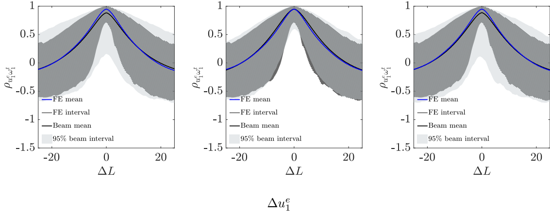
Figure 19: Prediction and observation intervals for the cross-correlation functions of both the FE and beam simulations alongside the means. Left: independent fields, center: ICM and right: SLFM. Only the cross-correlation function between \Delta u_1^e and \Delta \omega_1^t is presented as the other cross-correlations are the same for the three approaches. The envelopes of both the independent fields and the SLFM methods include the entire FE intervals. On the other hand, the mean cross-correlation of the ICM method is more accurate than those of both the independent fields and SLFM methods. Although the prediction bounds for both the independent fields approach and the SLFM approach look similar, it is clear that the SLFM approach predicts wider intervals. Furthermore, the mean of the SLFM approach is closer to the observation mean than that of the independent fields. The similar behavior of both the SLFM and the independent fields approaches can be due to the fact that the intercorrelation between the parameter fields may not be very strong. Note that in the proposed SLFM model, the intercorrelations between the parameter fields are modeled by a second latent random field that is linearly combined with the independent fields by the \underline{a}^5 vector. If the components of this vector (linear combination coefficients) are small, the result will be similar to the case of the independent fields. Note that the numerical estimate for the cross-correlation function provides a reasonable estimate for \Delta L \leq \frac{L}{4} [73]. Furthermore, a good estimate of the cross-correlation function needs at least 50 sample points of a realization from a random process/field [73].
