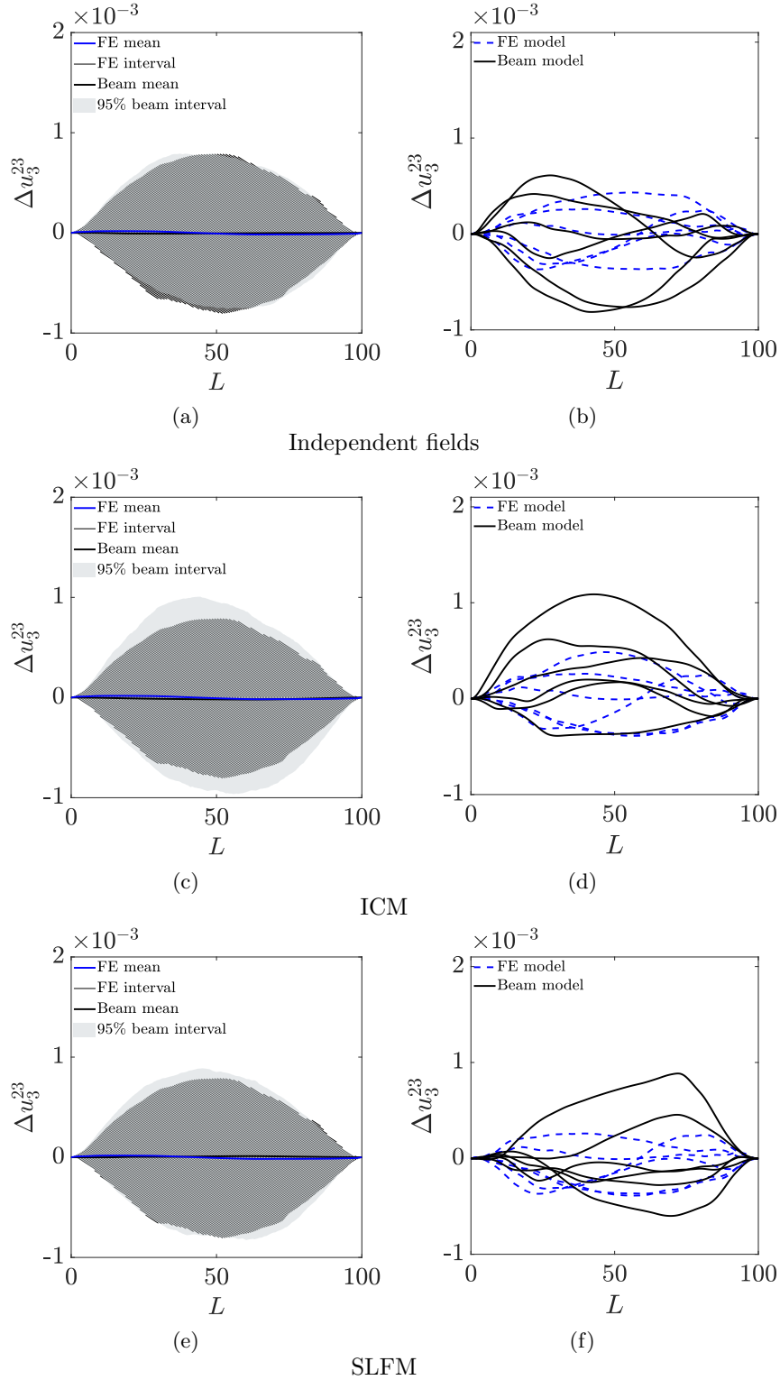
Figure 15: Bending applied in both x_2 and x_3 simultaneously, lateral displacement in x_3 : prediction intervals and observation intervals when the parameter fields are modeled as (a) independent random fields, (c) correlated random fields using the ICM approach and (e) correlated random fields using the SLFM approach. A few sample responses of the FE models and of the beam models are shown in the diagrams on the right. The prediction intervals of both the ICM approach and the SLFM approach encompass all the FE results. However, the ICM approach yields a wider prediction interval than the SLFM approach. Note that the presented responses are relative to that of the homogeneous case.
