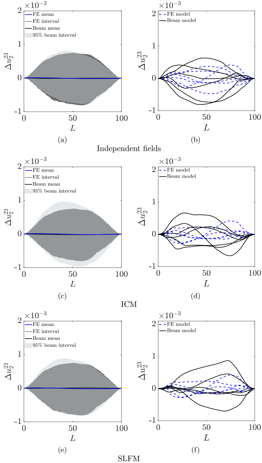
Figure 14: Bending applied in both x_2 and x_3 simultaneously, lateral displacement in x_2 : prediction intervals and observation intervals when the parameter fields are modeled as (a) independent random fields, (c) correlated random fields using the ICM approach and (e) correlated random fields using the SLFM approach. A few sample responses of the FE models and of the beam models are shown in the diagrams on the right. The prediction intervals of both the ICM approach and the SLFM approach encompass all the FE results. However, the ICM approach yields a wider prediction interval than the SLFM approach. Note that the presented responses are relative to that of the homogeneous case.
