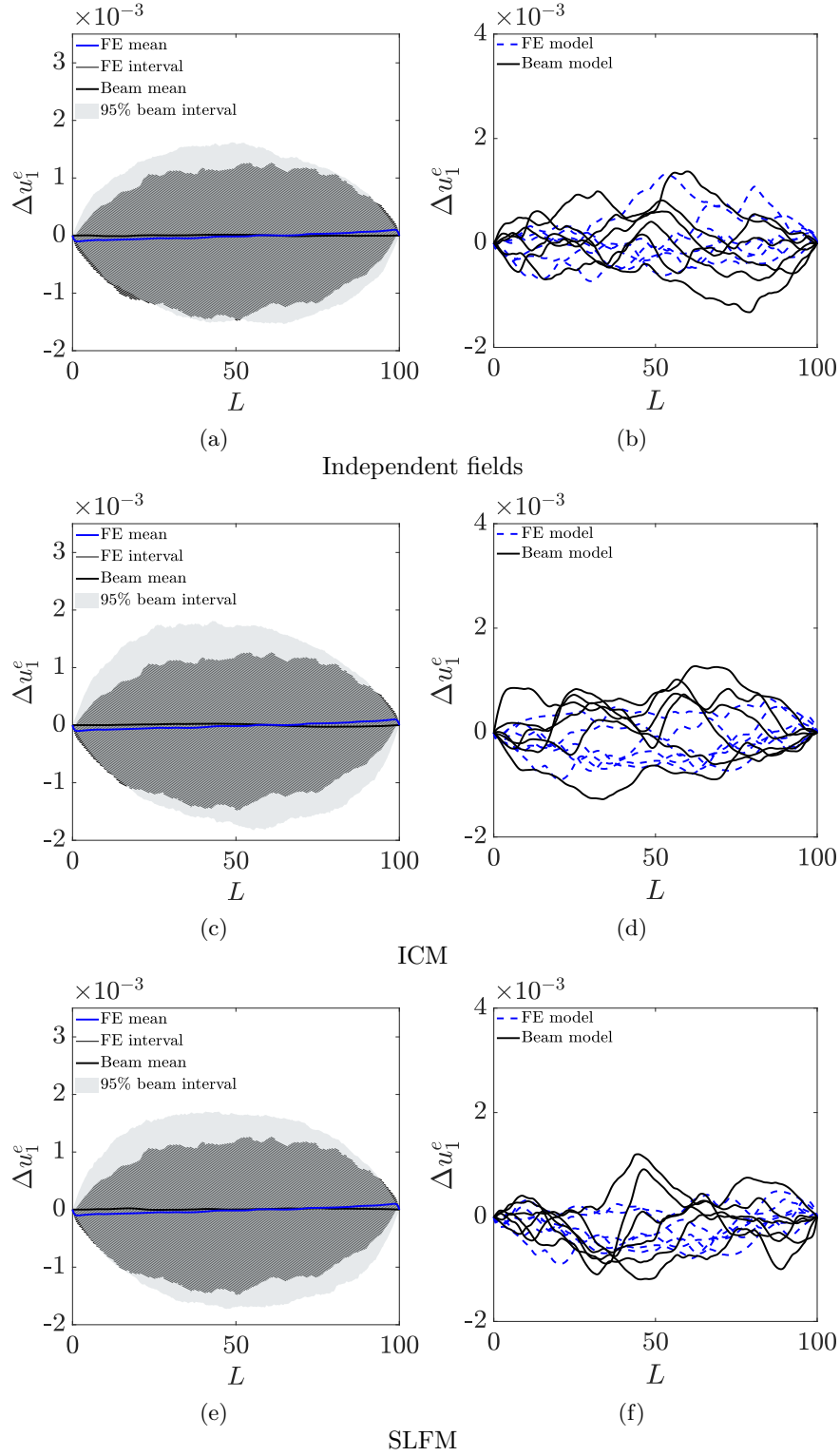
Figure 10: Elongation: prediction intervals and observation intervals when the parameter fields are modeled as (a) independent random fields, (c) correlated random fields using the ICM approach and (e) correlated random fields using the SLFM approach. (b), (d) and (f) show samples of the FE model response and of the beam model response. One can see that in both the ICM and the SLFM approaches the observations at all locations are inside the prediction intervals. However, in the case of independent fields the observations bounds around x_1 = 15 are outside the predictions intervals. Furthermore, comparing (a), (c) and (e) indicates that the ICM approach has the widest prediction interval and the independent fields approach has the narrowest prediction interval. Although the difference between the ICM approach and the SLFM approach for this test is not large. Moreover, the sample curves in (b), (d) and (f) show that the beam responses are similar to the FE responses. Note that the presented responses are relative to that of the homogeneous case.
