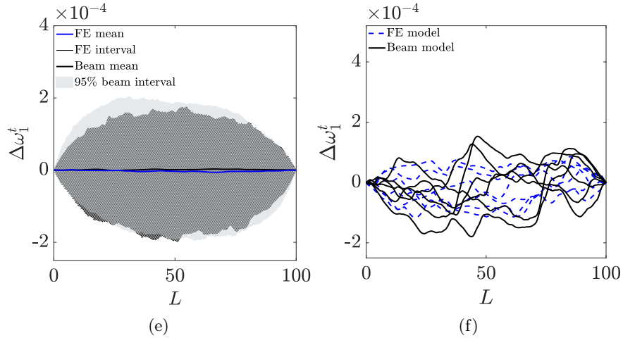
Figure 11: Torsion: prediction intervals and observation intervals when the parameter fields are modeled as (a) independent random fields, (c) correlated random fields using the ICM approach and (e) correlated random fields using the SLFM approach. A few sample responses of the FE models and of the beam models are shown in the diagrams on the right. The FE responses only remain the prediction interval of the ICM approach. Moreover, similar to axial elongation, the ICM approach has the widest prediction interval whereas the independent fields approach has the narrowest prediction interval. Note that the presented responses are relative to that of the homogeneous case.
