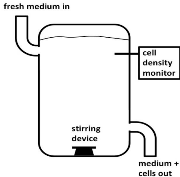
Figure 1: Our idealized one-liter chemostat. Cell density is continuously monitored and kept at a constant low level (say 106/ml) such that no supplied nutrient is limiting. Fresh medium is pumped in, and medium containing cells is pumped out.
