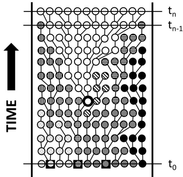
Figure 2: Fixation of sub-clones in our idealized chemostat. A sub-clone, like a clone or a clade, is defined as any ancestor plus all of its descendants, living or dead (expelled from the chemostat or extinct). Designation of cells as ancestors and thus as founders of sub-clones is arbitrary. A sub-clone is “dead” if none of its descendants are living in the chemostat. In our model, the number of living sub-clones at t_n is defined as the number having distinct common ancestors at t_0 , so this would be one for t_n as shown but would be three if t_n were one “generation” earlier, at t_{n-1} . Founder (ancestor) of sub-clone present at t_n is indicated by a circle and founders (ancestors) of sub-clones present at t_{n-1} are indicated by squares. That at some time t_n sufficiently distant from t_0 , the number of living sub-clones will be one is a consequence of both neutral and coalescent theory (Kingman 2000). If a mutation favouring differential growth (increase in number of organisms) of a sub-clone (indicated as changes in pattern of fill in this figure) occurs, then the probability of fixation increases and the number of generations between t_0 and t_n will likely be reduced.
