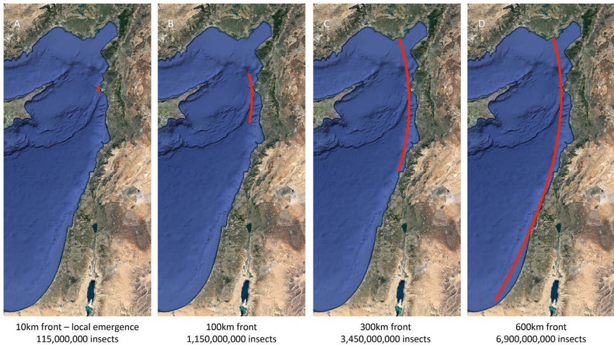
Figure S2. Lengths of proposed insect migration fronts leaving the Middle Eastern coastline and crossing the Mediterranean. Estimates of the number of insects leaving the Middle East under each scenario are given.
