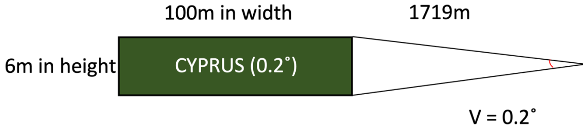
Figure S1. Viewing angles and distance at which Cyprus first exceeds 0.2° in an insect's field of view when approaching from the east. See main text for details. V = visual angle.
