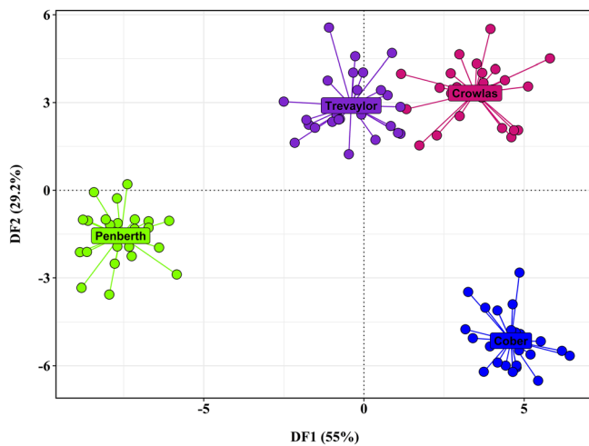
FIGURE 2 A priori discriminant analysis of principal components (DAPC) of trout genotypes from rivers flowing into Mount's Bay, Cornwall. Individuals are represented by individual points, with centroids for each river labelled. Discriminant function 1 (DF1) is represented by the x axis, and discriminant function 2 (DF2) by the y-axis
