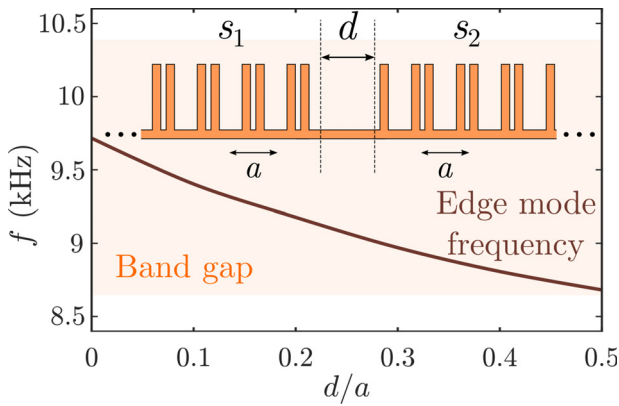
FIG. 1. Tunable edge mode by dislocation: Frequency domain FEM simulations showing change in edge mode frequency with dislocation length d between two SSH chains s_1 and s_2 , with unit cell width a . We supplement this with dynamic tunability through the use of a photo-responsive material.
