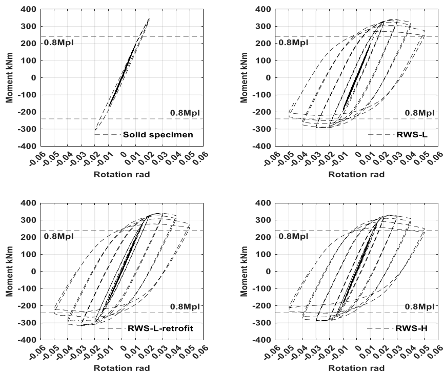
Figure 4. Hysteretic curve of the specimens.
