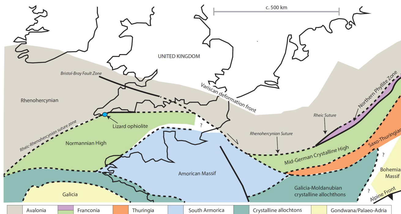
Figure 1. Simplified tectonic map of Europe, after Franke et al. (2017).
