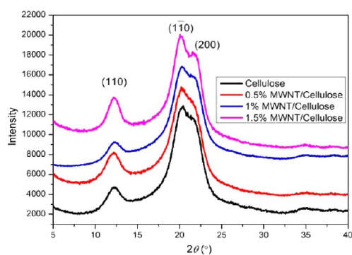
Figure 2. Typical XRD patterns of the regenerated cellulose and MWNT/cellulose nanofibers.
