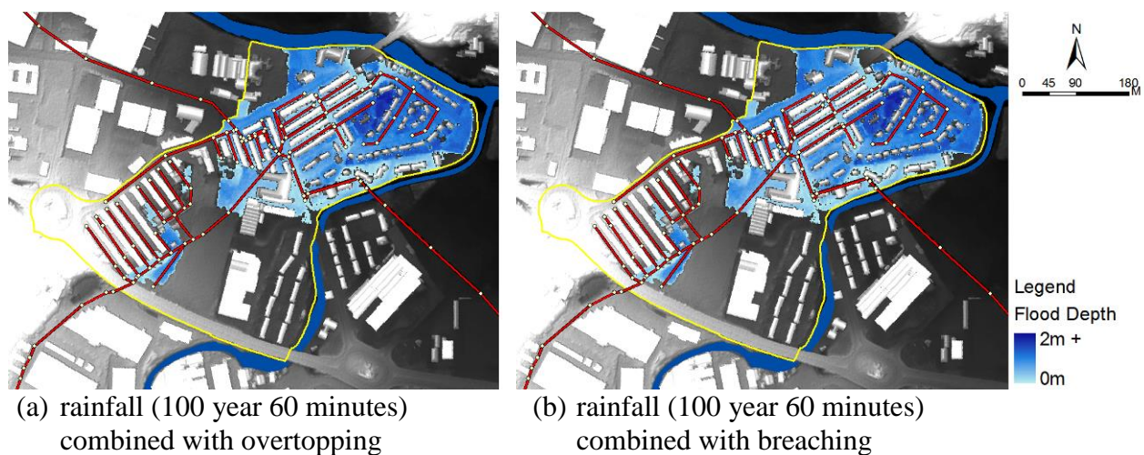
Figure 4. The maximum flood depth caused by composite pluvial and fluvial flooding scenarios
