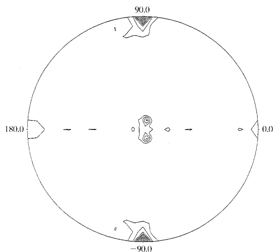
Figure 3 Self-rotation function calculated using monoclinic crystal data (section \kappa = 180^\circ , integration radius of 29 Å, calculated at 10–2.4 Å resolution).
